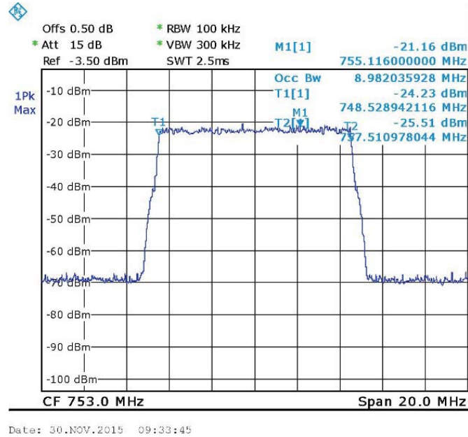
Figure 31. — 16QAM 753 MHz IN
