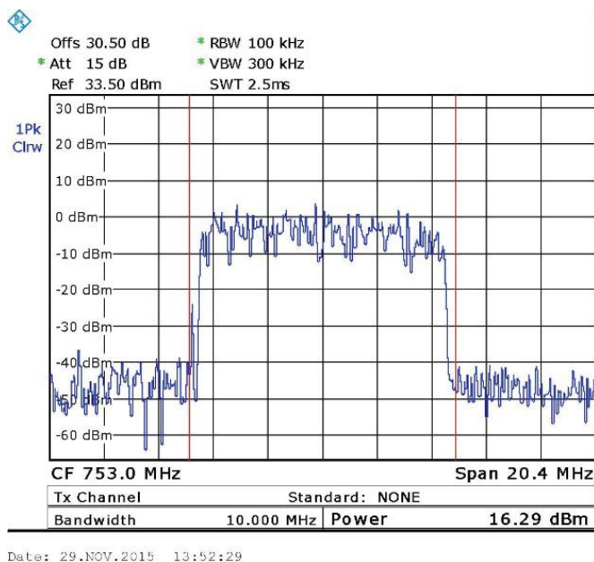
Figure 12. — 64QAM 753.0 MHz
