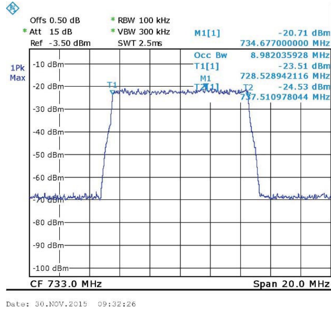
Figure 27. — 16QAM 733 MHz IN
