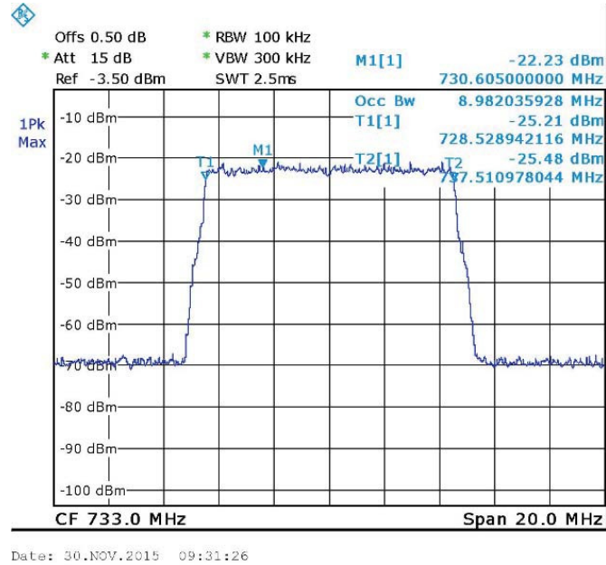
Figure 33. — QPSK 733 MHz IN
