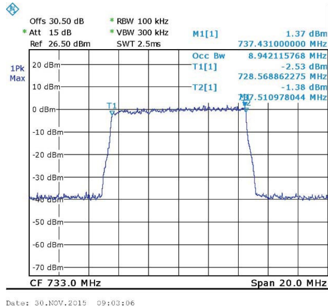
Figure 28. — 16QAM 733 MHz OUT
