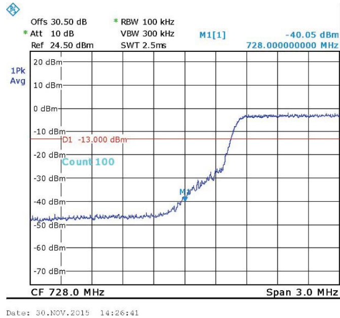
Figure 51. — 64QAM 733.0 MHz
