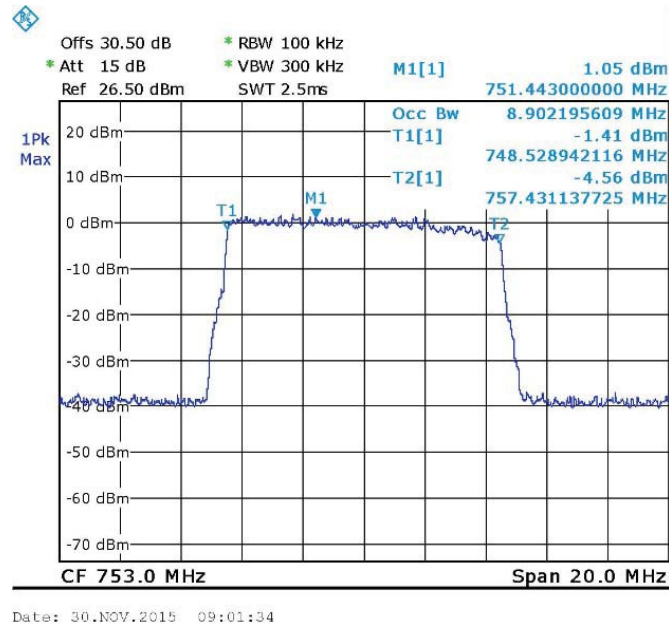
Figure 32. — 16QAM 753 MHz OUT
