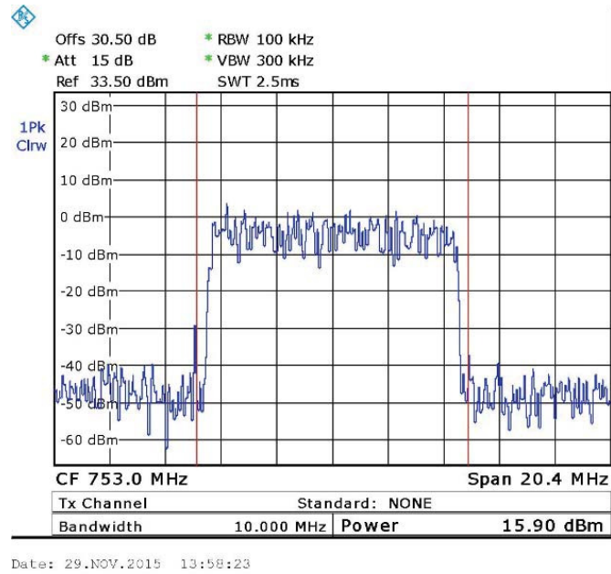
Figure 18. — QPSK 753.0 MHz
