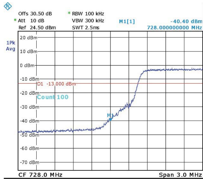
Figure 53. — 16QAM 733.0 MHz
