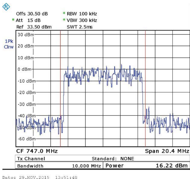
Figure 11. — 64QAM 747.0 MHz
