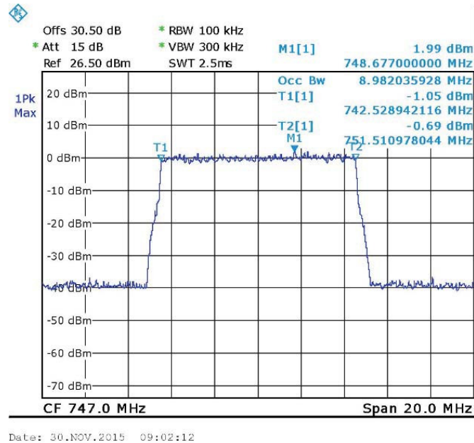
Figure 30. — 16QAM 747 MHz OUT
