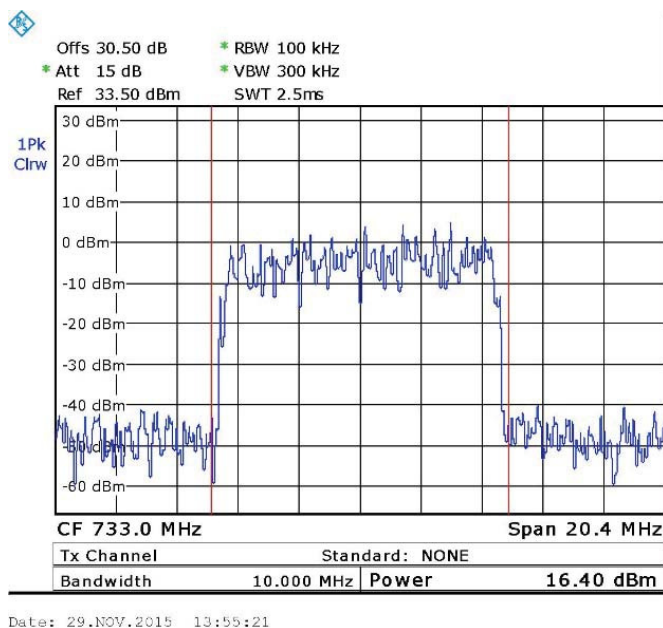
Figure 13. — 16QAM 733.0 MHz
