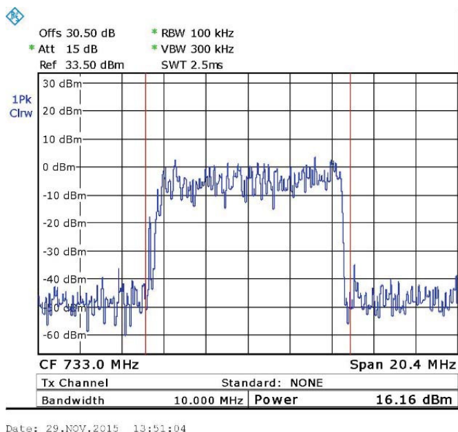
Figure 10. — 64QAM, 733.0 MHz
