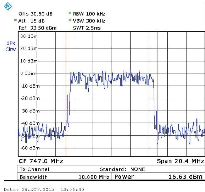
Figure 17. — QPSK 747.0 MHz
