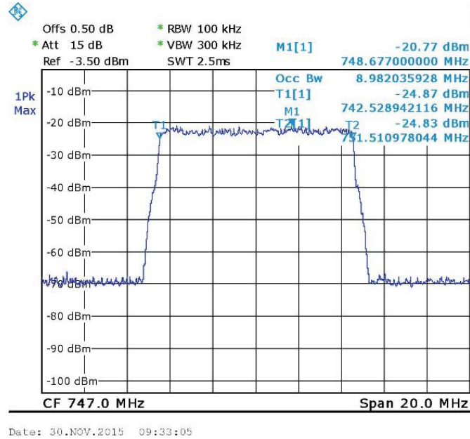
Figure 29. — 16QAM 747 MHz IN
