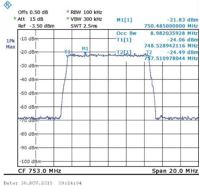
Figure 37. — QPSK 753 MHz IN
