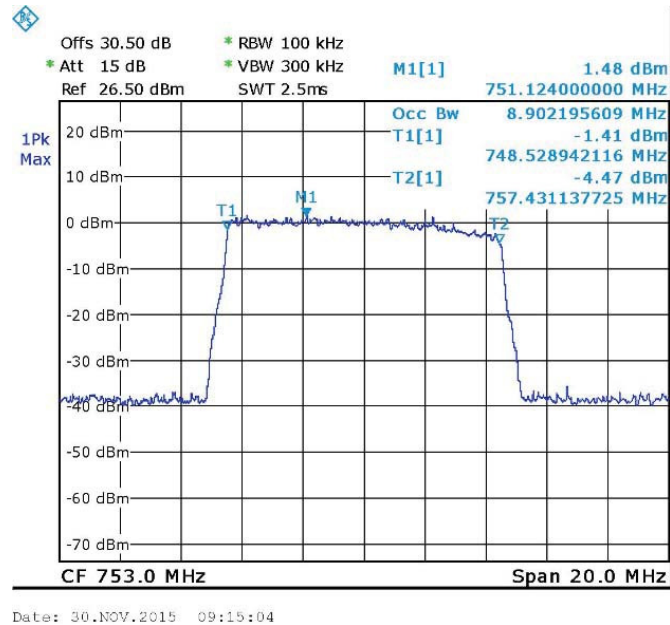
Figure 38. — QPSK 753 MHz OUT
