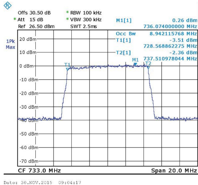
Figure 34. — QPSK 733 MHz OUT
