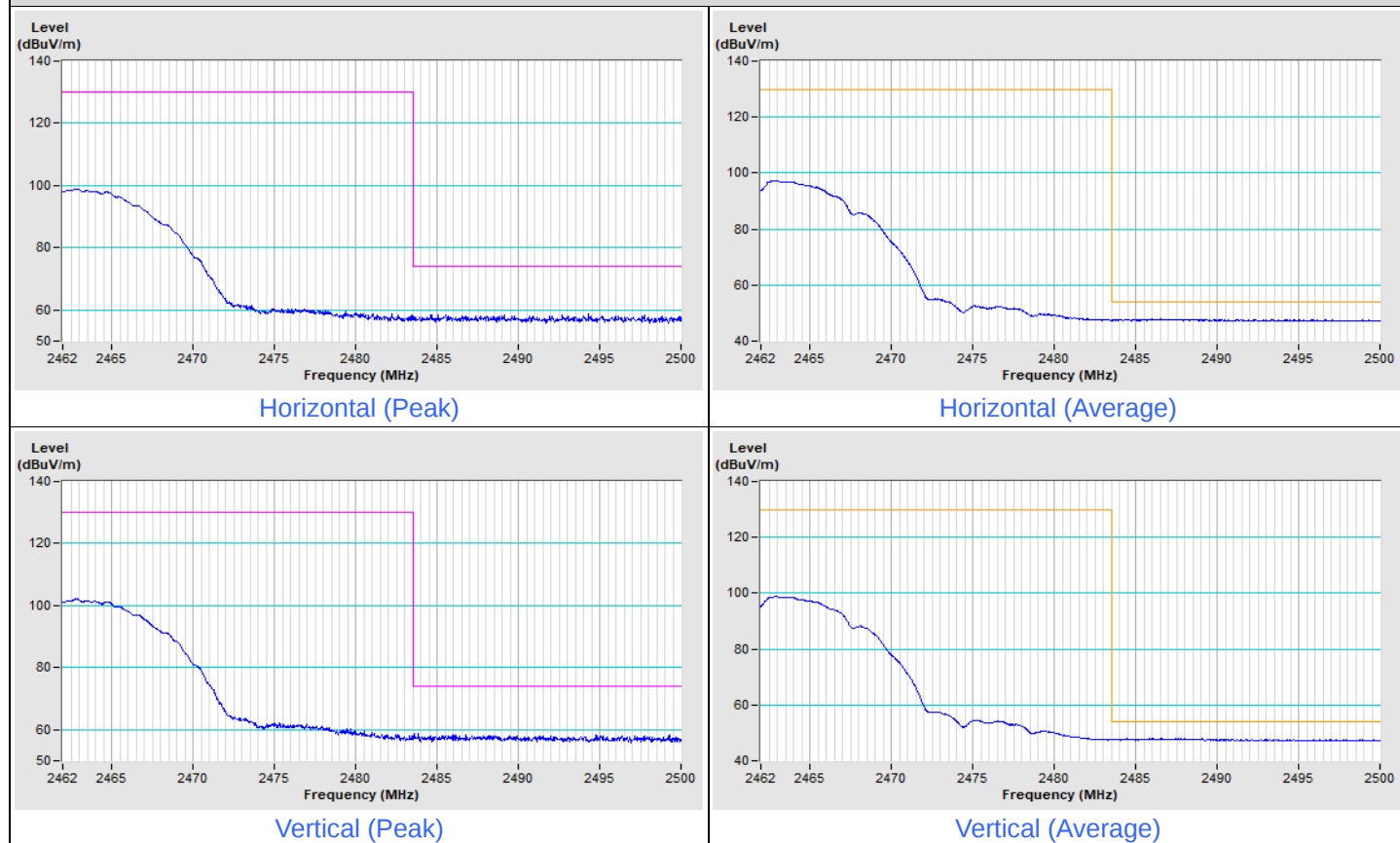
802.11b Channel 11
