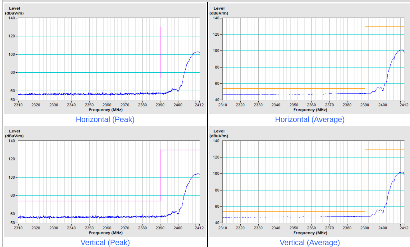
802.11b Channel 1
