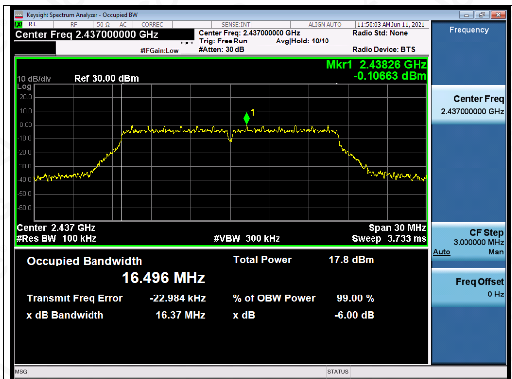
Test_Graph_802.11g_ANT1_2437_6Mbps_DTSBW
