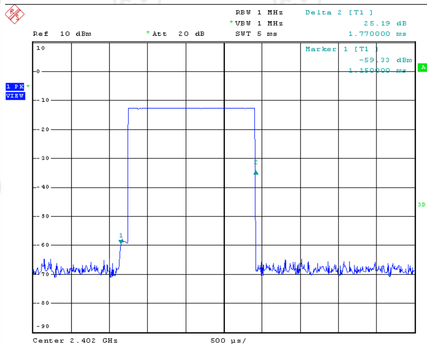
2402 MHz_DH3
