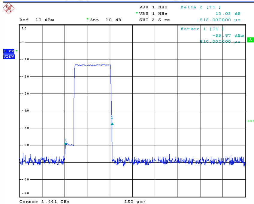
2441 MHz_DH1
