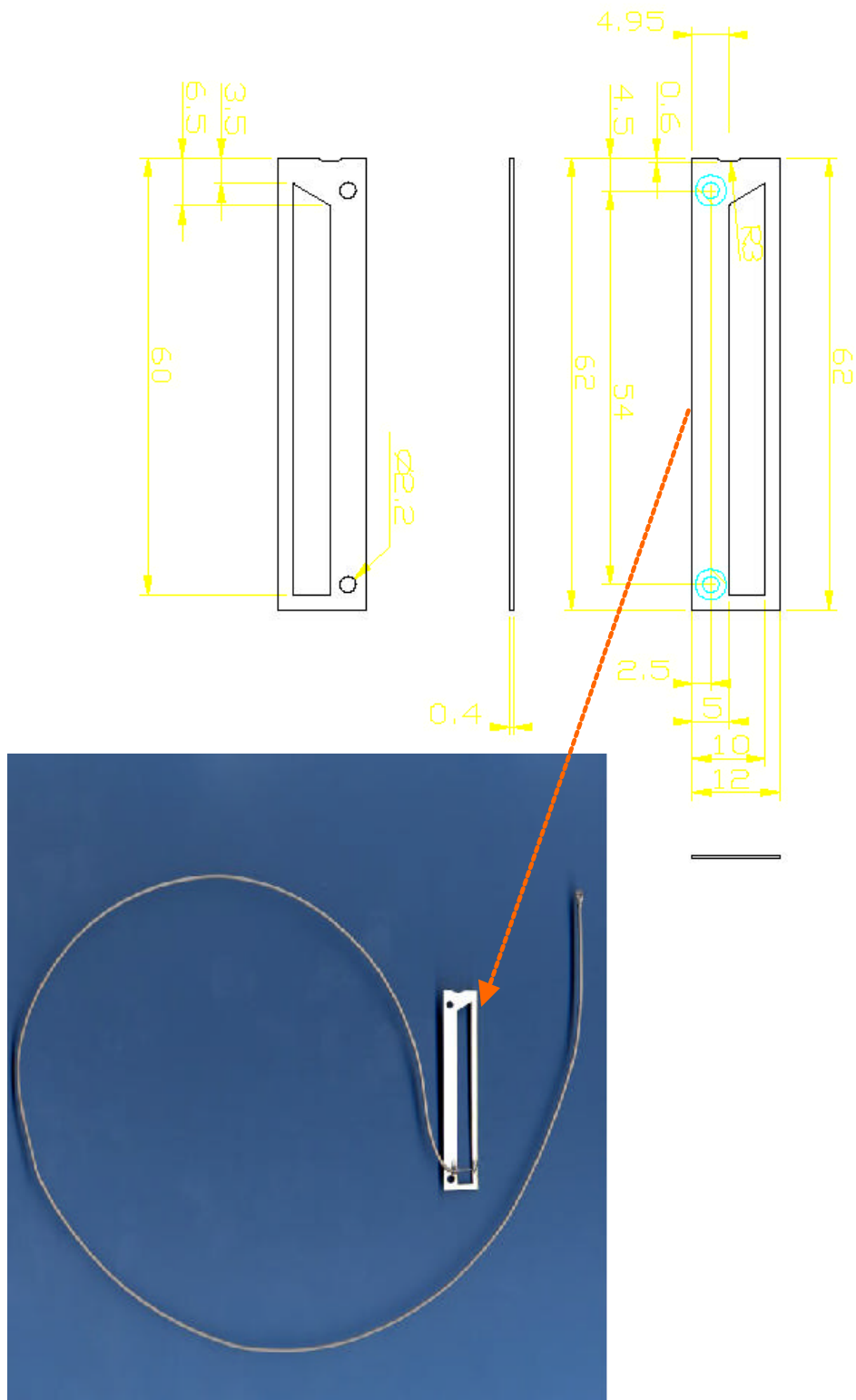
Photo.9: Exterior views of Antenna
