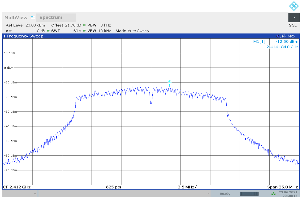
Fig.A.3.7 Power Spectral Density (802.11n-HT20, Ch 1)
