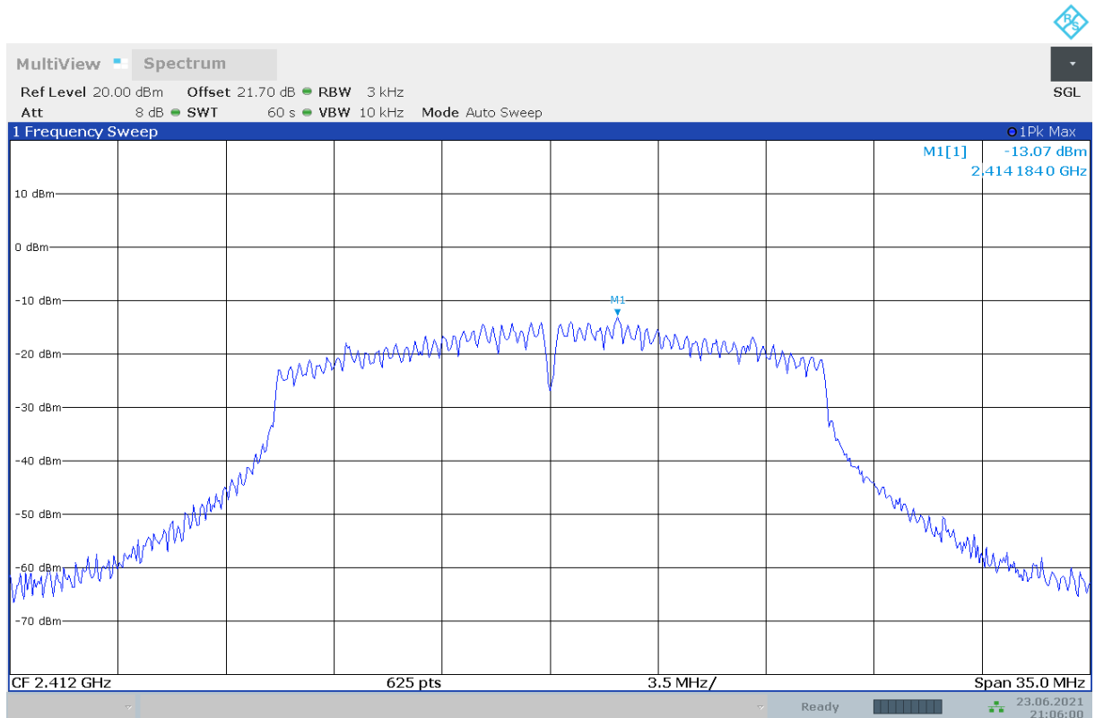
Fig.A.3.13 Power Spectral Density (802.11n-HT20, Ch 1)
