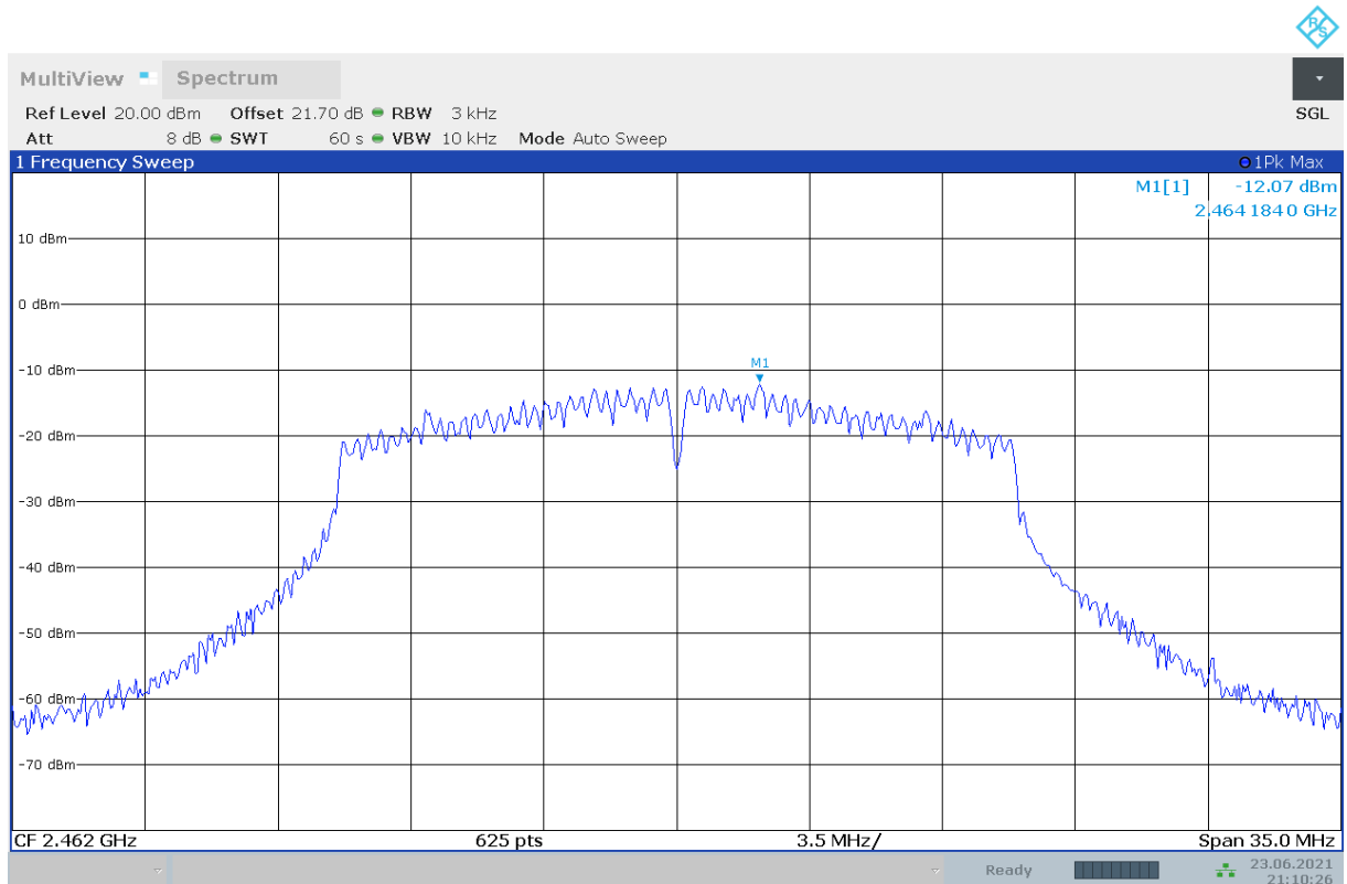
Fig.A.3.15 Power Spectral Density (802.11n-HT20, Ch 11)
