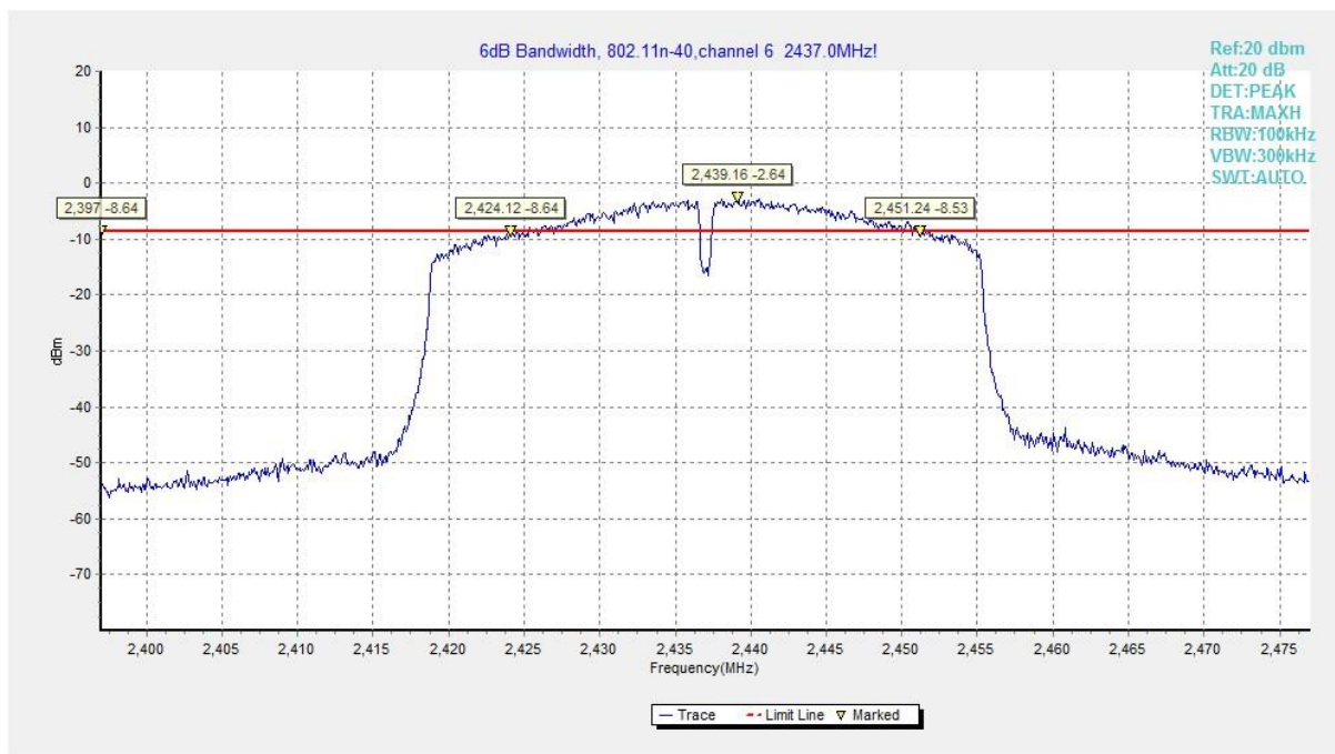
Fig.A.4.17 Occupied 6dB Bandwidth (802.11n-HT40, Ch 6)
