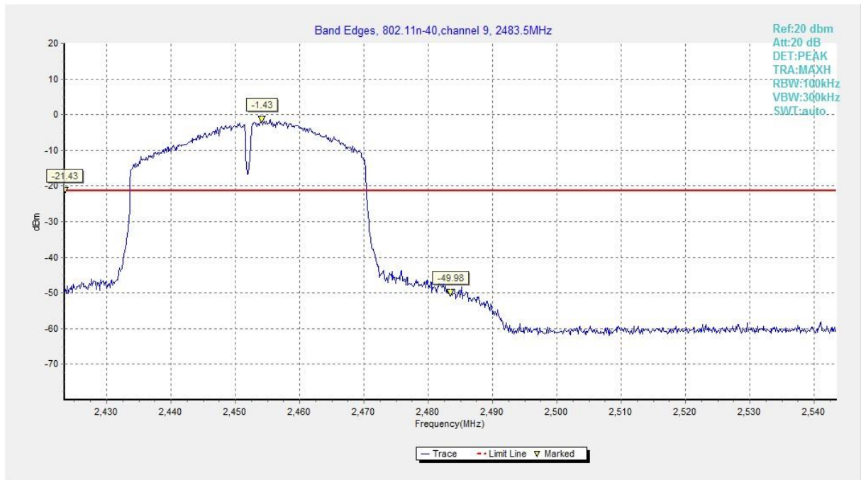
Fig.A.5.16 Band Edges (802.11n-HT40, Ch 9)
