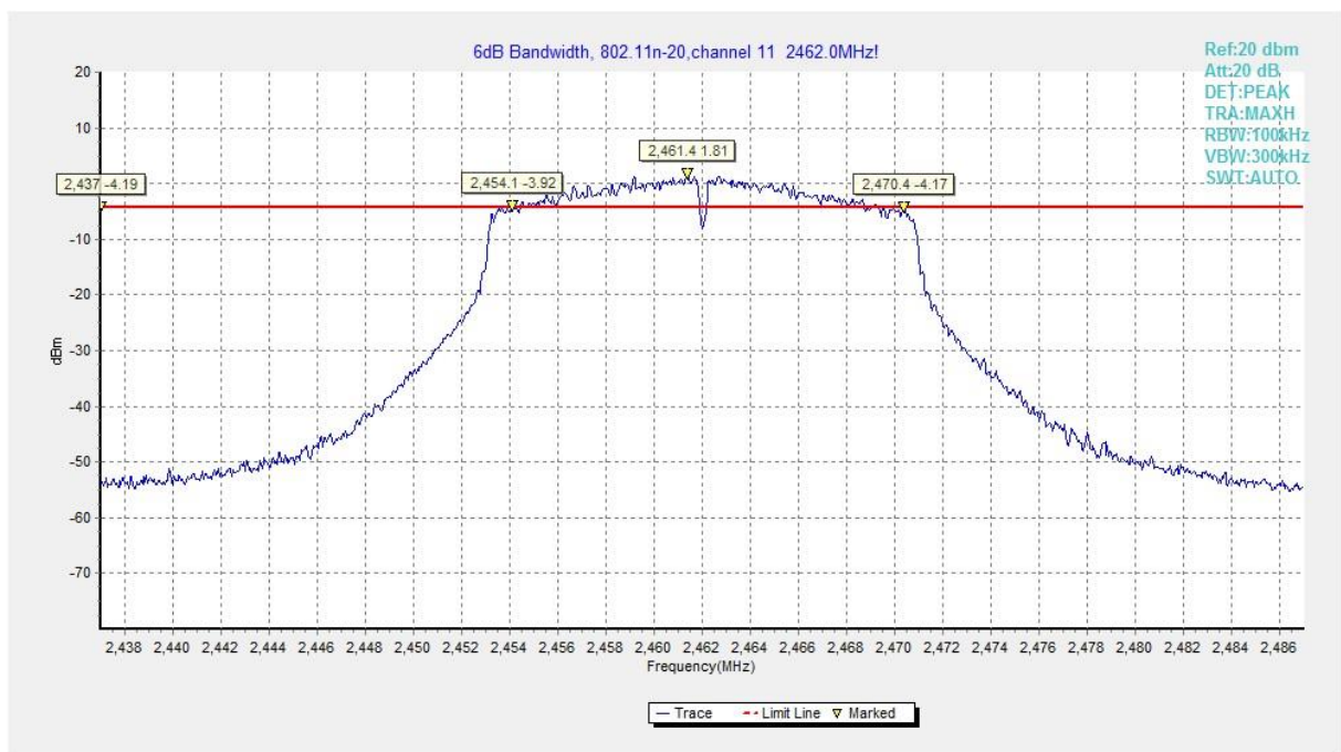
Fig.A.4.15 Occupied 6dB Bandwidth (802.11n-HT20, Ch 11)
