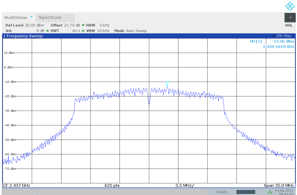
Fig.A.3.8 Power Spectral Density (802.11n-HT20, Ch 6)
