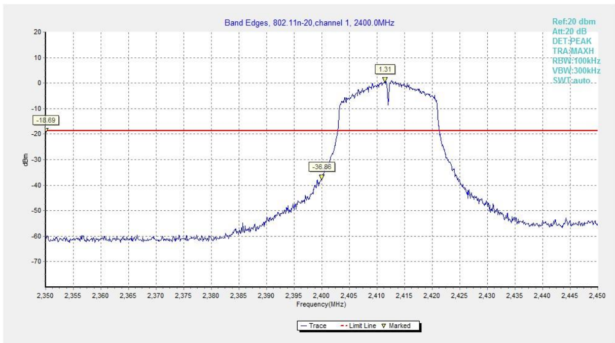
Fig.A.5.13 Band Edges (802.11n-HT20, Ch 1)
