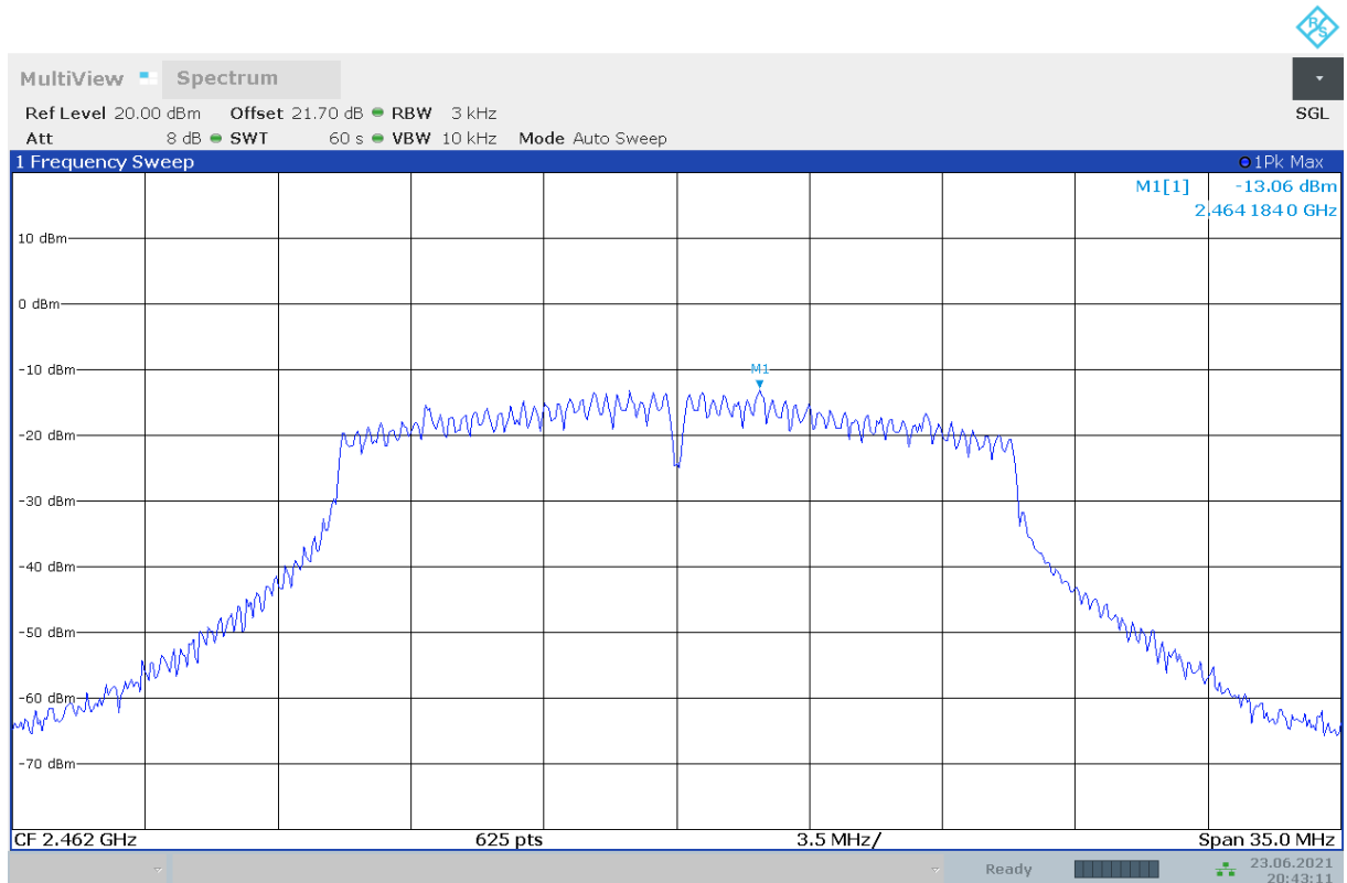
Fig.A.3.9 Power Spectral Density (802.11n-HT20, Ch 11)
