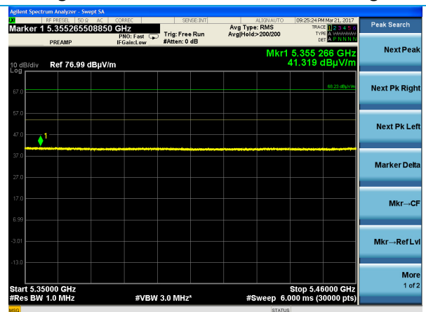
High Channel – 802.1ac HT-40 - Average
