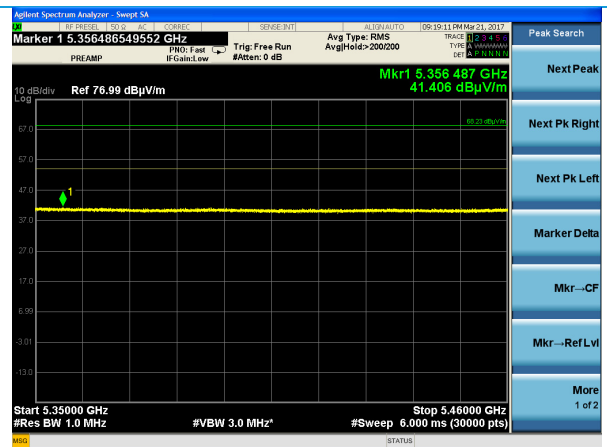
High Channel – 802.11a HT-20 – Average
