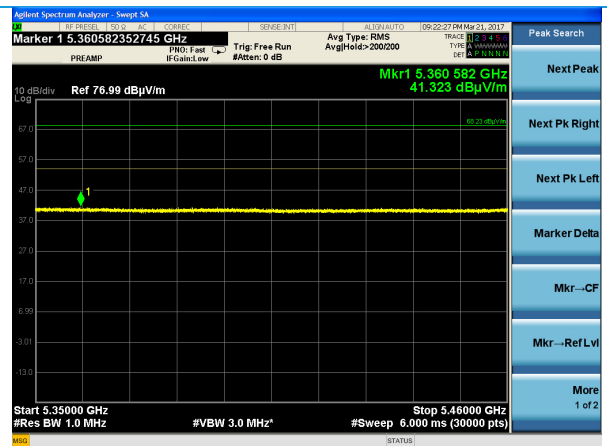
High Channel – 802.11ac HT-20 – Average
