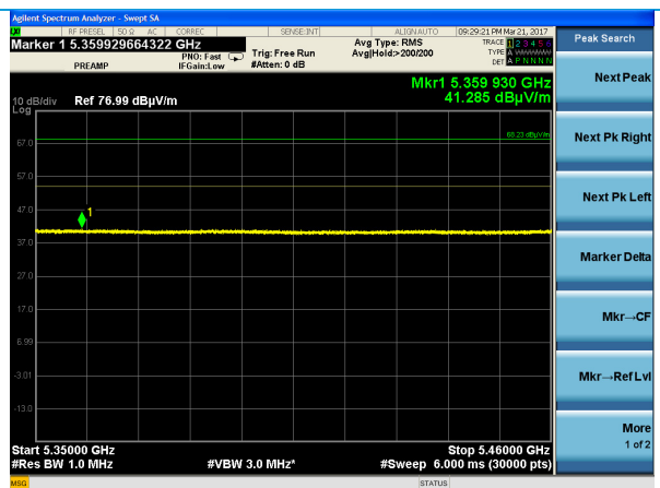
High Channel – 802.11ac HT-80 – Average
