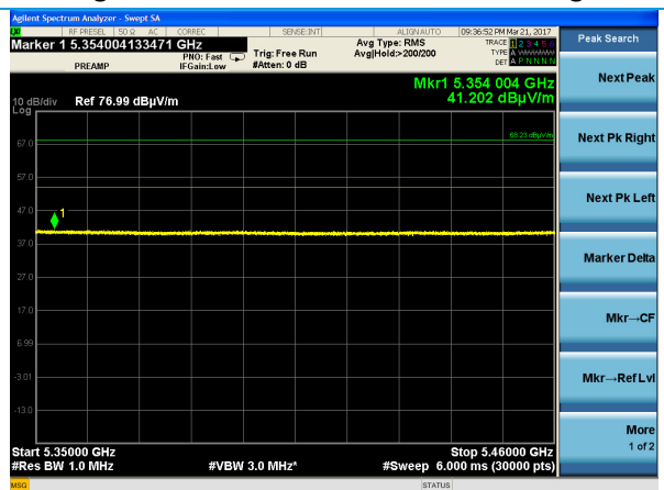
High Channel – 802.11n HT-40 - Average
