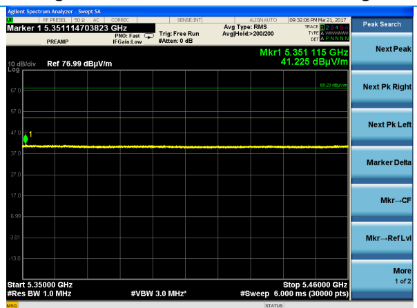
High Channel – 802.11n HT-20 – Average
