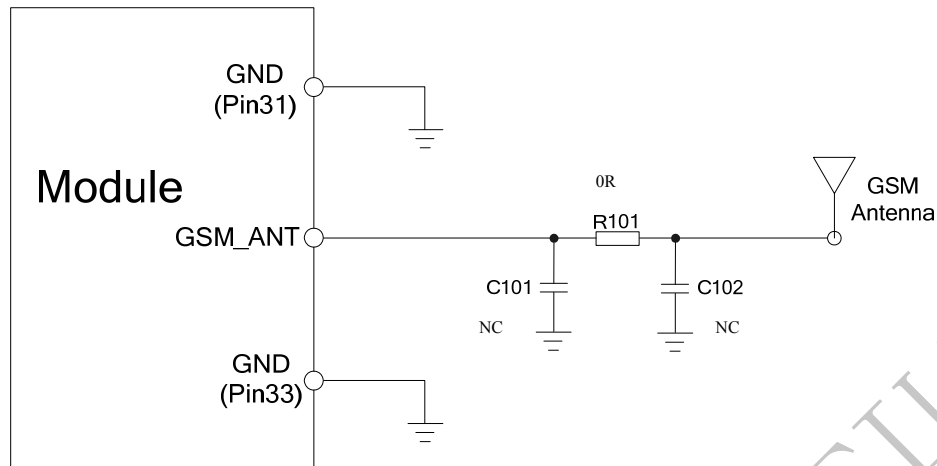
Figure5: GSM antenna matching circuit without RF connector
