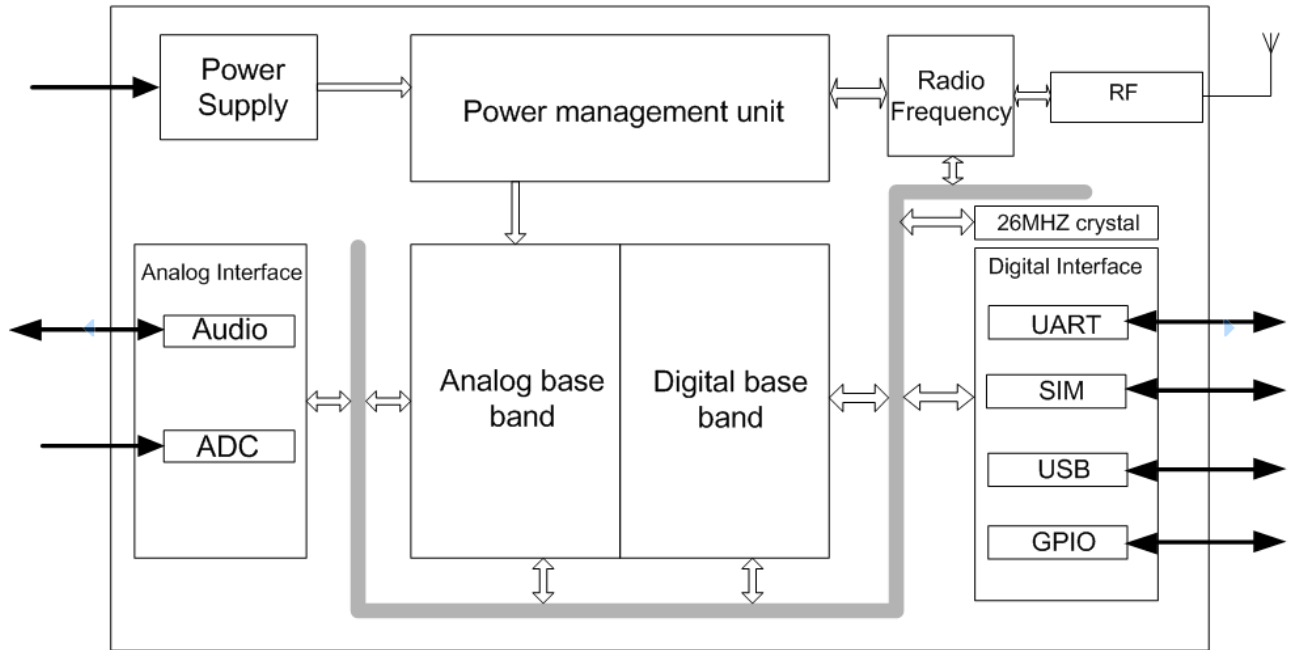
Figure 3: Block diagram of SIM800C
