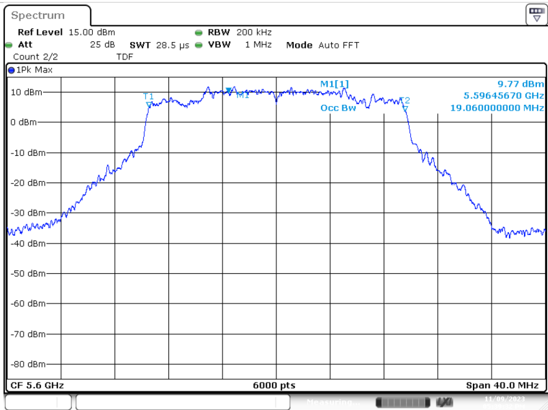
SISO A-802.11ax/be20-CH120-5600MHz-MCS0
