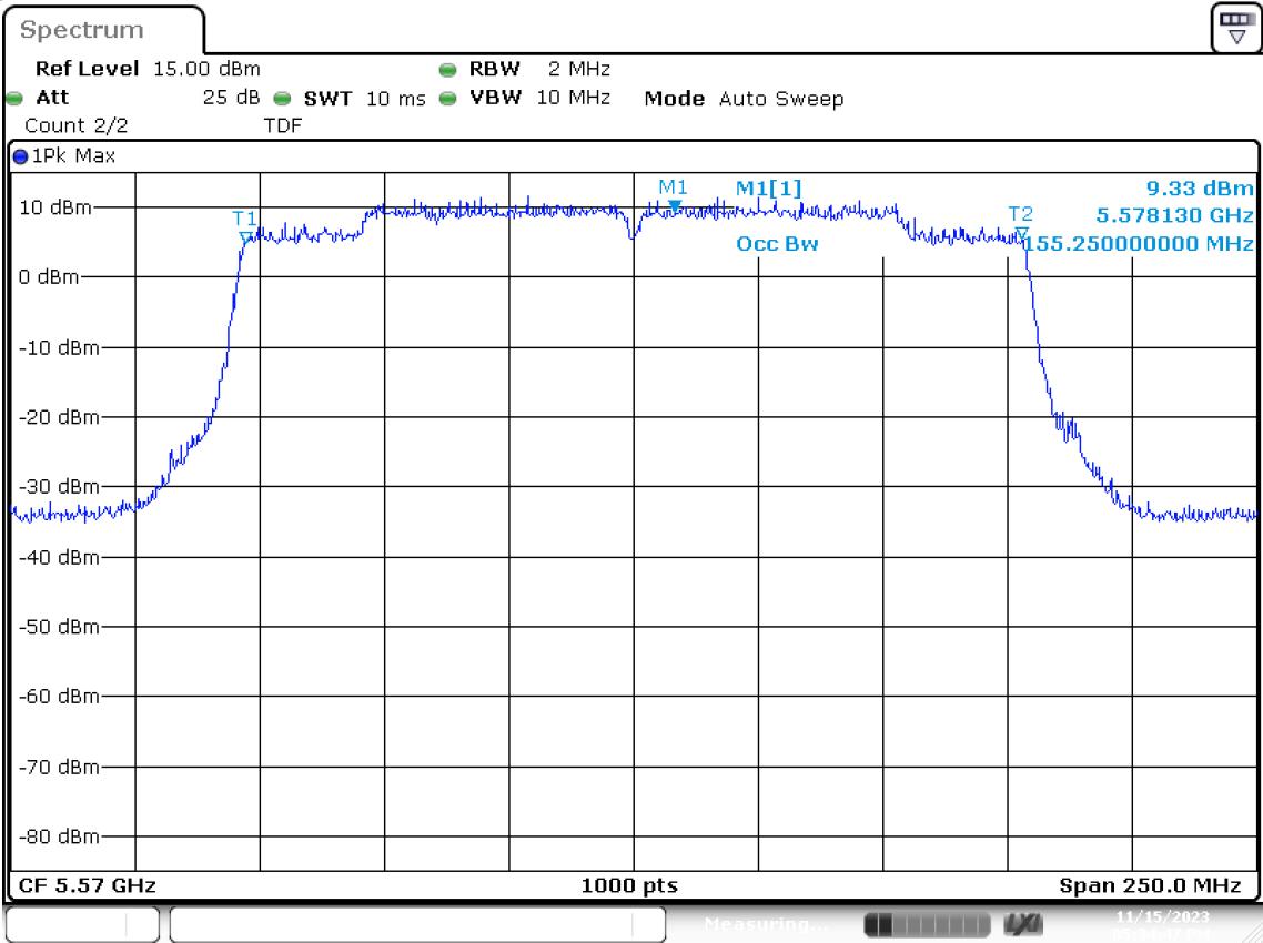
MIMO A-802.11ax/be160-CH114-5570MHz-MCS0
