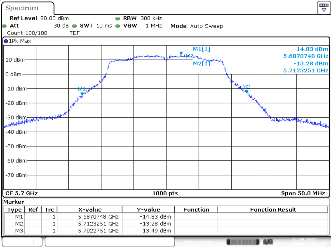
SISO A-802.11n20-CH140-5700MHz-HT0
