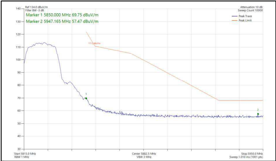
Figure 281 - 802.11a, SISO, Core 0 - 5825 MHz, Band Edge Frequency 5850 MHz
