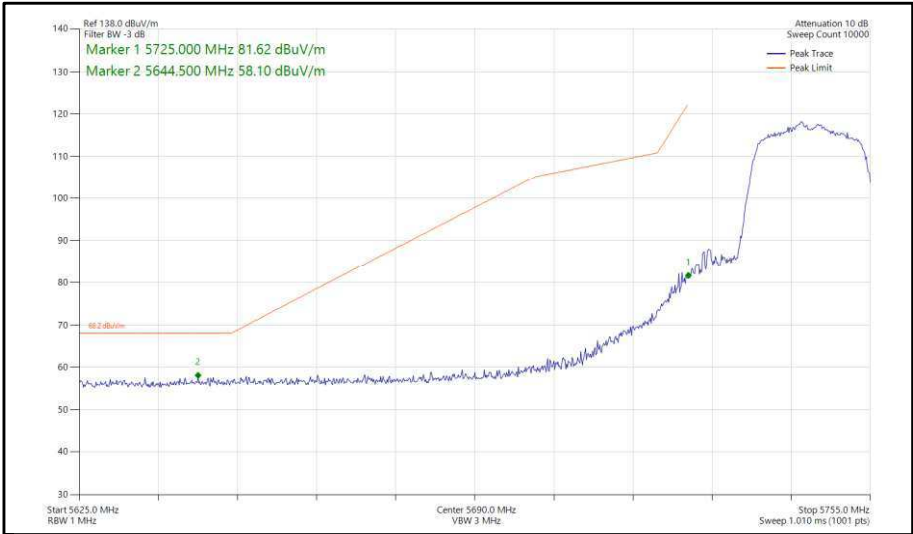
Figure 290 - 802.11n, HT20, SISO, Core 1 - 5745 MHz, Band Edge Frequency 5725 MHz
