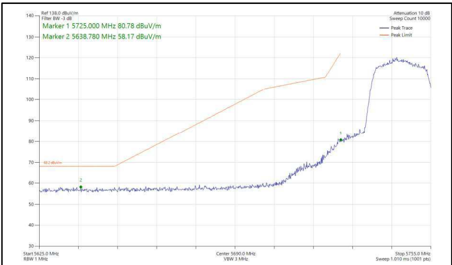
Figure 329 - 802.11ac, VHT20, TxBF, Core 0-1 - 5745 MHz, Band Edge Frequency 5725 MHz
