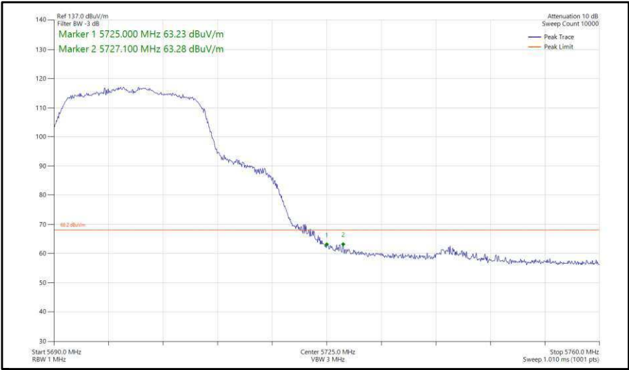
Figure 294 - 802.11n, HT20, SISO, Core 1 - 5700 MHz, Band Edge Frequency 5725 MHz
