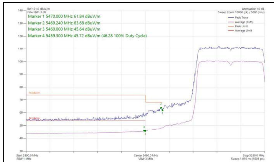
Figure 346 - 802.11ax, HE40, SU, SISO, Core 1 - 5510 MHz, Band Edge Frequency 5470 MHz
