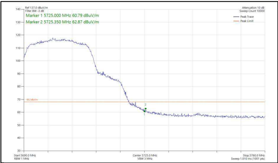
Figure 330 - 802.11ac, VHT20, TxBF, Core 0-1 - 5700 MHz, Band Edge Frequency 5725 MHz
