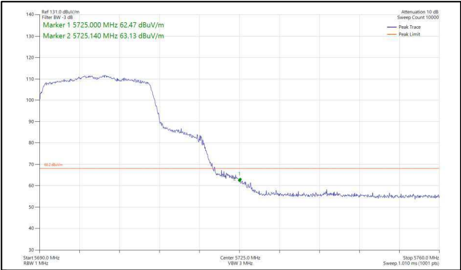
Figure 279 - 802.11ax, HE20, SU, SISO, Core 0 - 5700 MHz, Band Edge Frequency 5725 MHz
