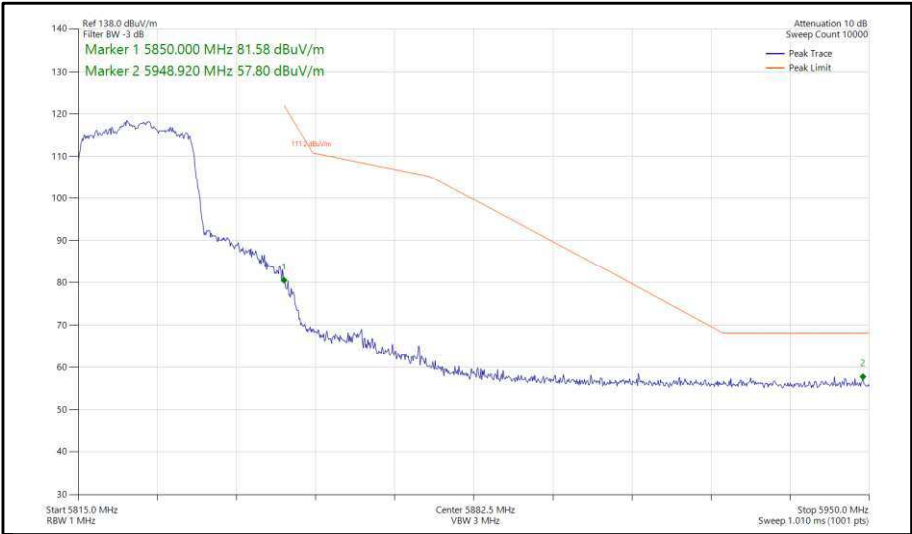
Figure 326 - 802.11ax, HE20, SU, SDM, Core 0-1 - 5825 MHz, Band Edge Frequency 5850 MHz
