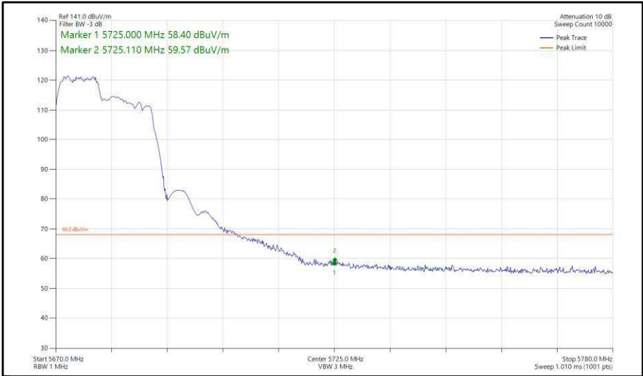
Figure 309 - 802.11ax, HE20, RU 106-53, CDD, Core 0-1 - 5680 MHz, Band Edge Frequency 5725 MHz
