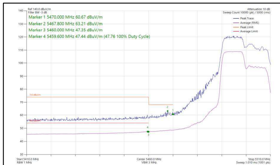
Figure 317 - 802.11ax, HE20, RU 106-53, SDM, Core 0-1 - 5500 MHz, Band Edge Frequency 5470 MHz
