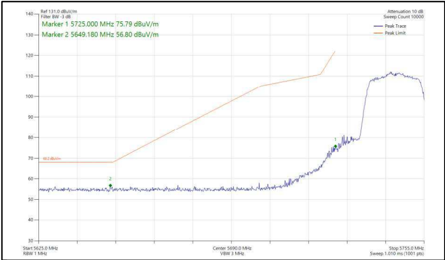
Figure 273 - 802.11n, HT20, SISO, Core 0 - 5745 MHz, Band Edge Frequency 5725 MHz
