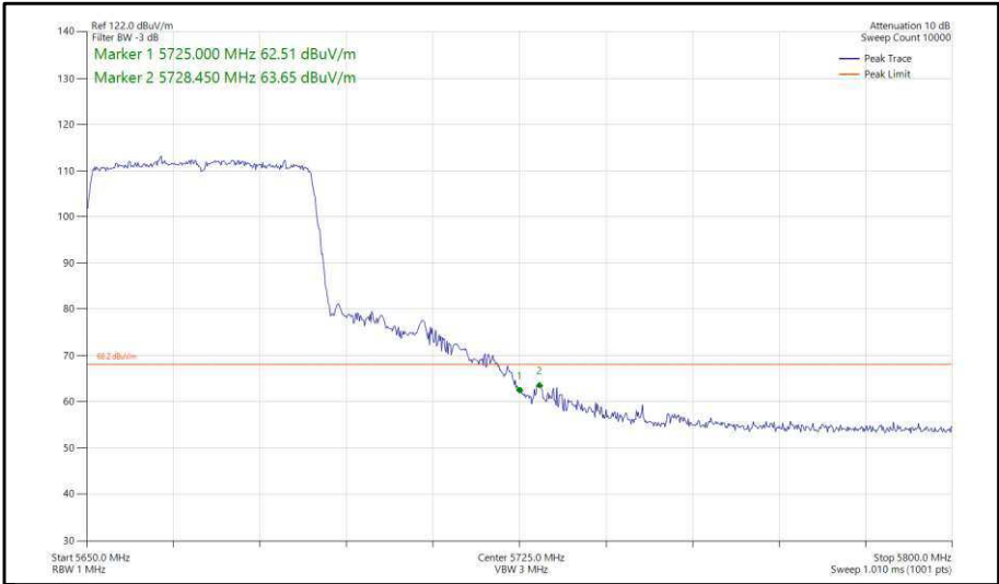
Figure 340 - 802.11ax, HE40, SU, SISO, Core 0 - 5670 MHz, Band Edge Frequency 5725 MHz
