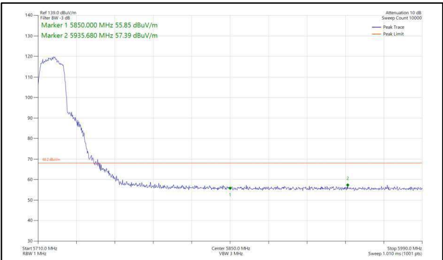
Figure 331 - 802.11ac, VHT20, TxBF, Core 0-1 - 5720 MHz, Band Edge Frequency 5850 MHz
