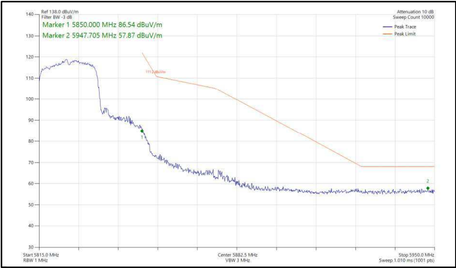
Figure 313 - 802.11ax, HE20, SU, CDD, Core 0-1 - 5825 MHz, Band Edge Frequency 5850 MHz
