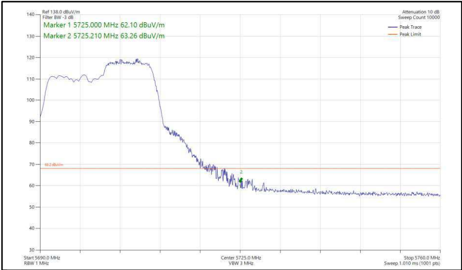
Figure 324 - 802.11ax, HE20, RU 106-54, SDM, Core 0-1 - 5700 MHz, Band Edge Frequency 5725 MHz
