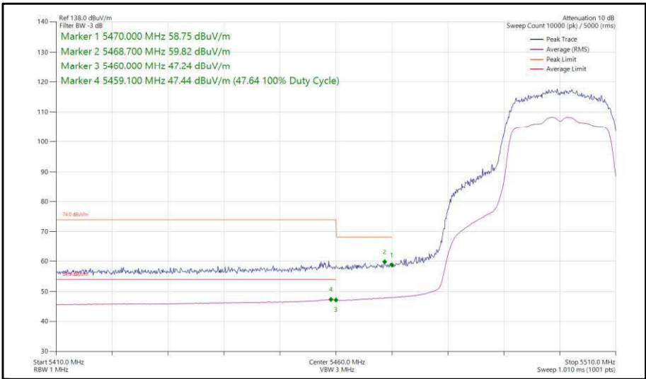
Figure 328 - 802.11ac, VHT20, TxBF, Core 0-1 - 5500 MHz, Band Edge Frequency 5470 MHz
