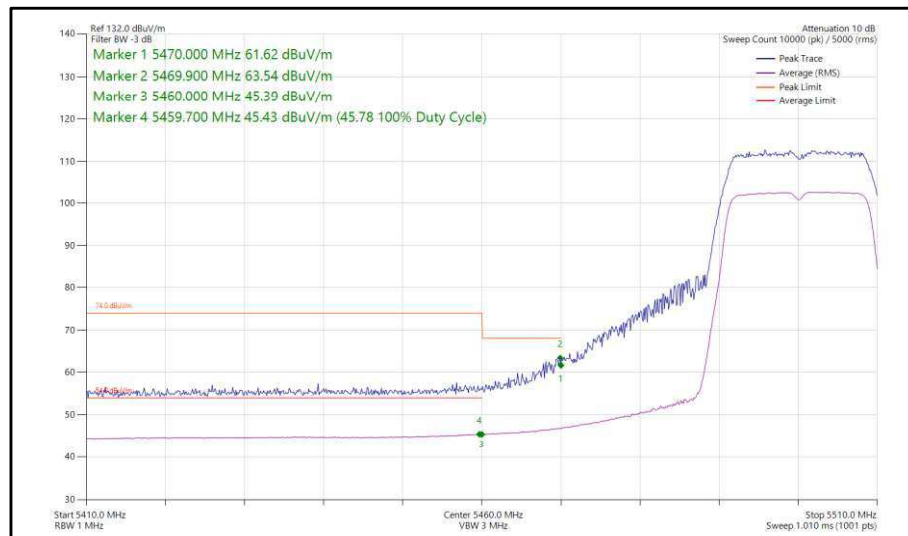
Figure 269 - 802.11n, HT20, SISO, Core 0 - 5500 MHz, Band Edge Frequency 5470 MHz
