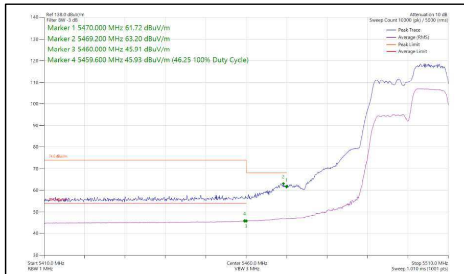
Figure 271 - 802.11ax, HE20, RU 106-54, SISO, Core 0 - 5500 MHz, Band Edge Frequency 5470 MHz
