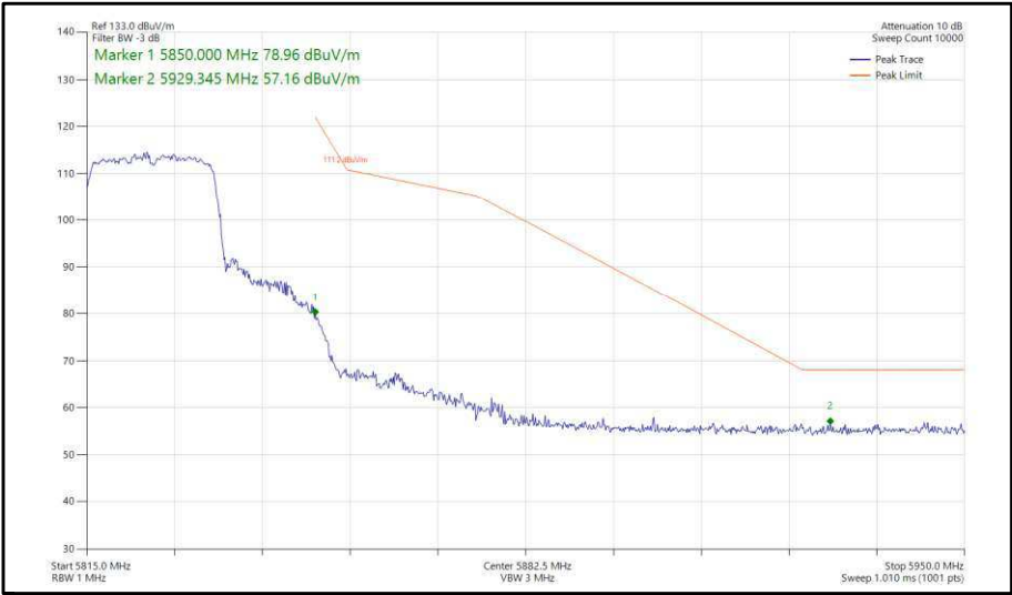
Figure 283 - 802.11ax, HE20, SU, SISO, Core 0 - 5825 MHz, Band Edge Frequency 5850 MHz
