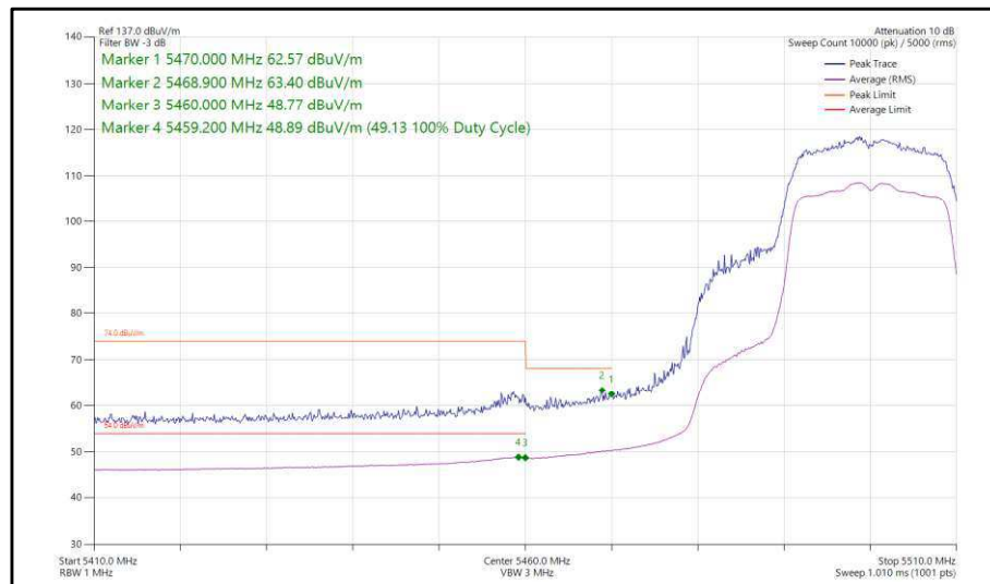
Figure 286 - 802.11n, HT20, SISO, Core 1 - 5500 MHz, Band Edge Frequency 5470 MHz
