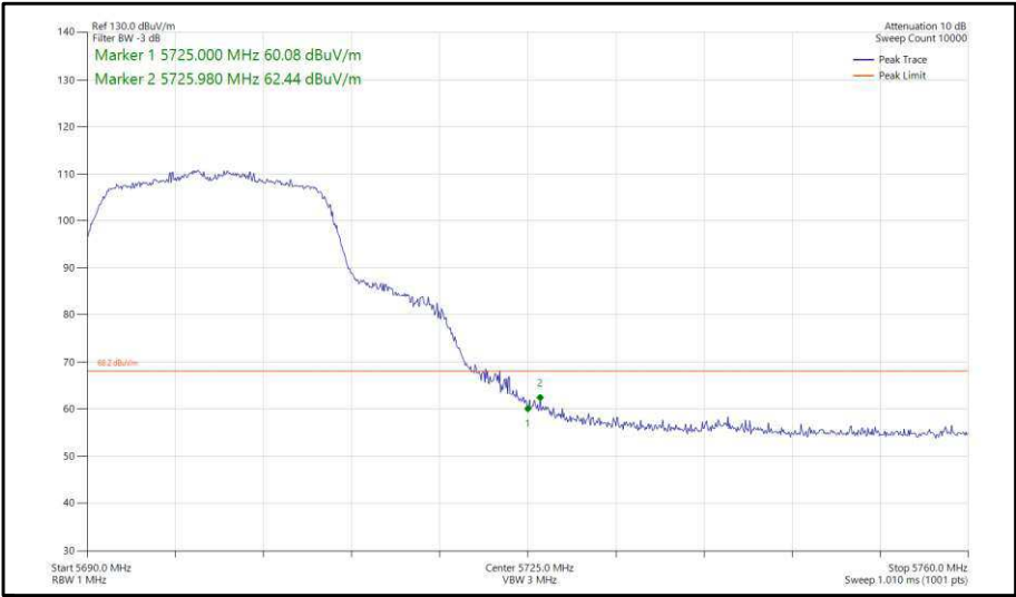
Figure 277 - 802.11n, HT20, SISO, Core 0 - 5700 MHz, Band Edge Frequency 5725 MHz
