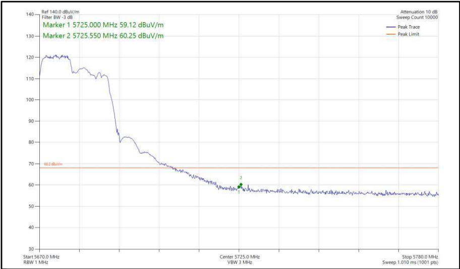
Figure 322 - 802.11ax, HE20, RU 106-53, SDM, Core 0-1 - 5680 MHz, Band Edge Frequency 5725 MHz
