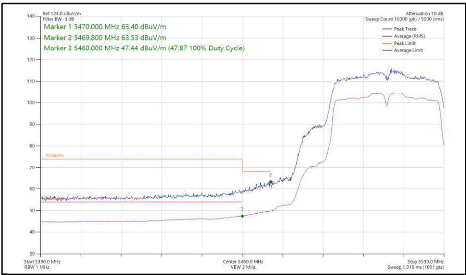
Figure 345 - 802.11n, HT40, SISO, Core 1 - 5510 MHz, Band Edge Frequency 5470 MHz
