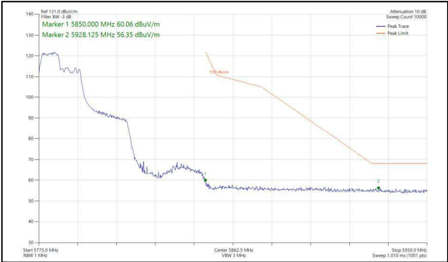
Figure 344 - 802.11ax, HE40, RU 106-53, SISO, Core 0 - 5795 MHz, Band Edge Frequency 5850 MHz
