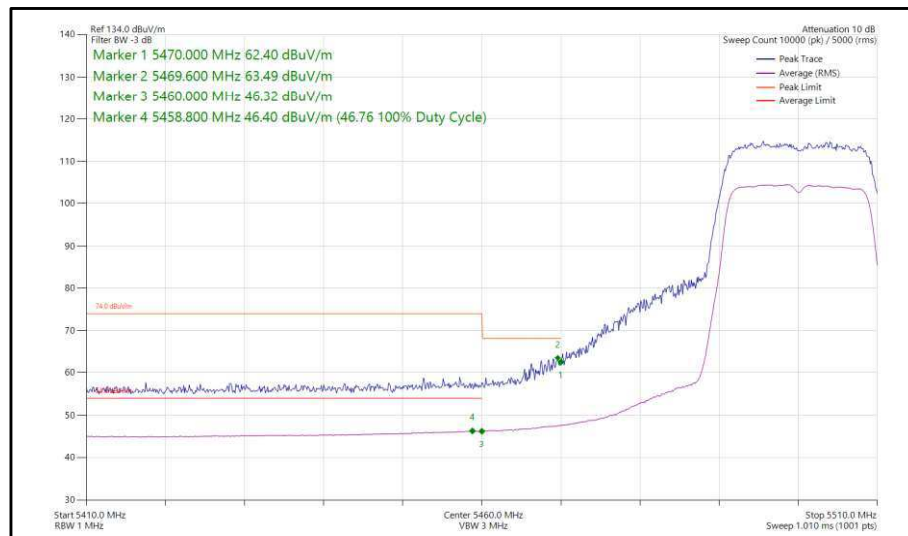
Figure 302 - 802.11n, HT20, CDD, Core 0-1 - 5500 MHz, Band Edge Frequency 5470 MHz
