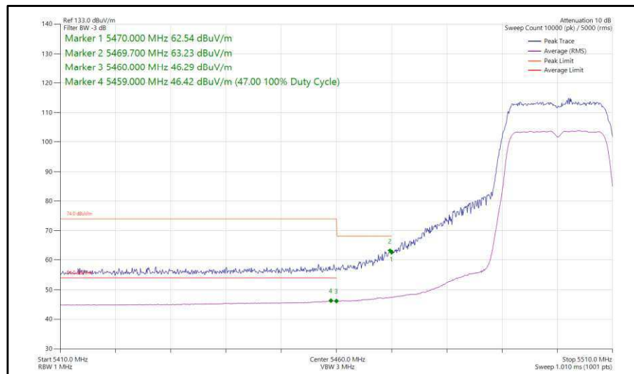
Figure 315 - 802.11n, HT20, SDM, Core 0-1 - 5500 MHz, Band Edge Frequency 5470 MHz
