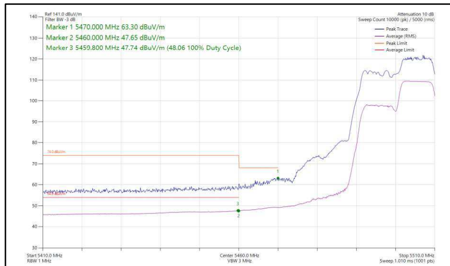
Figure 288 - 802.11ax, HE20, RU 106-54, SISO, Core 1 - 5500 MHz, Band Edge Frequency 5470 MHz
