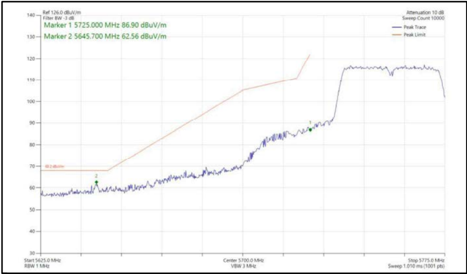
Figure 336 - 802.11n, HT40, SISO, Core 0 - 5755 MHz, Band Edge Frequency 5725 MHz
