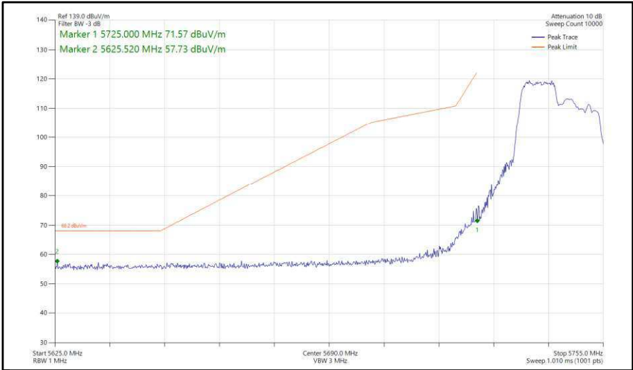
Figure 307 - 802.11ax, HE20, RU 106-53, CDD, Core 0-1 - 5745 MHz, Band Edge Frequency 5725 MHz
