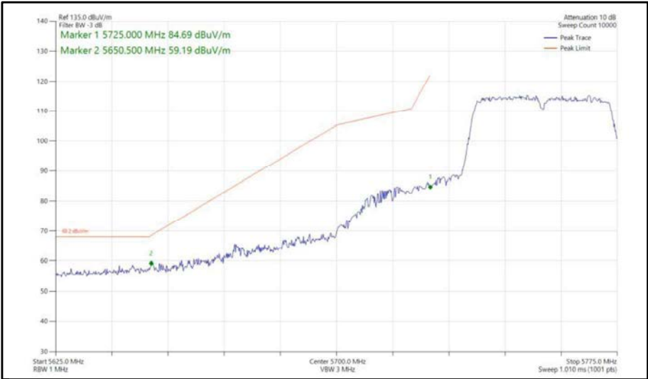
Figure 348 - 802.11n, HT40, SISO, Core 1 - 5755 MHz, Band Edge Frequency 5725 MHz
