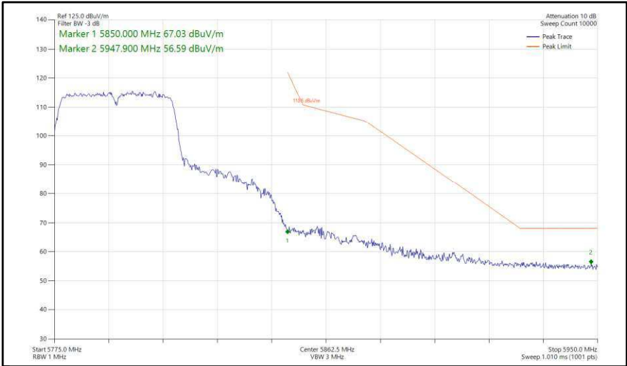
Figure 342 - 802.11n, HT40, SISO, Core 0 - 5795 MHz, Band Edge Frequency 5850 MHz
