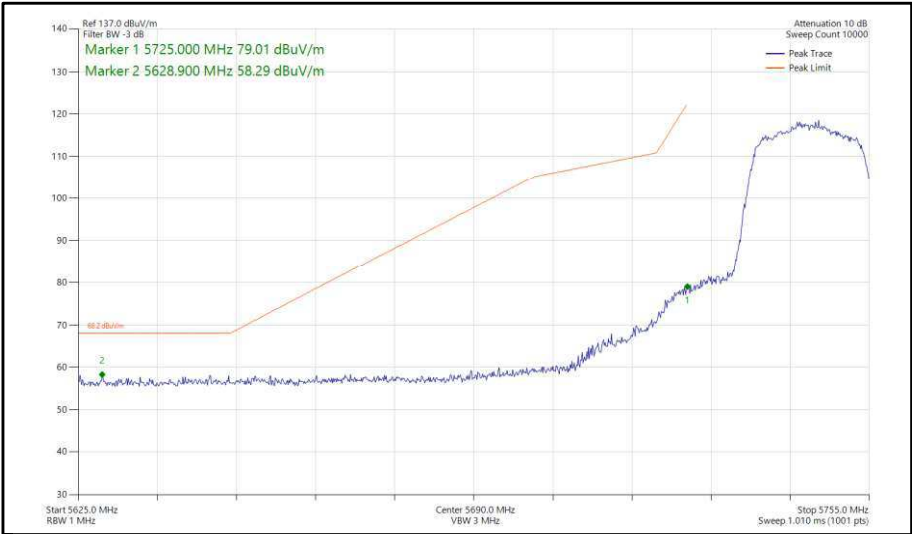
Figure 318 - 802.11n, HT20, SDM, Core 0-1 - 5745 MHz, Band Edge Frequency 5725 MHz
