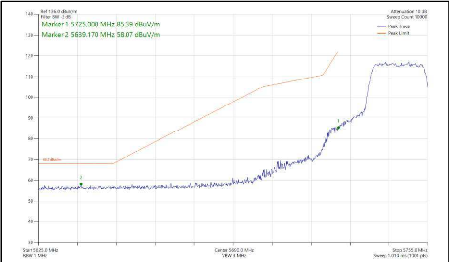
Figure 305 - 802.11n, HT20, CDD, Core 0-1 - 5745 MHz, Band Edge Frequency 5725 MHz
