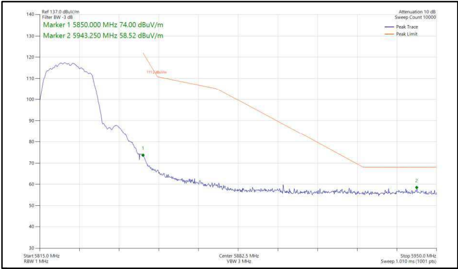
Figure 298 - 802.11a, SISO, Core 1 - 5825 MHz, Band Edge Frequency 5850 MHz
