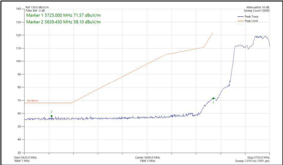
Figure 320 - 802.11ax, HE20, RU 106-54, SDM, Core 0-1 - 5745 MHz, Band Edge Frequency 5725 MHz
