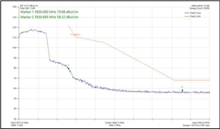
Figure 300 - 802.11ax, HE20, SU, SISO, Core 1 - 5825 MHz, Band Edge Frequency 5850 MHz
