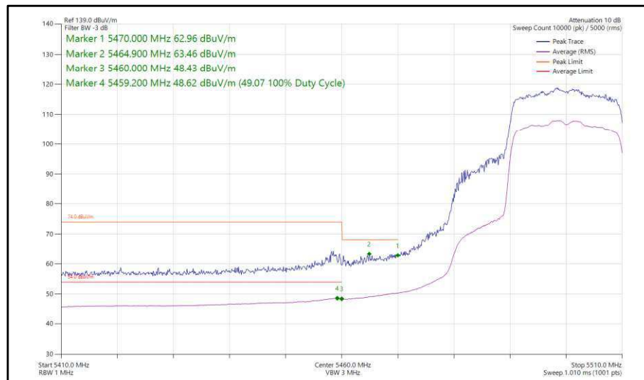
Figure 316 - 802.11ax, HE20, SU, SDM, Core 0-1 - 5500 MHz, Band Edge Frequency 5470 MHz
