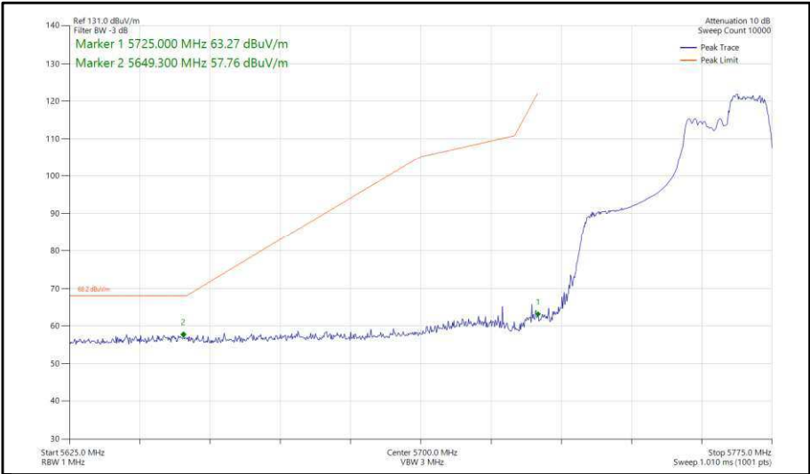
Figure 338 - 802.11ax, HE40, RU 106-56, SISO, Core 0 - 5755 MHz, Band Edge Frequency 5725 MHz
