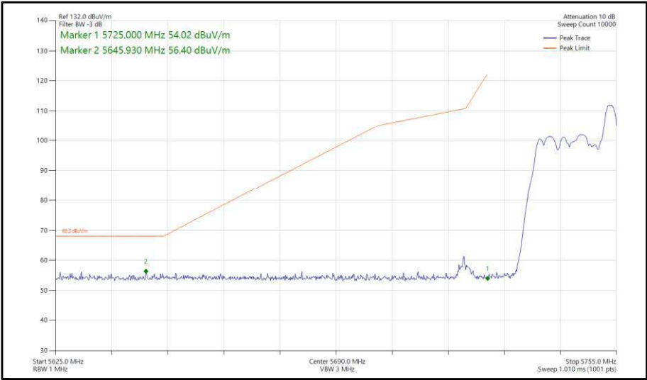
Figure 275 - 802.11ax, HE20, RU 26-8, SISO, Core 0 - 5745 MHz, Band Edge Frequency 5725 MHz
