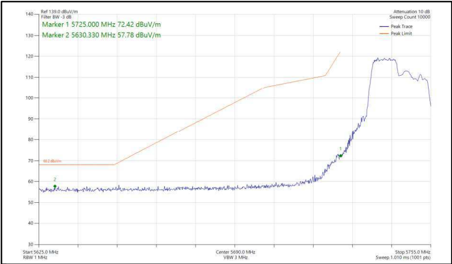
Figure 292 - 802.11ax, HE20, RU 106-53, SISO, Core 1 - 5745 MHz, Band Edge Frequency 5725 MHz
