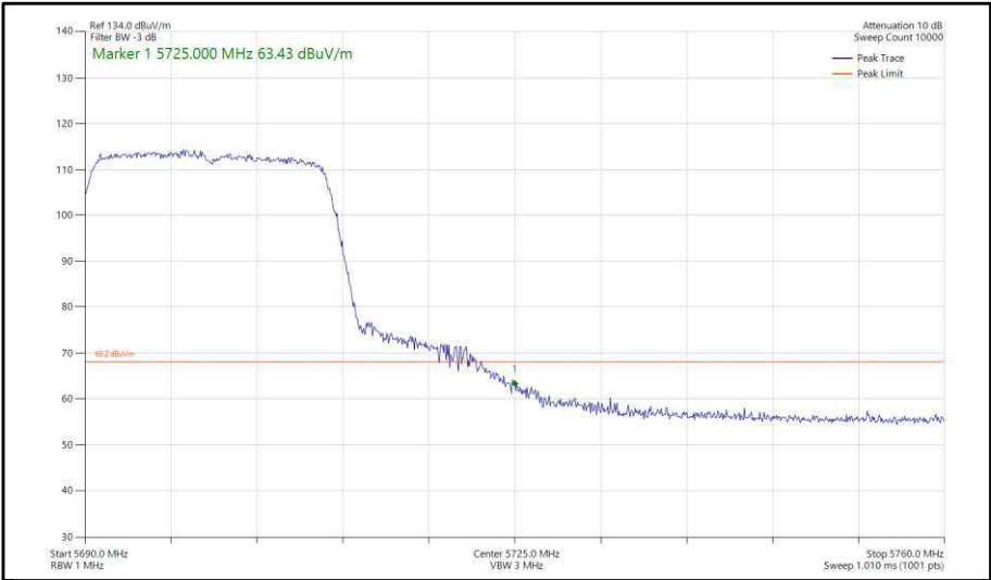
Figure 296 - 802.11ax, HE20, SU, SISO, Core 1 - 5700 MHz, Band Edge Frequency 5725 MHz
