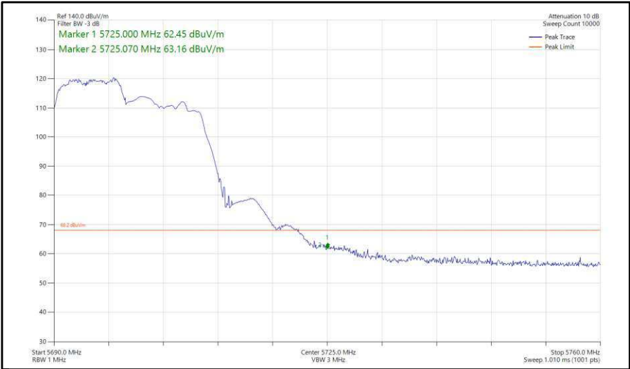
Figure 311 - 802.11ax, HE20, RU 106-53, CDD, Core 0-1 - 5700 MHz, Band Edge Frequency 5725 MHz
