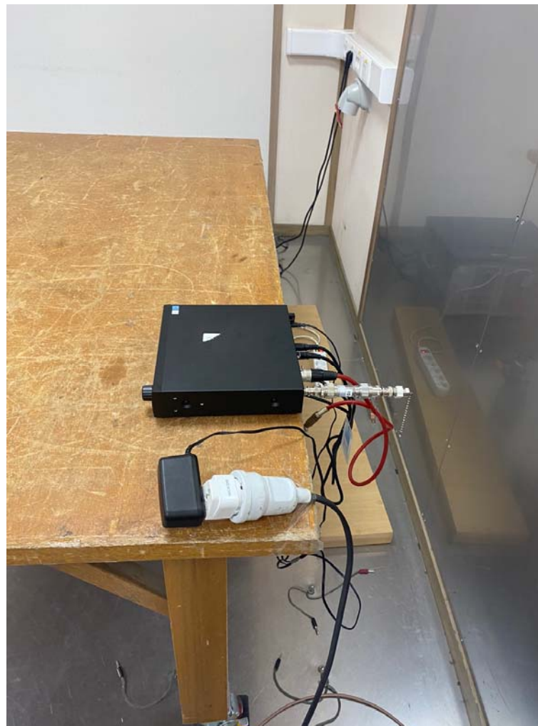
AC Conducted measurement (Rear view)
