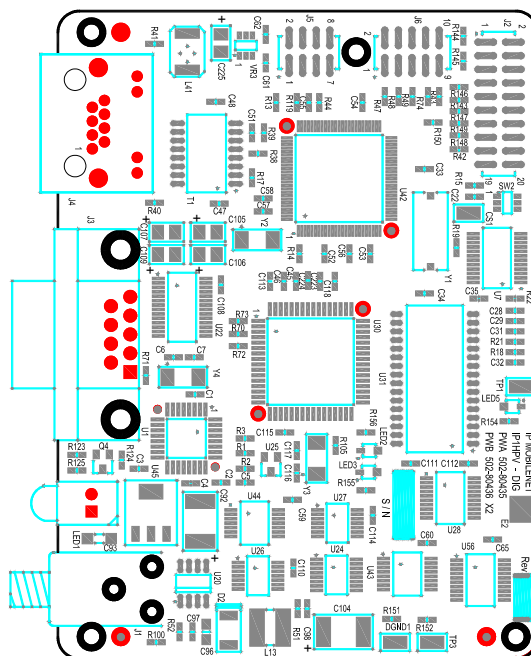
M1617-12 Mobile Radio Digital Circuit Board
