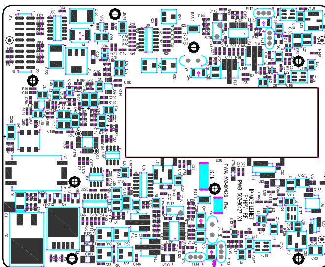
M1617-12 Mobile Radio RF Circuit Board
