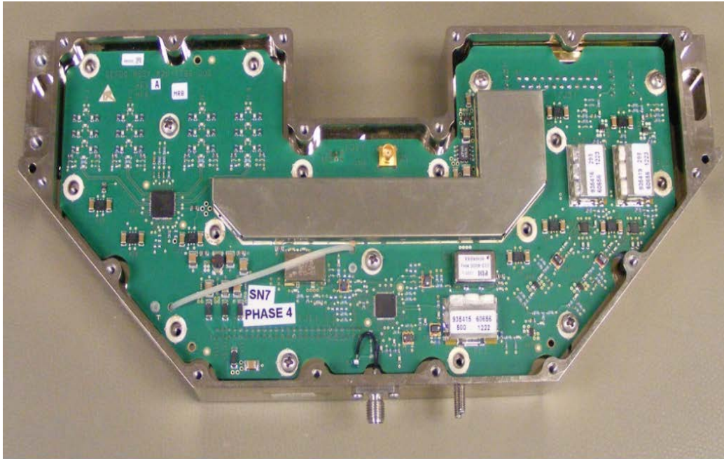
Figure I-3 – Digital Receiver/ Frequency Source Chassis 2
