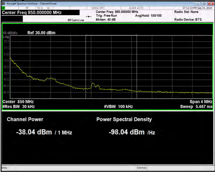
Band26(824-849) QPSK BW=1.4MHz Channel=27033 RB Size=1 Position=#0 Normal
