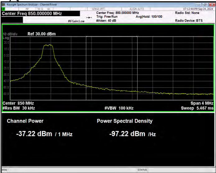
Band26(824-849) QPSK BW=1.4MHz Channel=27033 RB Size=1 Position=#Max Extended
