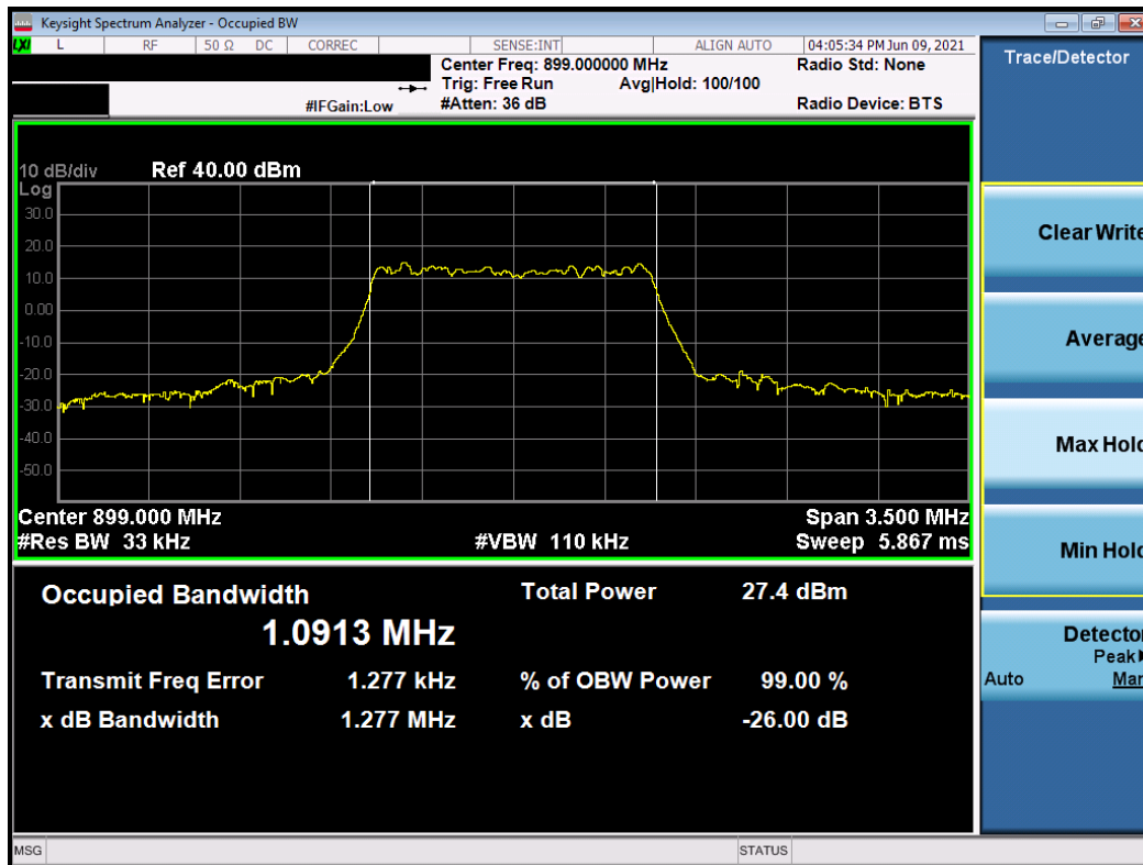
Plot 7-7. Occupied Bandwidth Plot (1.4MHz, QPSK, RB 6, RB Offset 0, NB=0)
