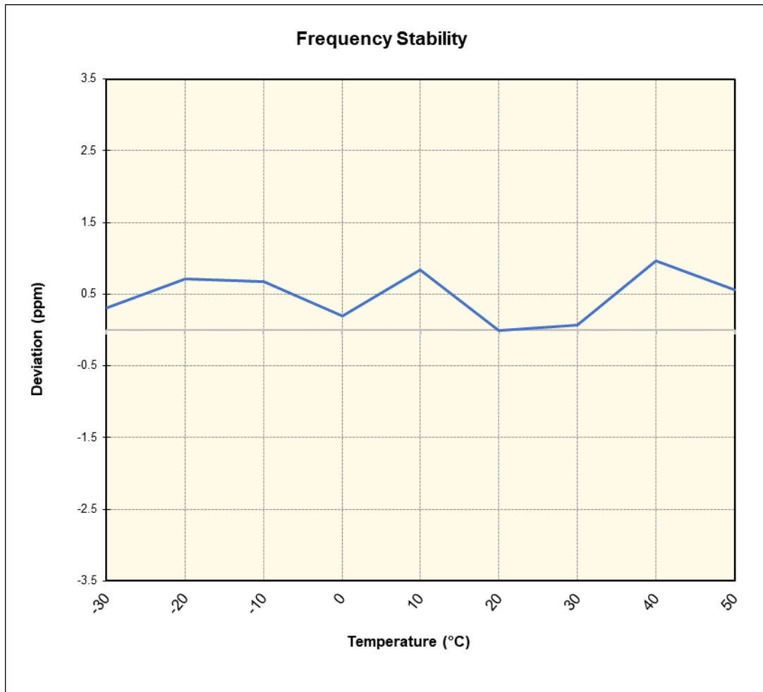
Plot 7-32. LTE Band 8 CAT-M1 Frequency Stability Chart
