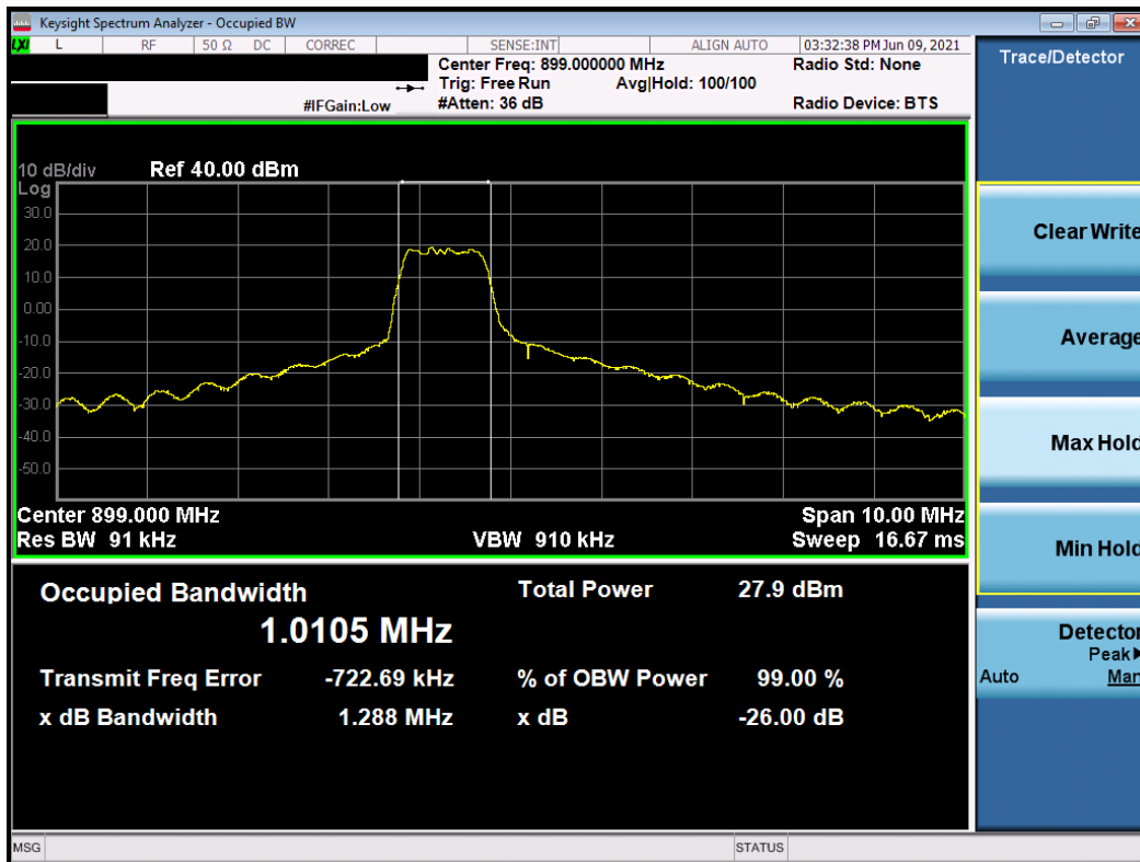
Plot 7-3. Occupied Bandwidth Plot (3MHz, 16-QAM, RB 5, RB Offset 0, NB=0)
