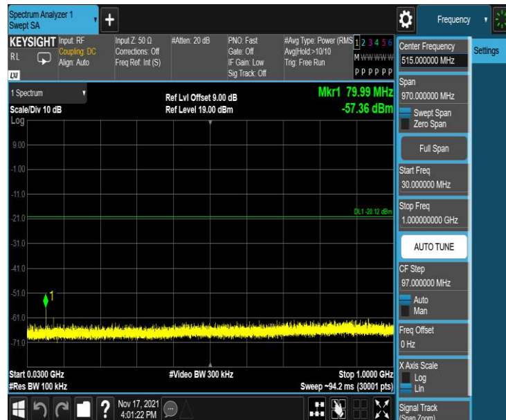
11G_Ant1_2437_30~1000
