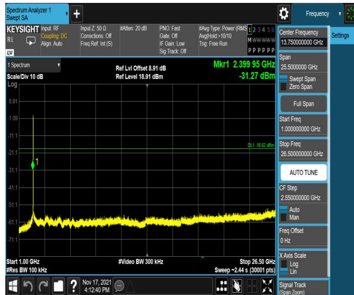
11N20SISO_Ant1_2412_1000~26500
