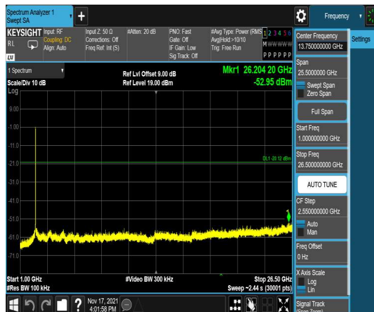
11G_Ant1_2437_1000~26500
