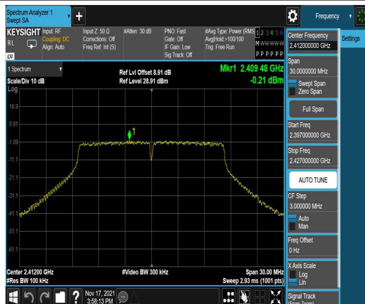
11G_Ant1_2412_0~Reference
