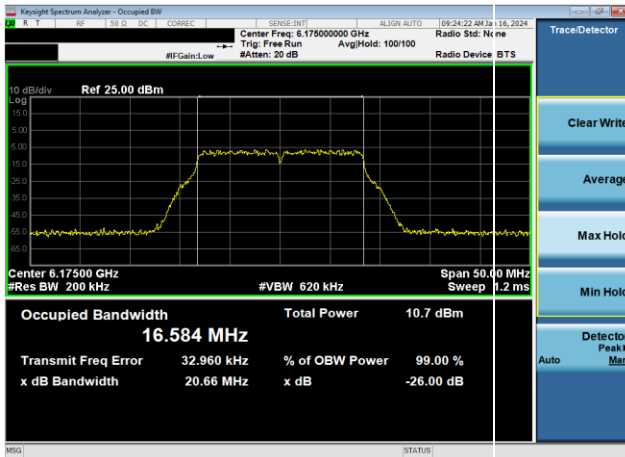
Plot 7-21. 26dB & 99% Bandwidth Plot Antenna WF5B (20MHz 802.11a (UNII Band 5) – Ch. 45, 24Mbps)
