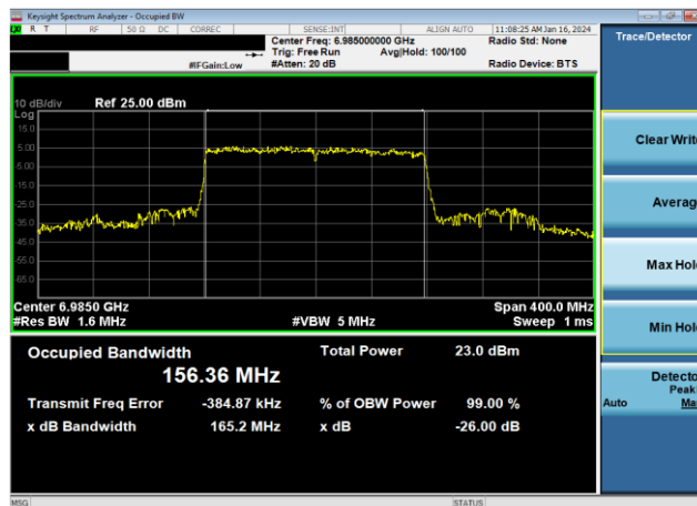
Plot 7-60. 26dB & 99% Bandwidth Plot Antenna WF5B (160MHz 802.11ax (UNII Band 8) – Ch. 207, MCS11)
