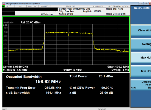
Plot 7-40. 26dB & 99% Bandwidth Plot Antenna WF5B (160MHz 802.11ax (UNII Band 8) – Ch. 207, MCS4)
