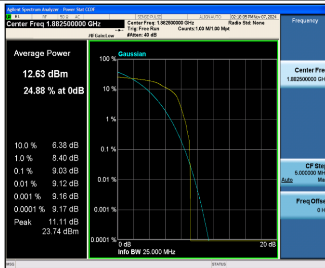
Band25-15MHz-16QAM-26365-1-0-Low-9.03-&lt;=13-PASS
