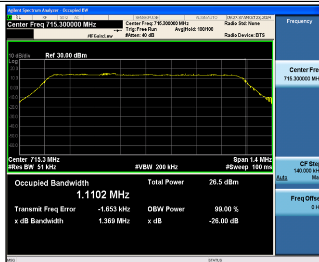
Band12-1.4MHz-16QAM-23173-6-0-Low-1.1102-1.369-PASS
