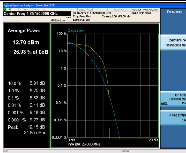
Band25-15MHz-16QAM-26115-6-0-Low-8.88-&lt;=13-PASS
