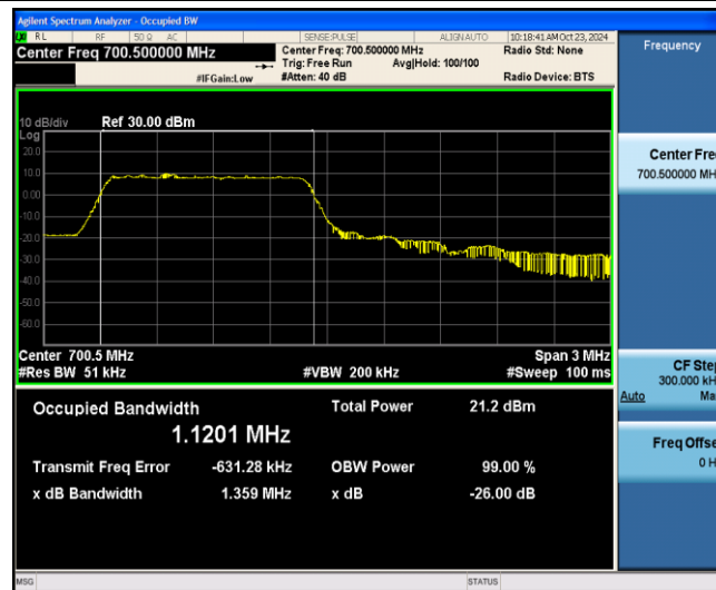
Band12-3MHz-QPSK-23025-6-0-Low-1.1201-1.359-PASS
