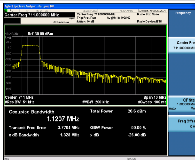
Band12-10MHz-16QAM-23130-6-0-Low-1.1207-1.328-PASS
