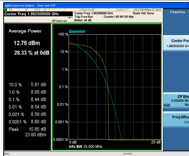
Band25-15MHz-QPSK-26365-1-0-Low-8.44-&lt;=13-PASS
