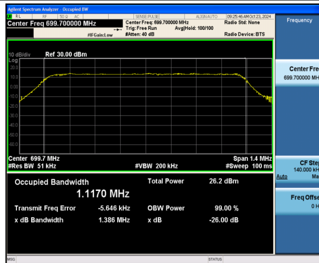
Band12-1.4MHz-16QAM-23017-6-0-Low-1.1170-1.386-PASS
