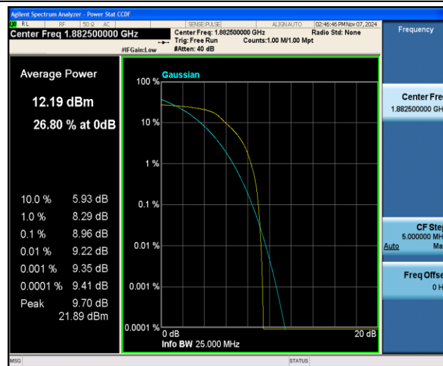
Band25-20MHz-16QAM-26365-6-0-Low-8.96-&lt;=13-PASS
