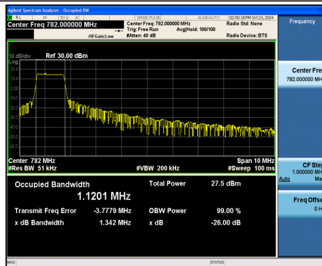
Band13-10MHz-16QAM-23230-6-0-Low-1.1201-1.342-PASS
