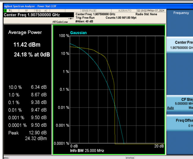
Band25-15MHz-16QAM-26615-1-0-Low-9.38-&lt;=13-PASS
