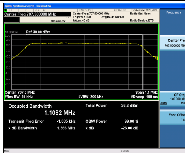
Band12-1.4MHz-16QAM-23095-6-0-Low-1.1082-1.366-PASS
