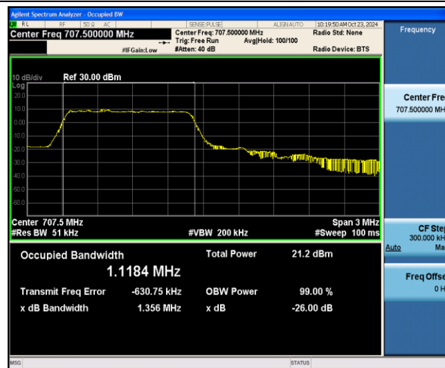
Band12-3MHz-QPSK-23095-6-0-Low-1.1184-1.356-PASS
