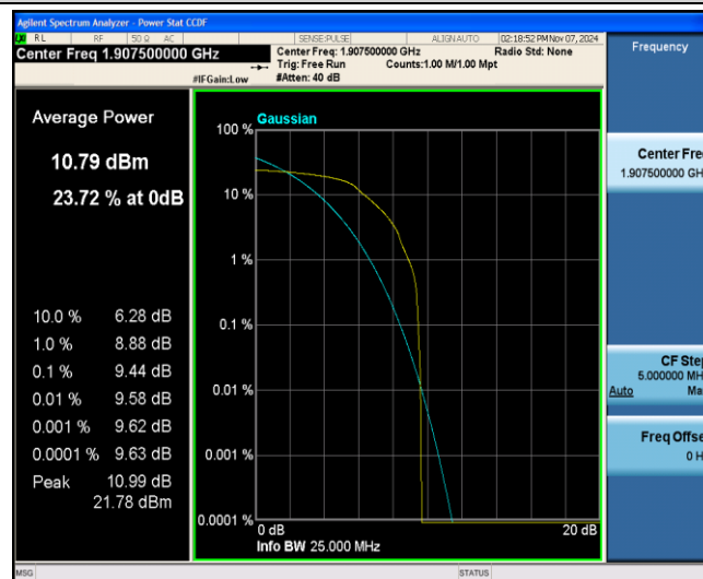
Band25-15MHz-QPSK-26615-1-0-Low-9.44-&lt;=13-PASS
