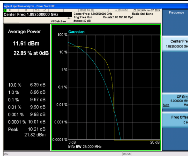
Band25-15MHz-16QAM-26365-6-0-Low-9.67-&lt;=13-PASS
