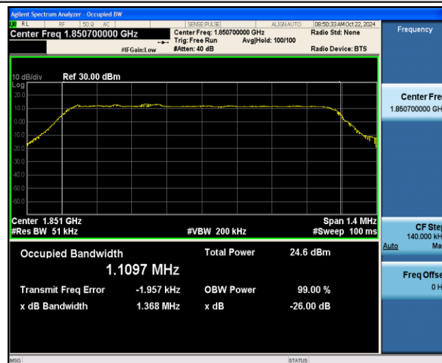
Band2-1.4MHz-QPSK-18607-6-0-Low-1.1097-1.368-PASS
