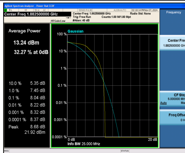
Band25-15MHz-QPSK-26365-6-0-Low-8.04-&lt;=13-PASS
