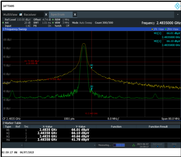
Upper Band Edge Peak & Average Measurement
