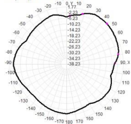
Total(H-XY), Max= 1.77dBi, CirD=8.31
