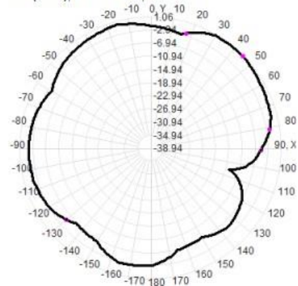
Total(H-XY), Max= 0.76dBi, CirD=15.12
