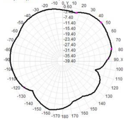
Total(H-XY), Max= 0.60dBi, CirD=15.08
