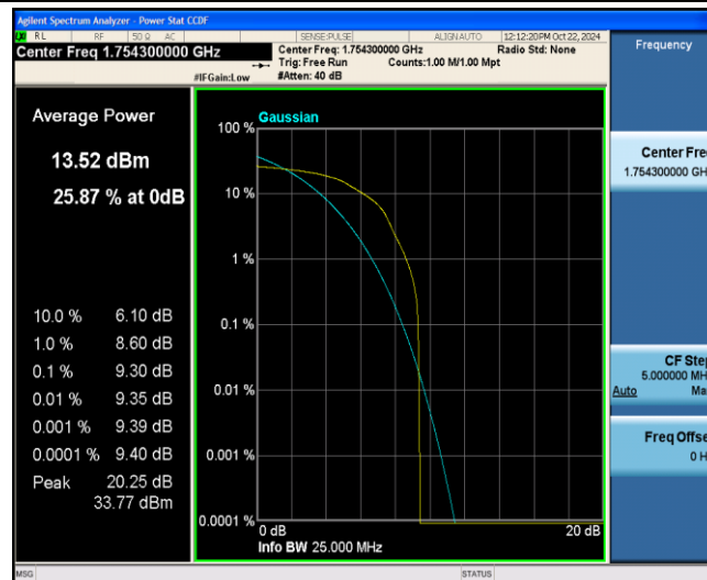
Band4-1.4MHz-16QAM-20393-1-0-Low-9.30- &lt;=13-PASS
