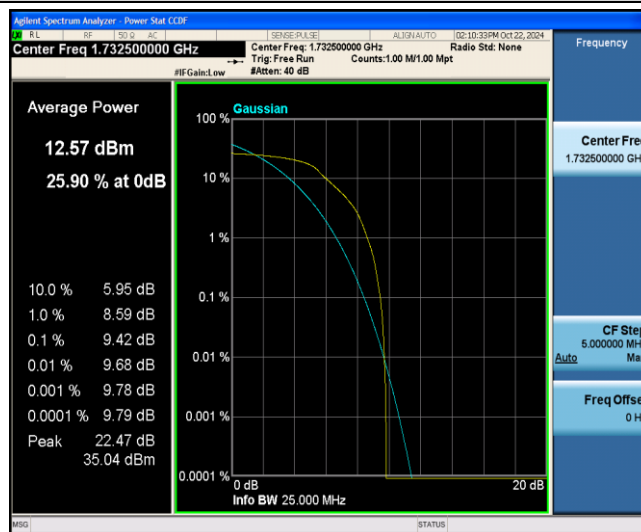
Band4-10MHz-16QAM-20175-6-0-Low-9.42-=&lt;=13-PASS
