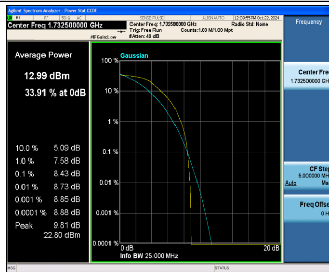
Band4-1.4MHz-QPSK-20175-6-0-Low-8.43-&lt;=13-PASS
