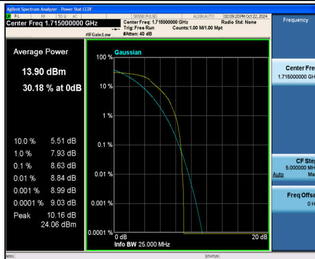
Band4-10MHz-16QAM-20000-6-0-Low-8.63-&lt;=13-PASS
