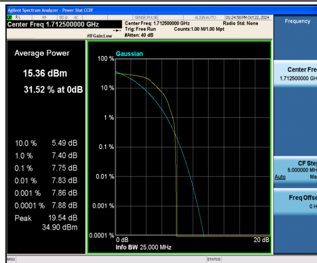
Band4-5MHz-QPSK-19975-1-0-Low-7.75-&lt;=13-PASS
