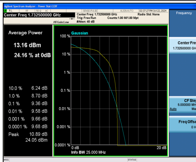
Band4-15MHz-16QAM-20175-6-0-Low-9.36-=&lt;=13-PASS
