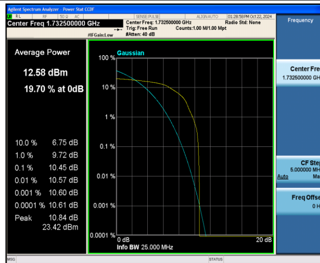
Band4-5MHz-16QAM-20175-1-0-Low-10.45-&lt;=13-PASS
