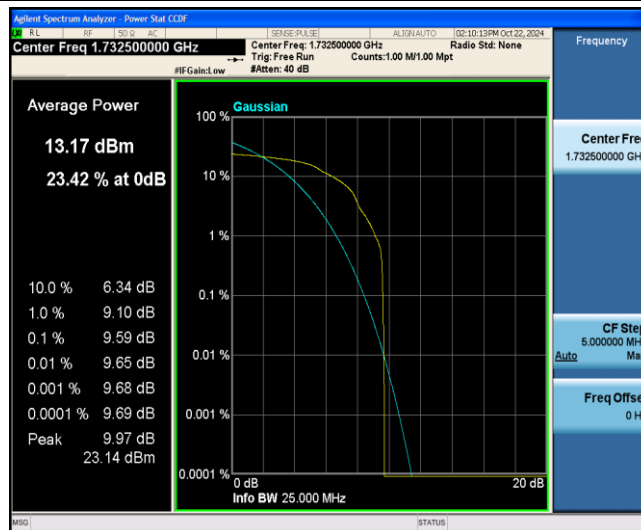
Band4-10MHz-16QAM-20175-1-0-Low-9.59-=&lt;=13-PASS
