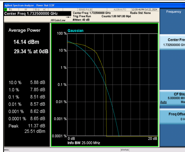
Band4-1.4MHz-16QAM-20175-1-0-Low-8.51- &lt;=13-PASS
