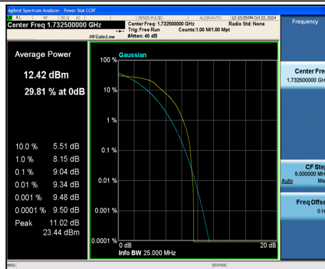
Band4-1.4MHz-16QAM-20175-6-0-Low-9.04- &lt;=13-PASS
