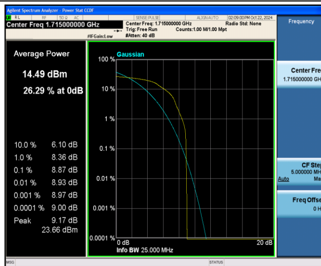
Band4-10MHz-16QAM-20000-1-0-Low-8.87-&lt;=13-PASS
