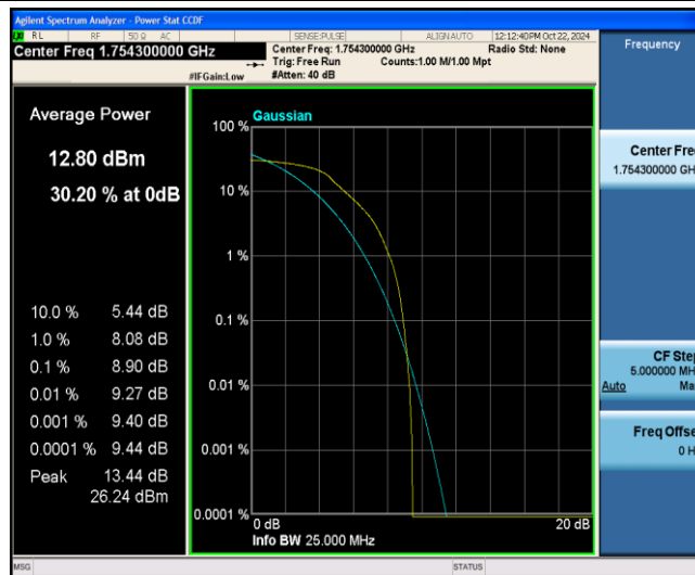
Band4-1.4MHz-16QAM-20393-6-0-Low-8.90-&lt;=13-PASS
