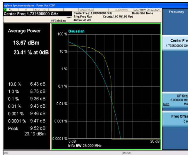
Band4-15MHz-16QAM-20175-1-0-Low-9.36-=&lt;=13-PASS
