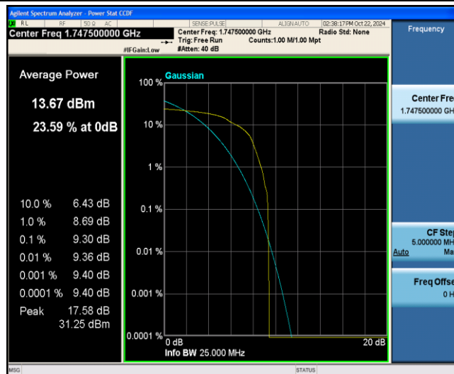
Band4-15MHz-16QAM-20325-1-0-Low-9.30-=&lt;=13-PASS
