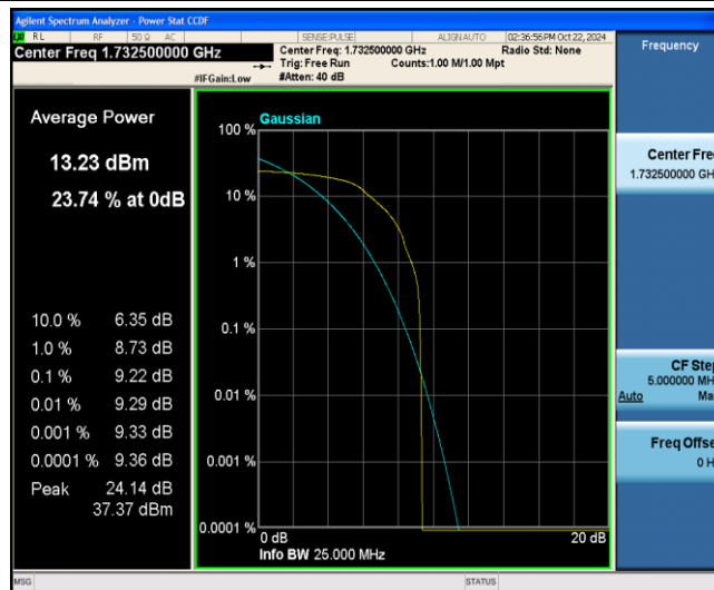
Band4-15MHz-QPSK-20175-1-0-Low-9.22-&lt;=13-PASS
