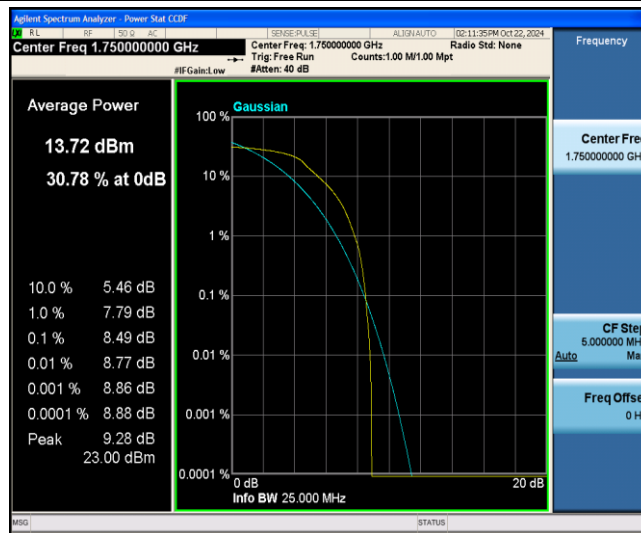
Band4-10MHz-QPSK-20350-6-0-Low-8.49-&lt;=13-PASS
