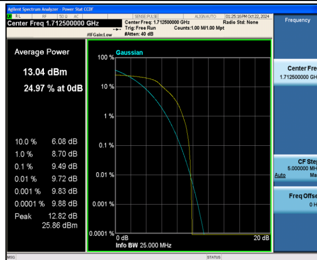
Band4-5MHz-QPSK-19975-6-0-Low-9.49-&lt;=13-PASS
