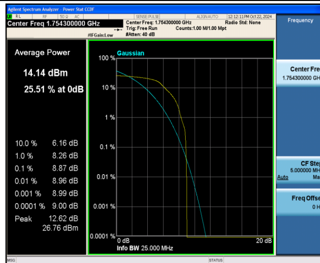
Band4-1.4MHz-QPSK-20393-1-0-Low-8.87-&lt;=13-PASS
