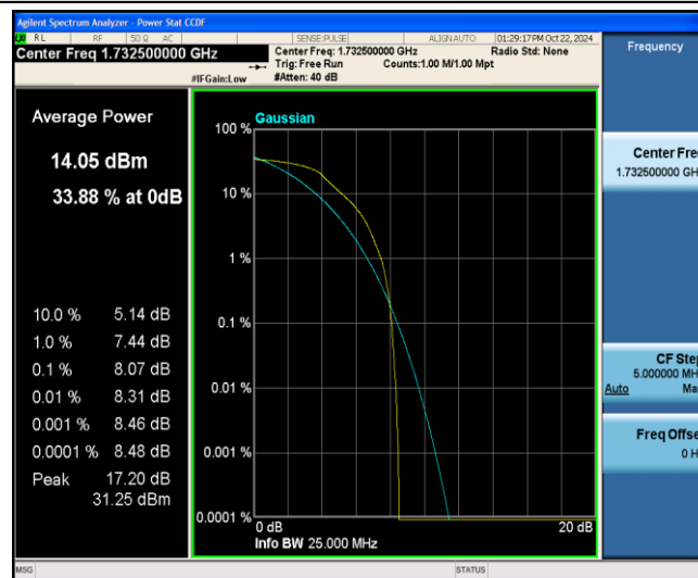
Band4-5MHz-16QAM-20175-6-0-Low-8.07-&lt;=13-PASS
