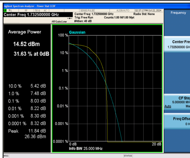
Band4-15MHz-QPSK-20175-6-0-Low-8.03-&lt;=13-PASS
