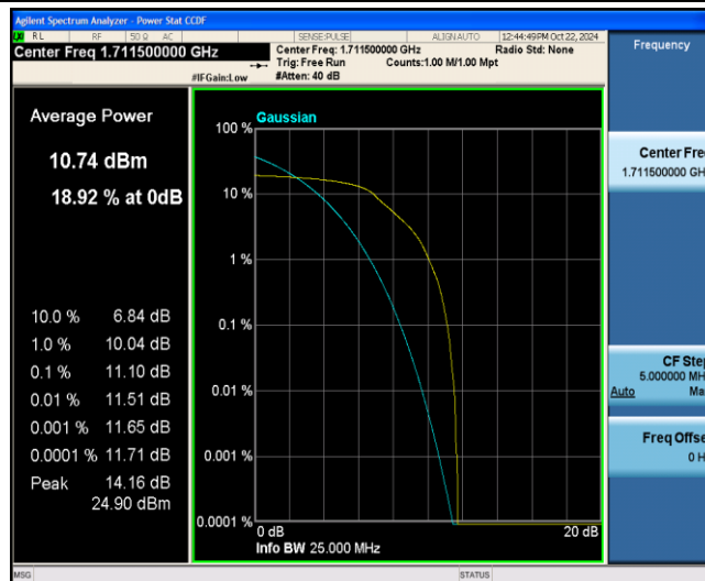
Band4-3MHz-QPSK-19965-6-0-Low-11.10-&lt;=13-PASS
