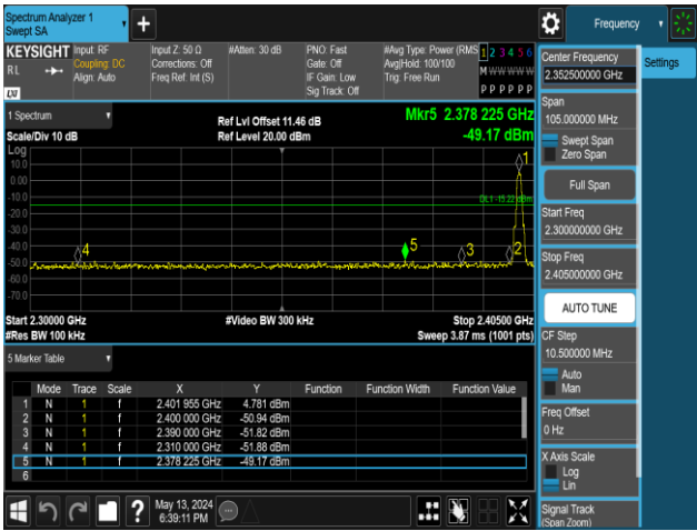
BLE_1M-Ant1-2402-PASS
