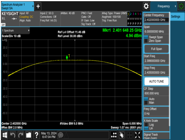
BLE_2M-Ant1-2402-PASS
