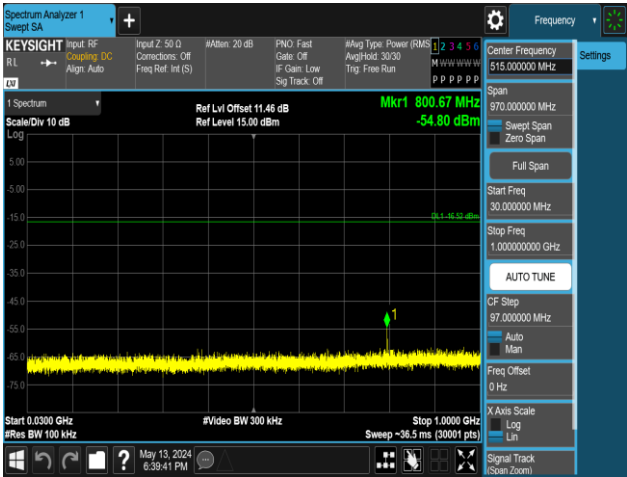
BLE_1M-Ant1-2402-30~1000-PASS
