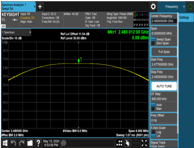
BLE_2M-Ant1-2480-PASS
