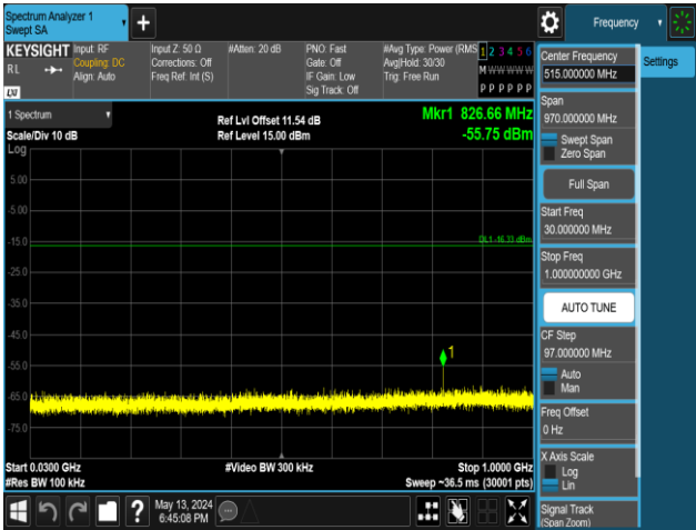
BLE_1M-Ant1-2480-30~1000-PASS
