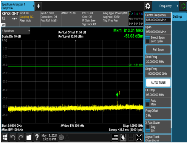
BLE_1M-Ant1-2440-30~1000-PASS
