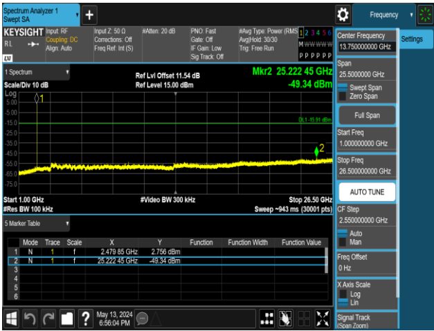
BLE_2M-Ant1-2480-1000~26500-PASS
