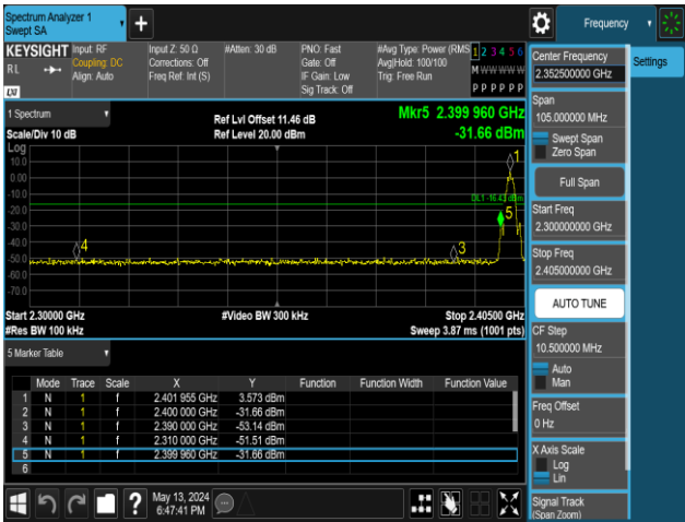
BLE_2M-Ant1-2402-PASS
