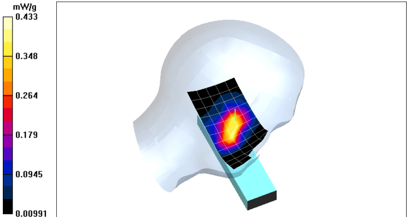
Fig. 25: SAR distribution for slider up, PCS 1900, channel 661, cheek position, left side of head. (19.05.2003; Ambient Temperature: 20.9° C; Liquid Temperature : 18.7° C).
