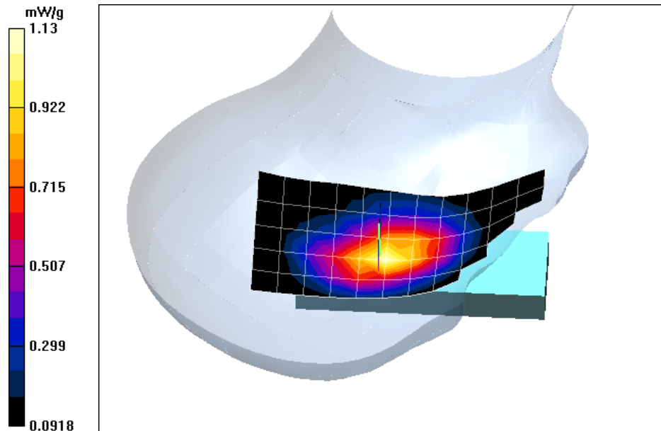
Fig. 15: Worst case SAR distribution for slider down, channel 128, cheek position, right side of head (18.06.2003; Ambient Temperature: 21.1° C; Liquid Temperature : 20.0° C).
