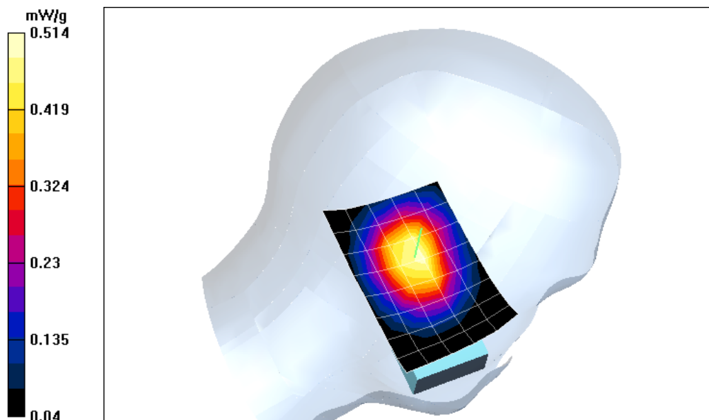
Fig. 6: SAR distribution for slider down, GSM 850, channel 190, tilted position, left side of head. (20.05.2003; Ambient Temperature: 21.1° C; Liquid Temperature : 20.1° C).
