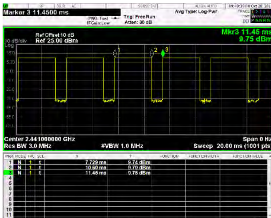
Time-domain plot for Bluetooth transmission signal
