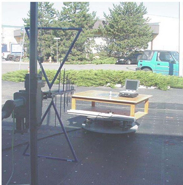
Photograph B.7-7 - Dipole Substitution Setup
