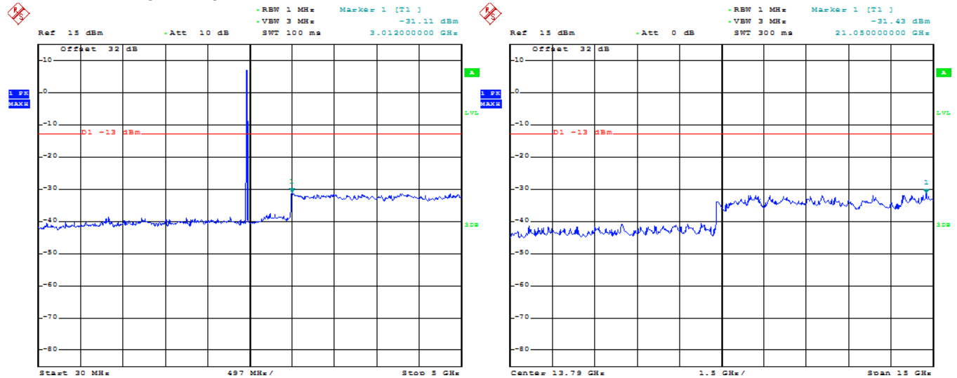
Figure 1-49: Spurious RF Conducted Emissions Single Freq., Static PBRS, DH5
