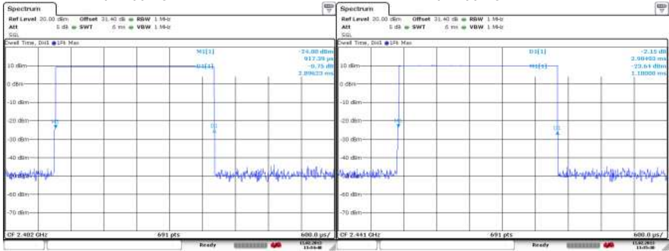
Figure 1-23: Time of Occupancy (Dwell Time) Freq. Hopping, Static PBRS, DH5
