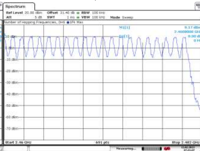
Figure 1-16: Number of Hopping Frequencies Static PBRS, DH5
