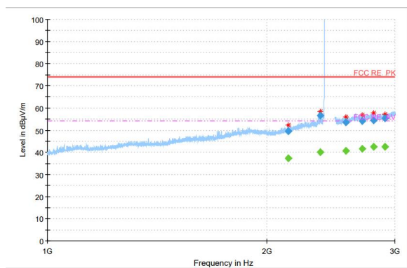
Bandedge:Ch0
