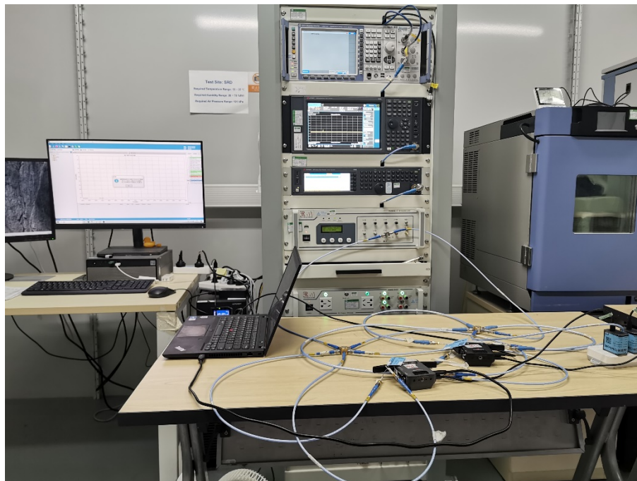
Photograph 1: Set-up photo for DFS Conducted Signal test
