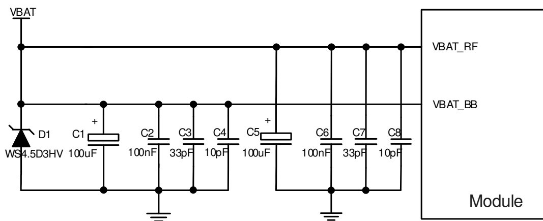
Figure 7: Star Structure of the Power Supply
