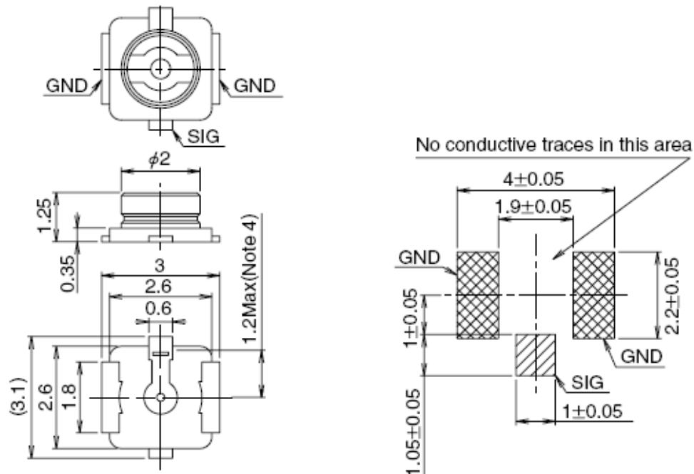
Figure 38: Dimensions of the U.FL-R-SMT Connector (Unit: mm)
