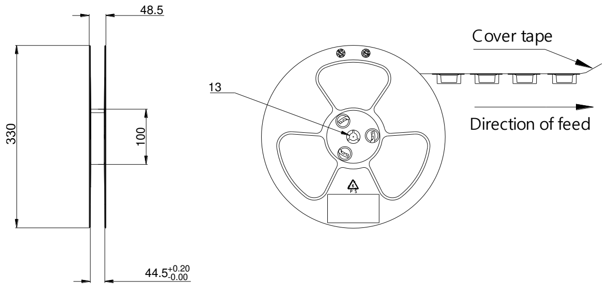
Figure 50: Reel Specifications
