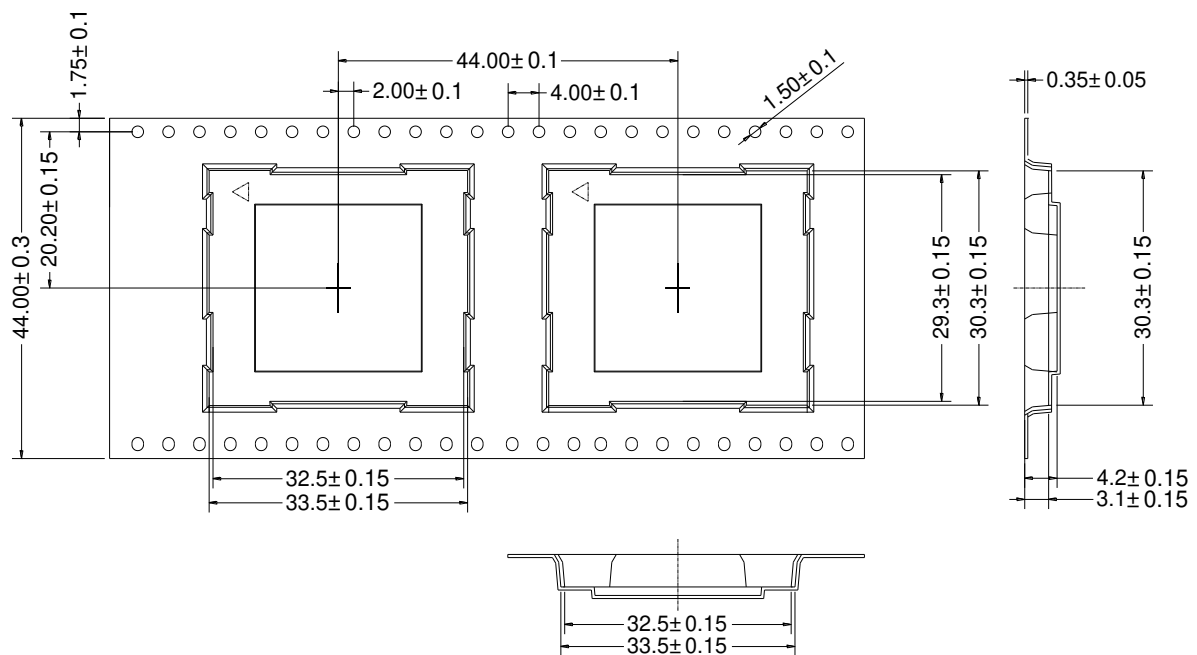
Figure 49: Tape Specifications
