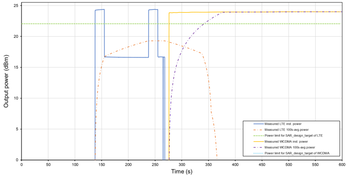
Conducted Tx Power for TAS to non-TAS H.O Tech: LTE, Band 66/ Tech: WCDMA, Band 4
