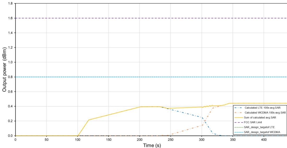
Total Time Averaged SAR Change in Tech/Band Tech: LTE, Band 66 / Tech: WCDMA, Band 2
