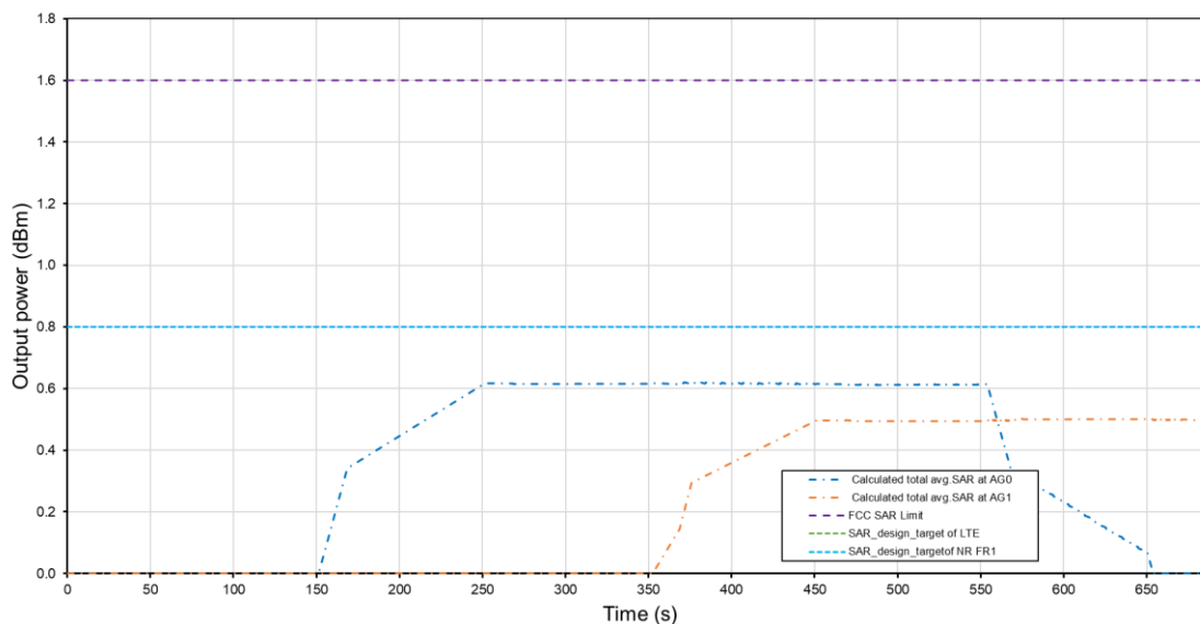
Total Time Averaged NSA with Spatial TAS Tech: LTE, Band 2, Ant A / Tech: NR FR1, n66, Ant F
