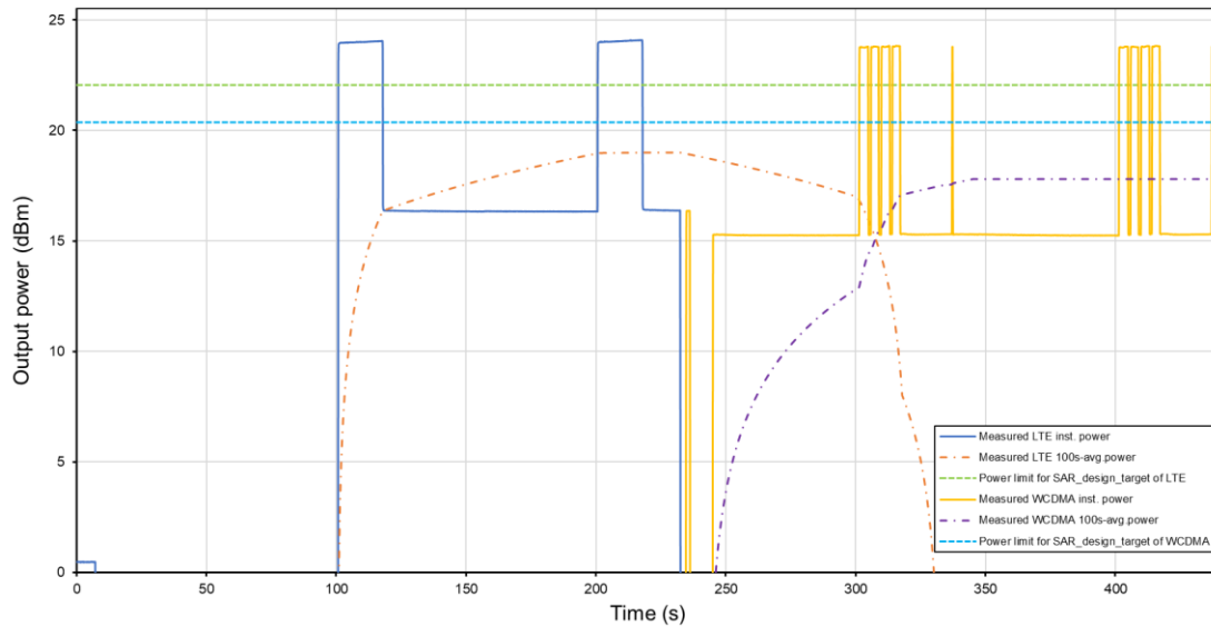
Conducted Tx Power for Change in Tech/Band Tech: LTE, Band 66 / Tech: WCDMA, Band 2
