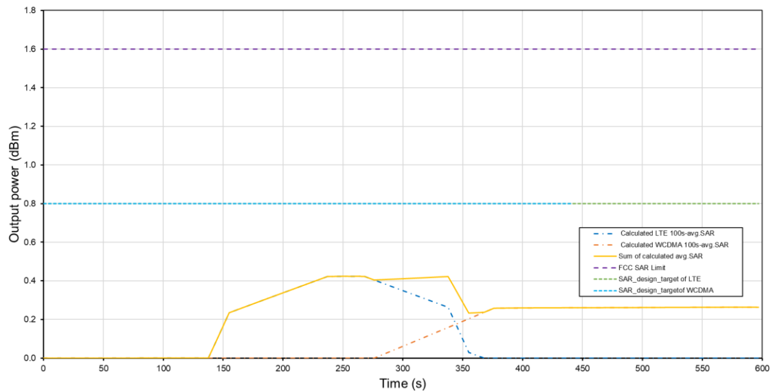
Total Time Averaged TAS to non-TAS H.O Tech: LTE, Band 66/ Tech: WCDMA, Band 4
