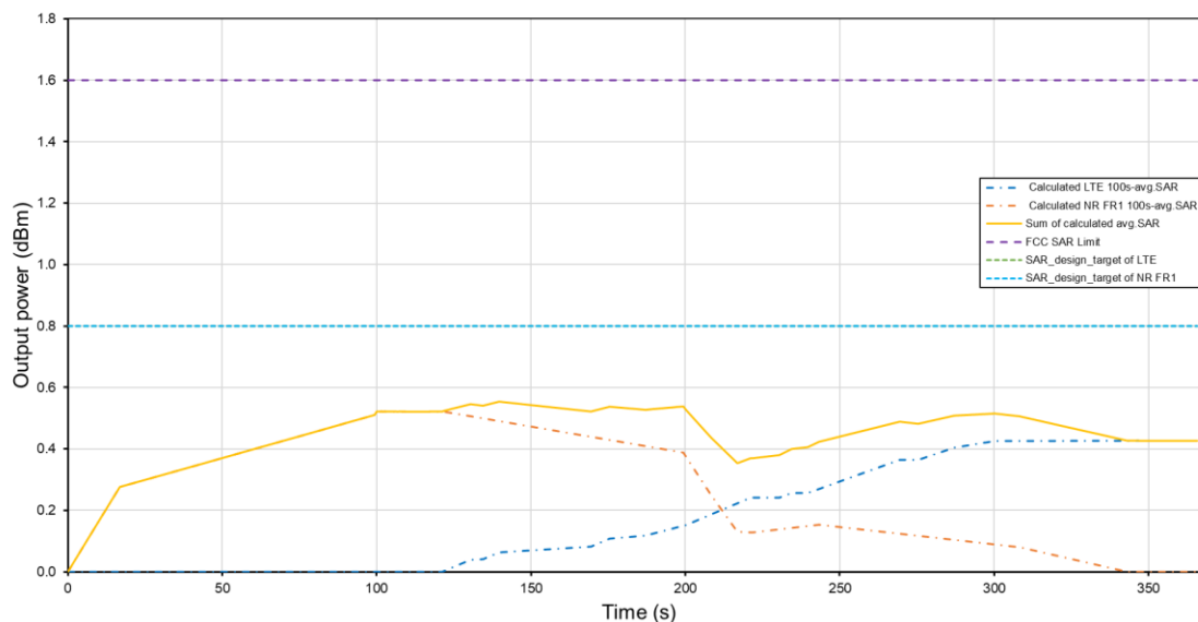
Total Time Averaged SAR Exposure Switching EN-DC Tech: LTE, Band 5, Antenna A / Tech: NR FR1, Band n66, Antenna A
