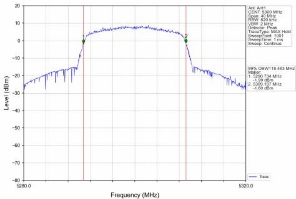
802.11n(HT20)_MCH_5300MHz_Ant1_NTNV
