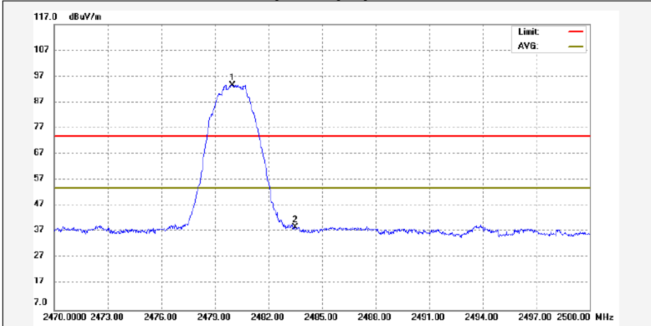
8DPSK Transmitting Band edge-right side Vertical
