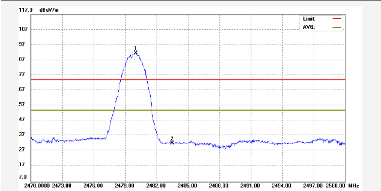
8DPSK Transmitting Band edge-right side Horizontal
