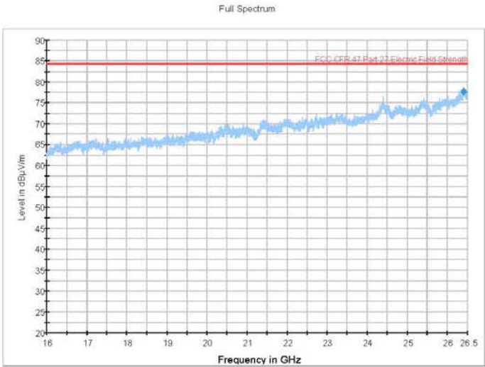
Figure 407 Radiated Emission 16 GHz – 26.5 GHz (2501.0 MHz) (10MHz Channel BW)
