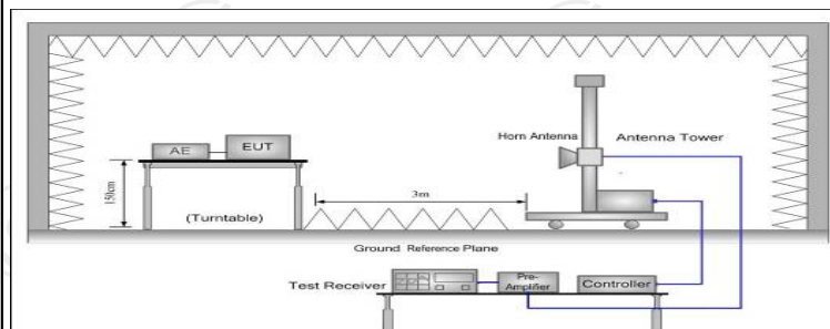
Above 1GHz
