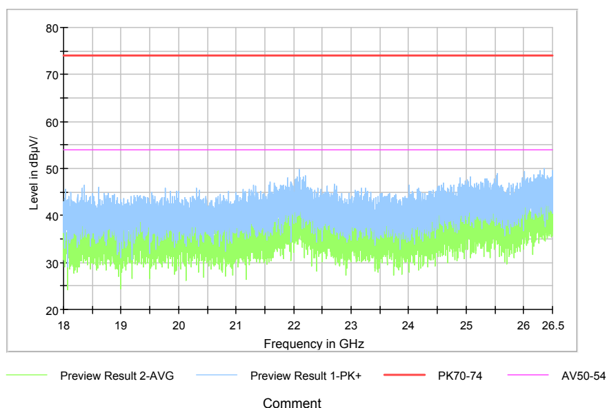
Pic11. Radiated emission (18GHz – 26GHz)
