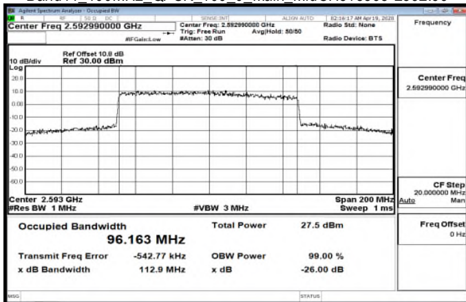
Band41_100MHz_QPSK_100_0_Main_MidCH518598-2592.99
