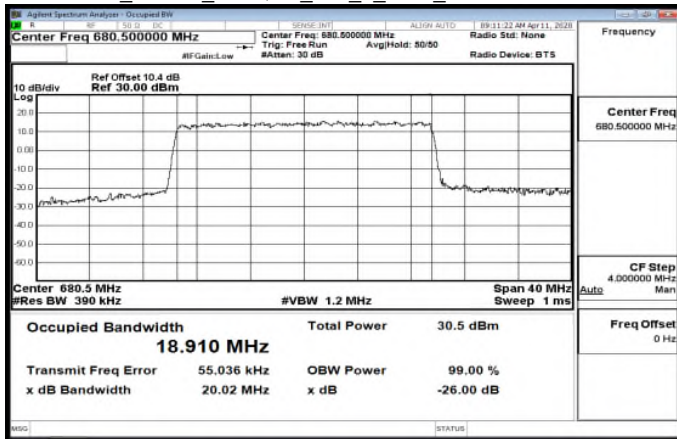
Band71_20MHz_QPSK_100_0_Main_MidCH136100-680.5
