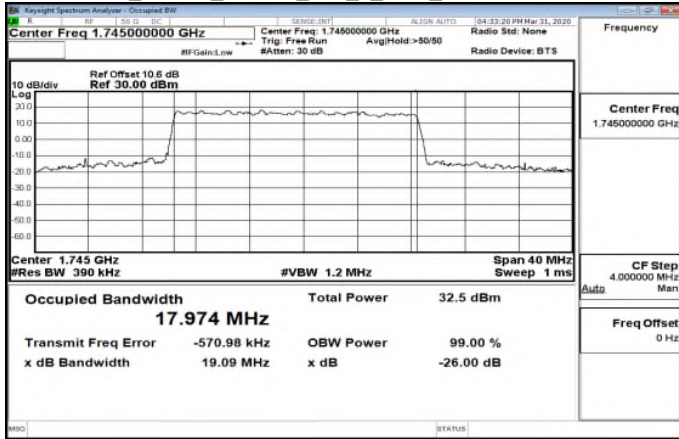
Band66 20MHz_64QAM_100_0_Main_MidCH349000-1745
