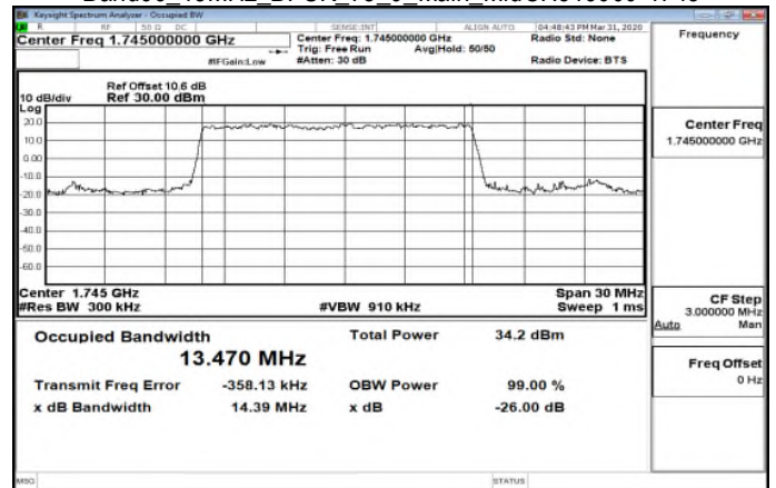
Band66_15MHz_BPSK_75_0_Main_MidCH349000-1745
