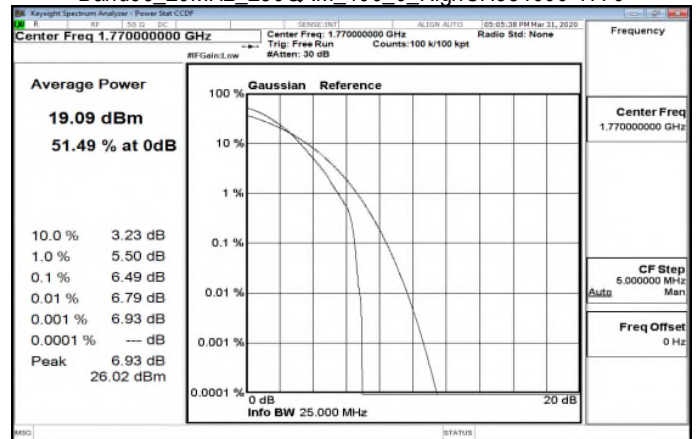
Band66_20MHz_256QAM_100_0_HighCH354000-1770
