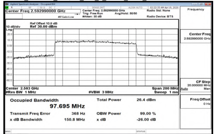
Band41_100MHz_16QAM_100_0_worse_Main_MidCH518598-2592.99
