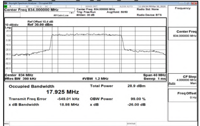
Band5_20MHz_16QAM_100_0_worse_Main_LowCH166800-834
