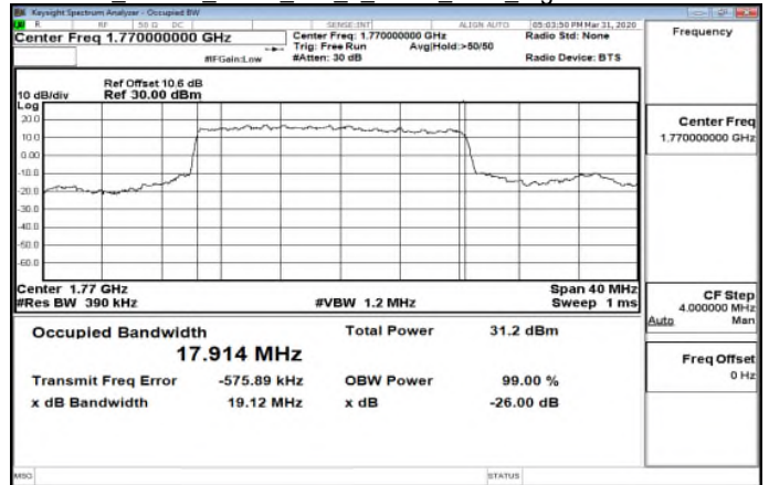
Band66_20MHz_BPSK_100_0_worse_Main_HighCH354000-1770
