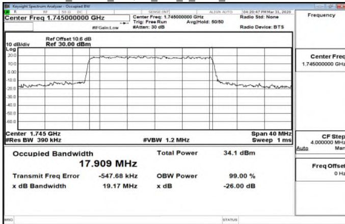
Band66_20MHz_64QAM_100_0_Main_MidCH349000-1745
