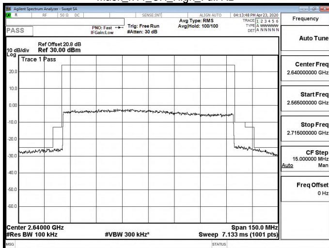
Mask_n41_CH_High_Full RB
