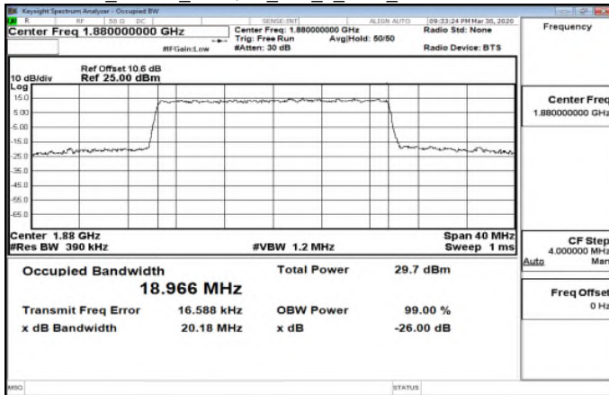
Band2_20MHz_QPSK_100_0_Main_MidCH376000-1880
