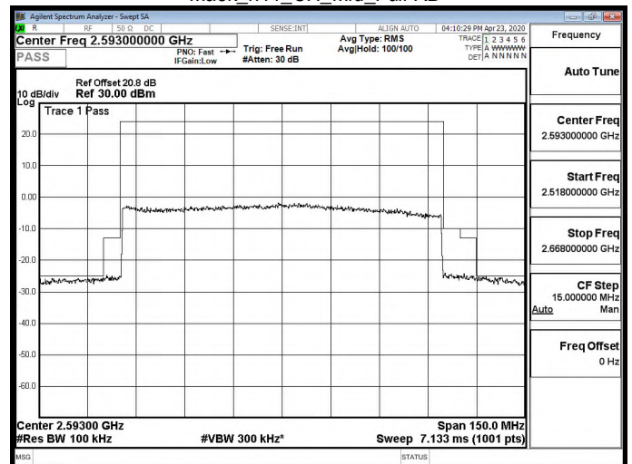
Mask_n41_CH_Mid_Full RB
