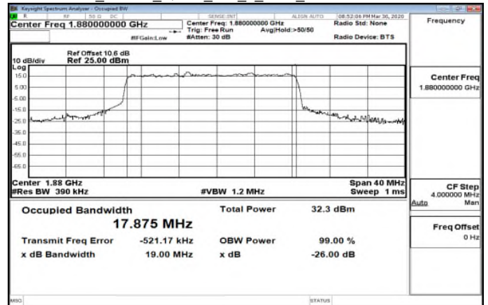
Band2_20MHz_16QAM_100_0_Main_MidCH376000-1880
