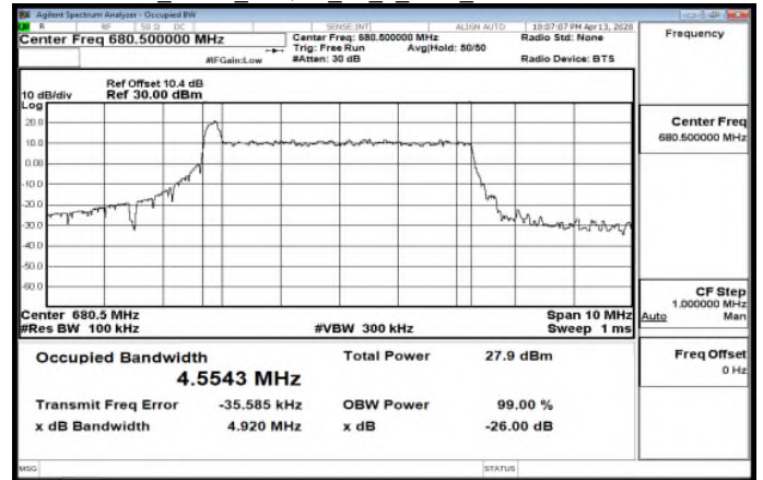
Band71 5MHz_64QAM_25_0_Main_MidCH136100-680.5
