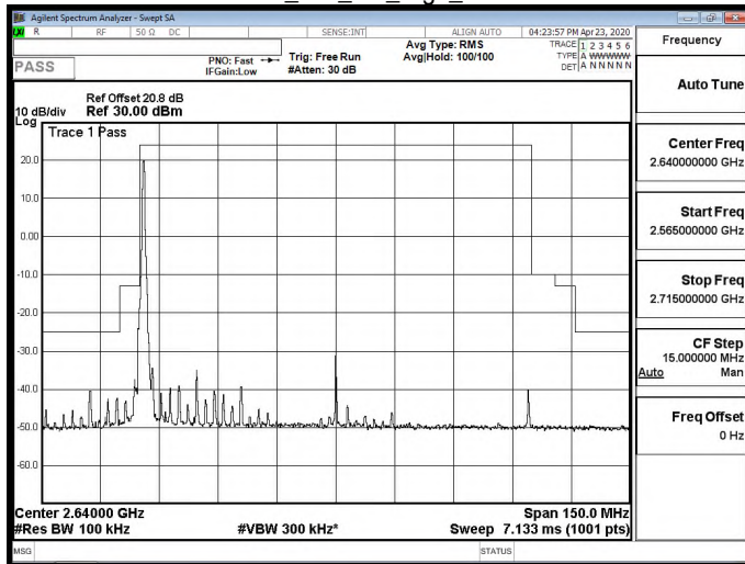
Mask_n41_CH_High_1RBMax
