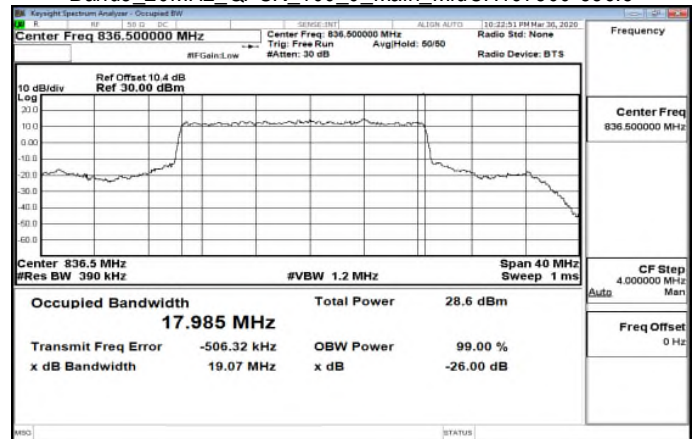
Band5_20MHz_QPSK_100_0_Main_MidCH167300-836.5
