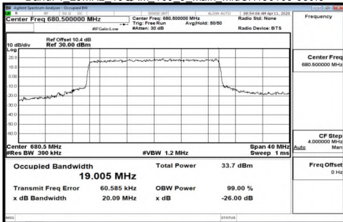
Band71_20MHz_16QAM_100_0_Main_MidCH136100-680.5
