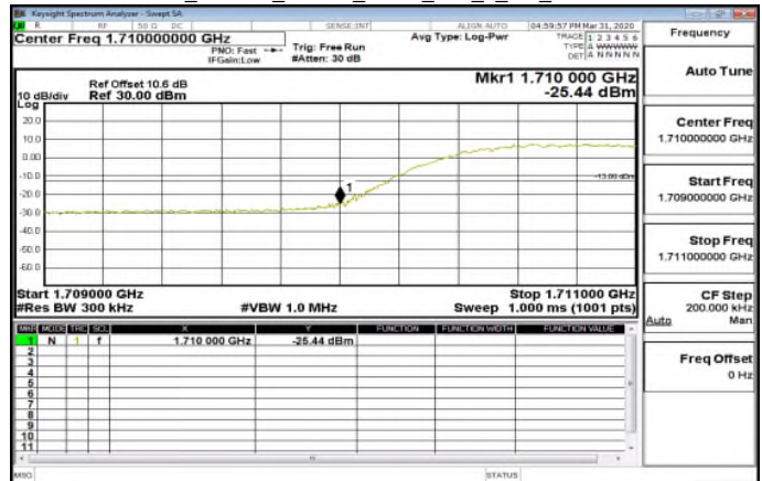
DFT-s-OFDM Pi/2_Band66_20MHz_BPSK_100_0_CH_LowCH344000-1720
