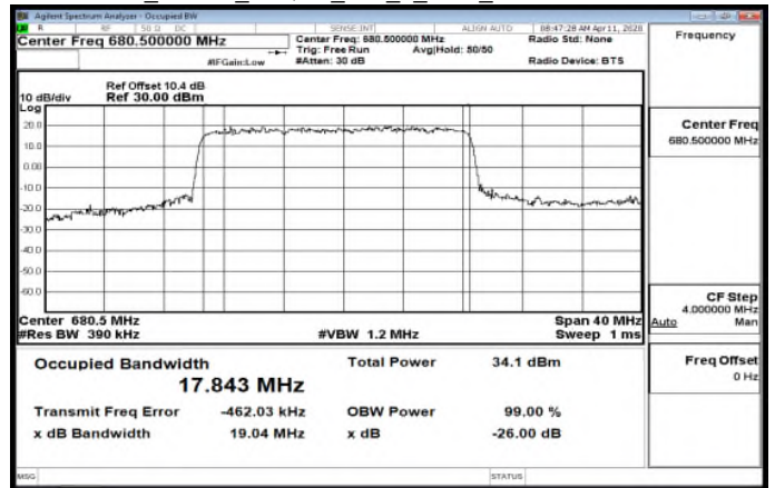
Band71_20MHz_256QAM_100_0_Main_MidCH136100-680.5
