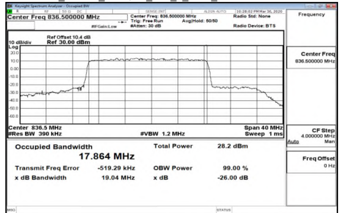
Band5_20MHz_BPSK_100_0_Main_MidCH167300-836.5
