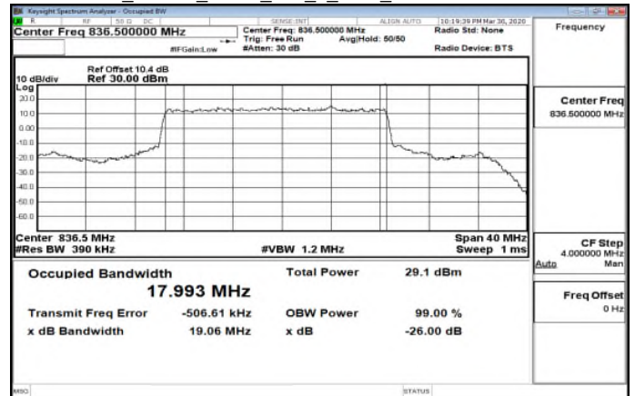
Band5_20MHz_QPSK_100_0_Main_MidCH167300-836.5
