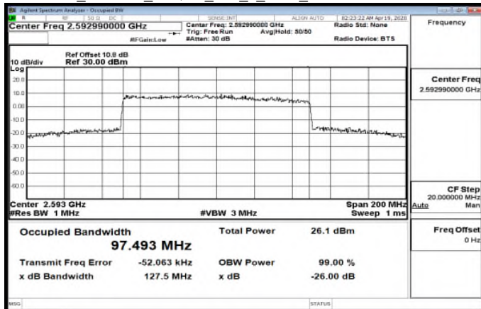
Band41_100MHz_256QAM_100_0_Main_MidCH518598-2592.99
