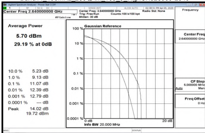
Band41_100MHz_256QAM_100_0_HighCH528000-2640
