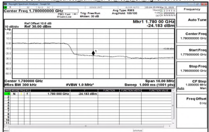
DFT-s-OFDM Pi/2_Band66_20MHz_BPSK_100_0_CH_HighCH354000-1770
