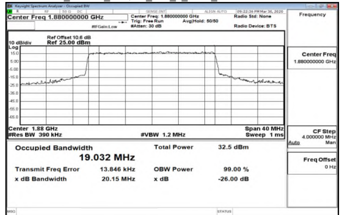
Band2_20MHz_64QAM_100_0_Main_MidCH376000-1880
