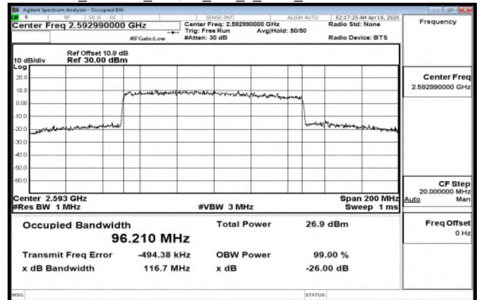
Band41_100MHz_64QAM_100_0_Main_MidCH518598-2592.99
