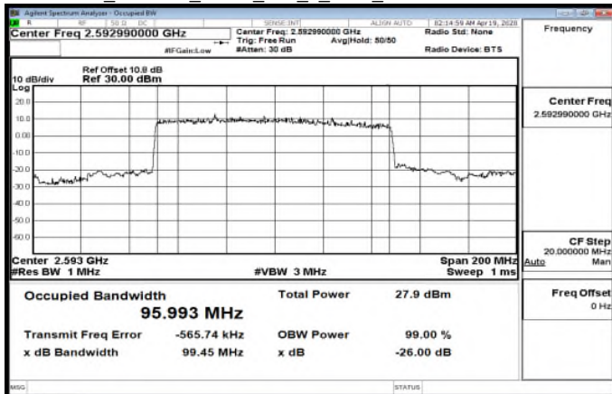
Band41_100MHz_BPSK_100_0_Main_MidCH518598-2592.99
