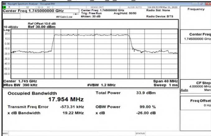
Band66 20MHz_16QAM_100_0_Main_MidCH349000-1745
