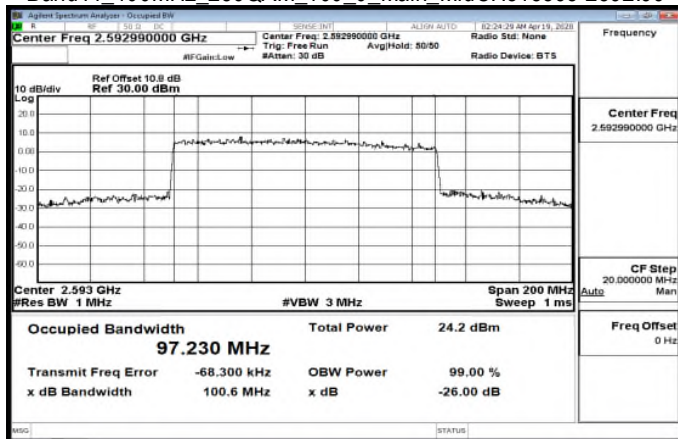
Band41_100MHz_256QAM_100_0_Main_MidCH518598-2592.99
