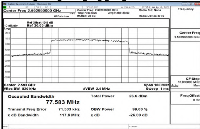
Band41_80MHz_16QAM_100_0_Main_MidCH518598-2592.99
