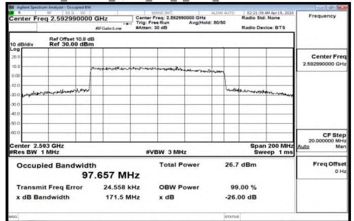
Band41_100MHz_16QAM_100_0_Main_MidCH518598-2592.99
