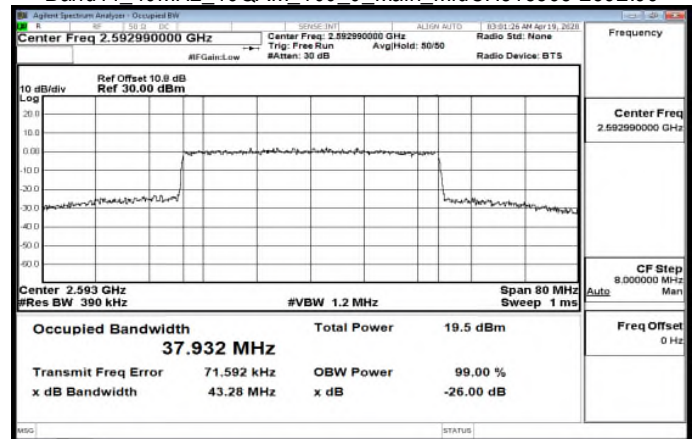
Band41 40MHz_16QAM_100_0_Main_MidCH518598-2592.99
