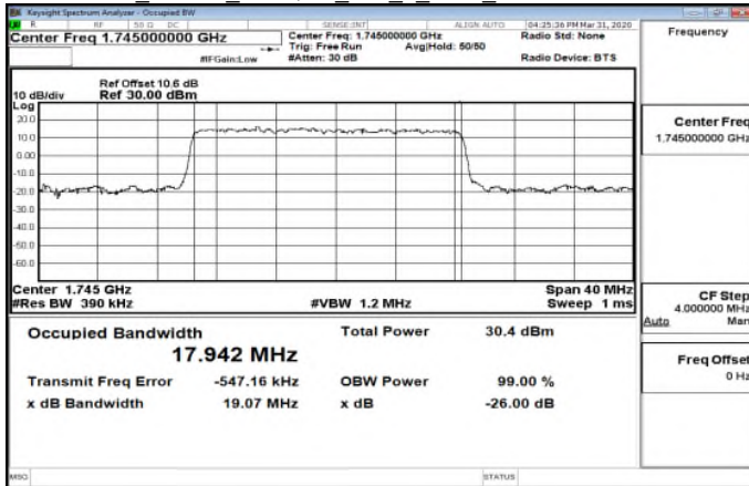
Band66_20MHz_256QAM_100_0_Main_MidCH349000-1745
