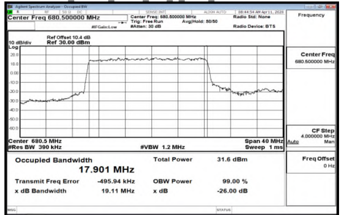
Band71_20MHz_BPSK_100_0_Main_MidCH136100-680.5
