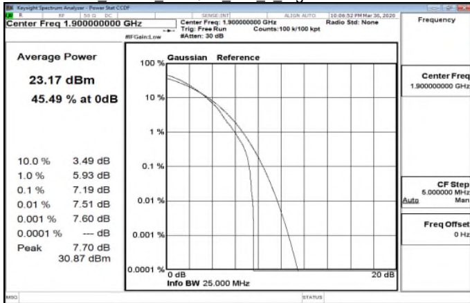
Band2_20MHz_256QAM_100_0_HighCH380000-1900
