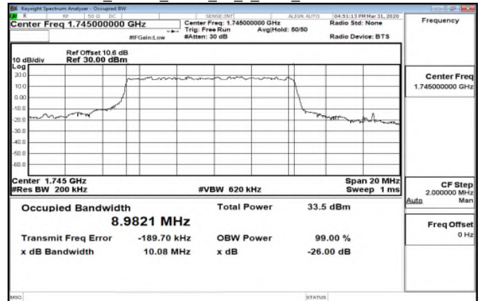
Band66_10MHz_BPSK_50_0_Main_MidCH349000-1745
