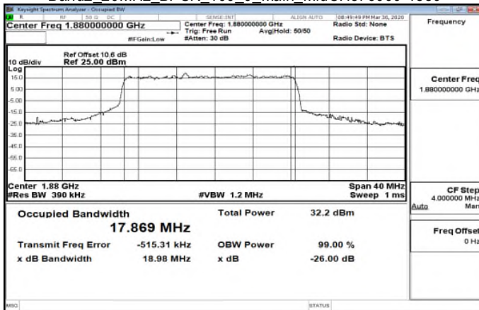
Band2_20MHz_BPSK_100_0_Main_MidCH376000-1880
