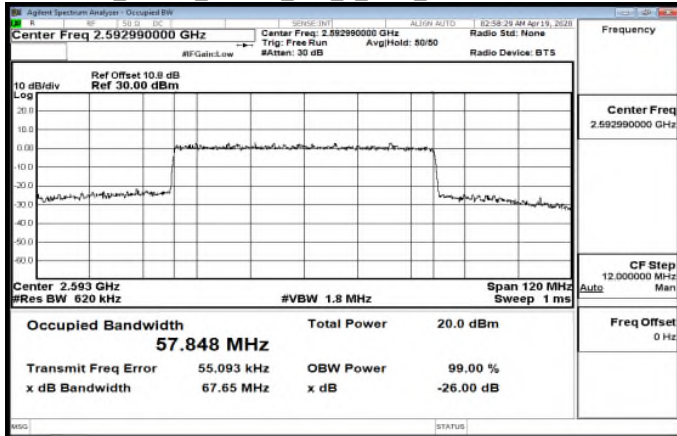
Band41_60MHz_16QAM_100_0_Main_MidCH518598-2592.99
