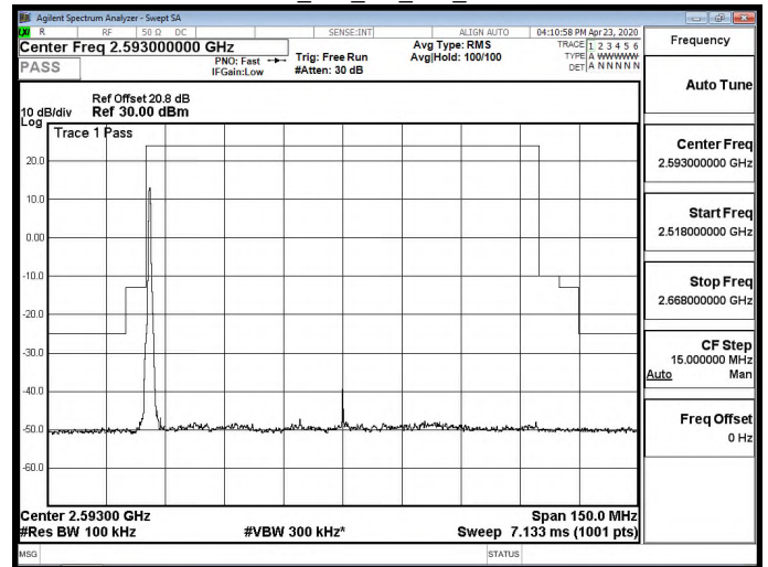
Mask_n41_CH_Mid_1RBmax
