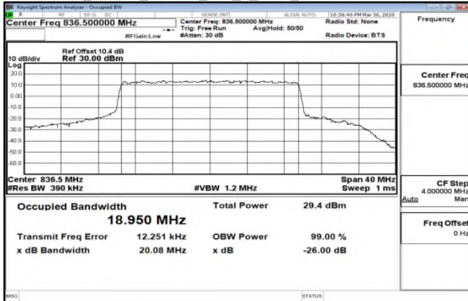
Band5 20MHz_256QAM_100_0_Main_MidCH167300-836.5
