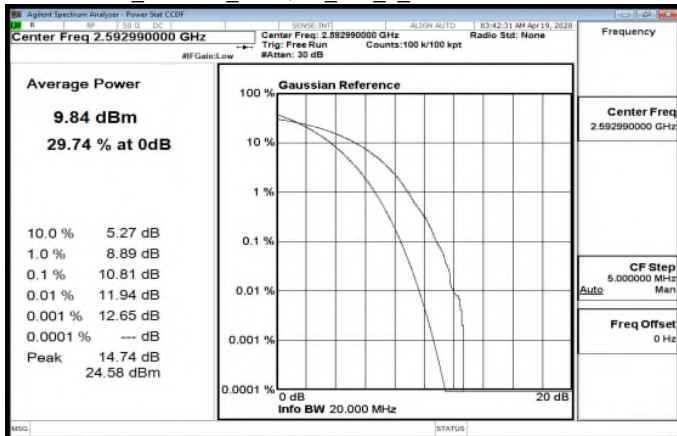
Band41_100MHz_256QAM_100_0_MidCH518598-2592.99
