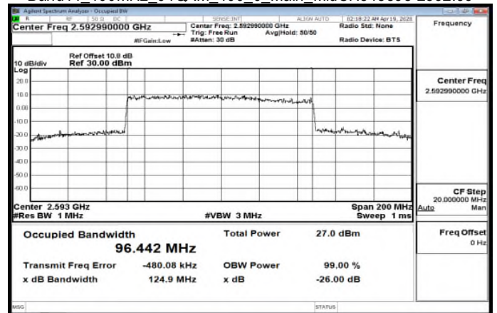
Band41_100MHz_64QAM_100_0_Main_MidCH518598-2592.99
