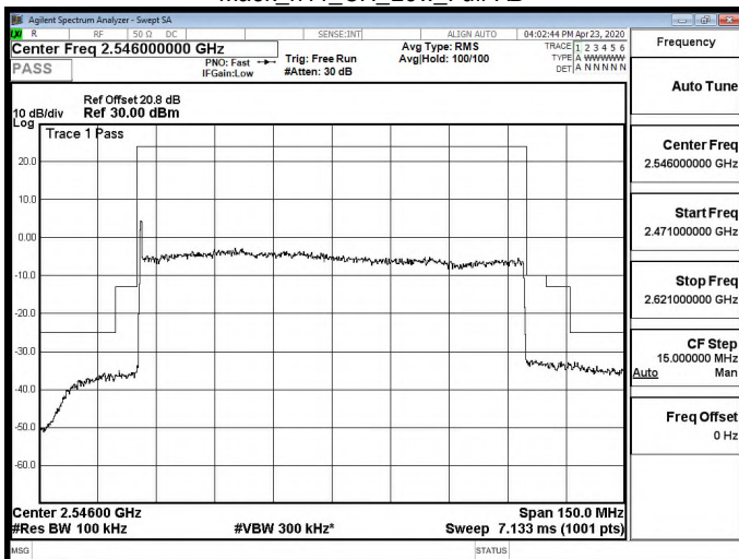
Mask_n41_CH_Low_Full RB
