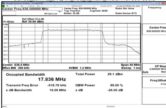
Band5_20MHz_64QAM_100_0_Main_MidCH167300-836.5
