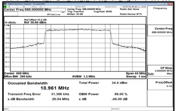
Band71_20MHz_64QAM_100_0_worse_Main_HighCH137600-688
