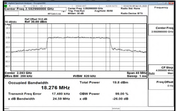
Band41 40MHz_16QAM_100_0_Main_MidCH518598-2592.99
