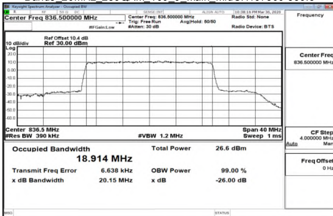
Band5 20MHz_256QAM_100_0_Main_MidCH167300-836.5
