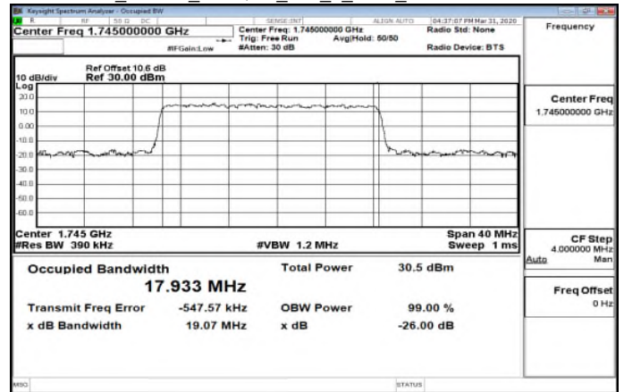
Band66 20MHz_QPSK_100_0_Main_MidCH349000-1745
