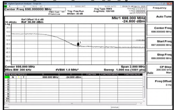
CP-OFDM_Band71_20MHz_64QAM_100_0_CH_HighCH137600-688
