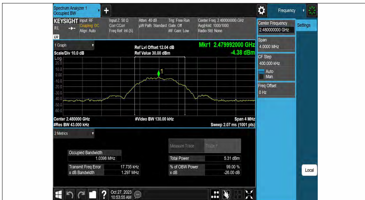
GFSK 1M-Ant1-2480
