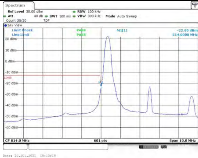
Band26-5MHz-16QAM-26715-1RB#24
