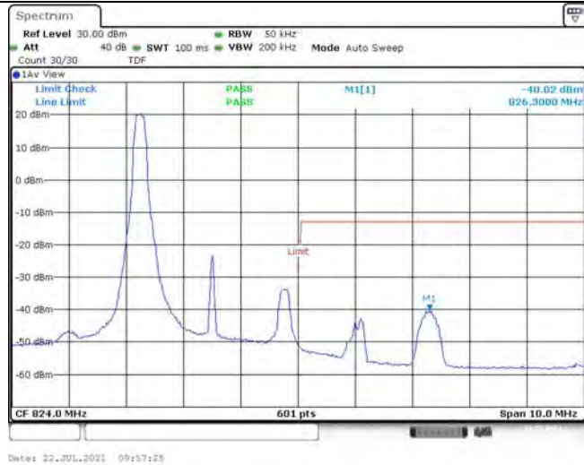
Band26-3MHz-16QAM-26775-1RB#14
