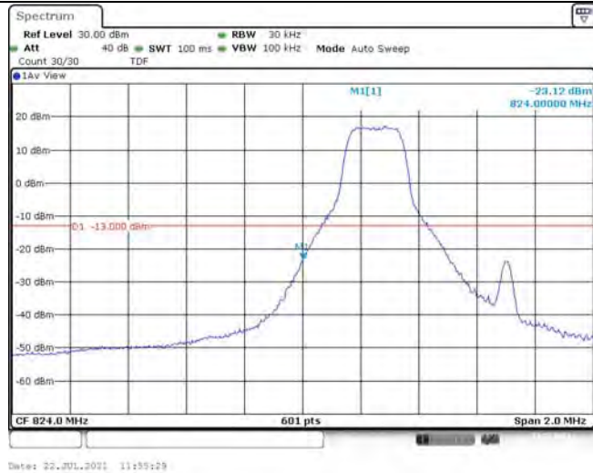
Band26-1.4MHz-16QAM-26797-1RB#5
