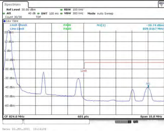
Band26-5MHz-16QAM-26765-1RB#24
