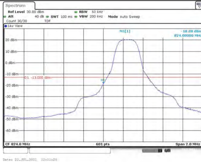
Band26-3MHz-QPSK-26805-1RB#14
