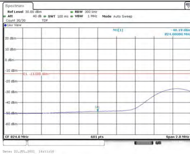
Band26-15MHz-QPSK-26865-75RB#0
