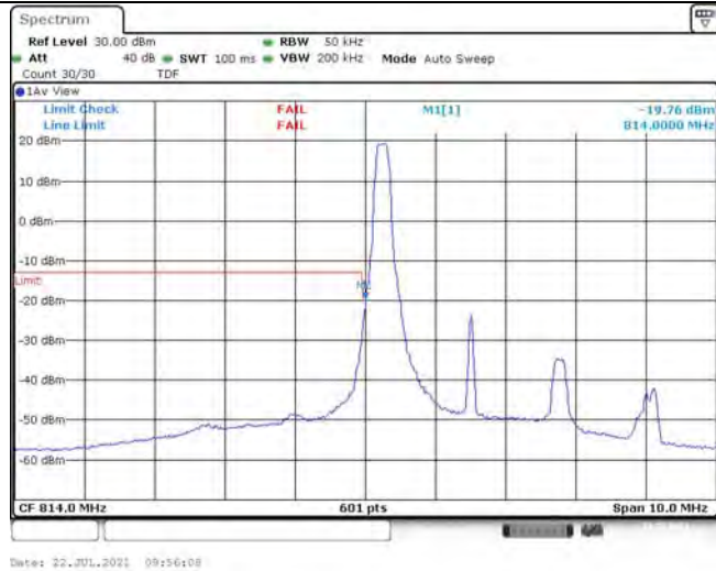
Band26-3MHz-16QAM-26705-1RB#14
