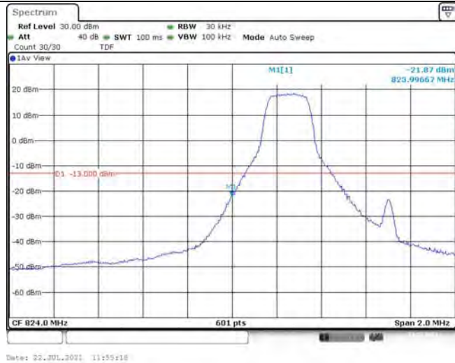
Band26-1.4MHz-QPSK-26797-1RB#5
