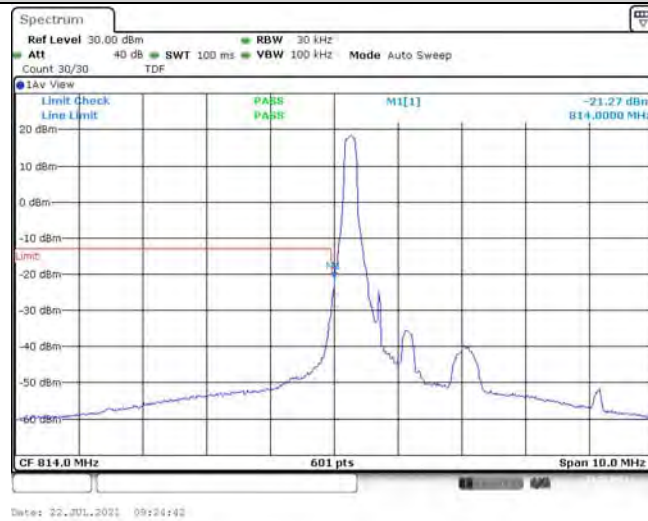
Band26-1.4MHz-QPSK-26697-1RB#5
