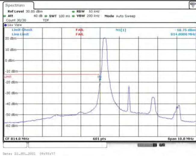
Band26-3MHz-QPSK-26705-1RB#14
