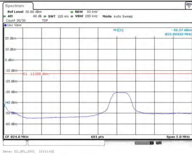
Band26-3MHz-16QAM-26805-15RB#0
