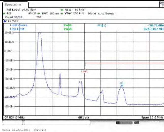
Band26-3MHz-QPSK-26775-1RB#14
