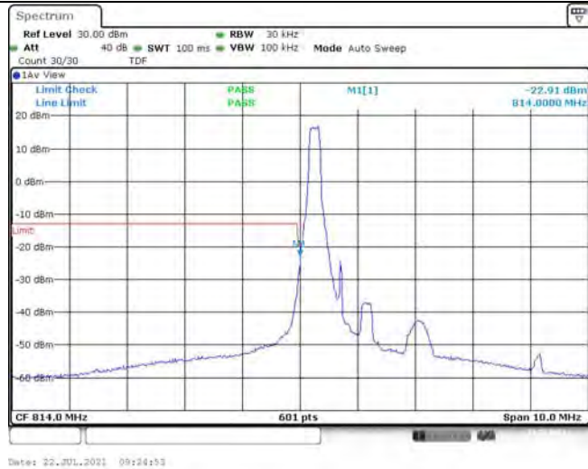
Band26-1.4MHz-16QAM-26697-1RB#5
