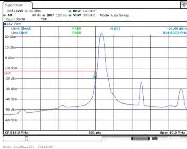
Band26-5MHz-QPSK-26715-1RB#24
