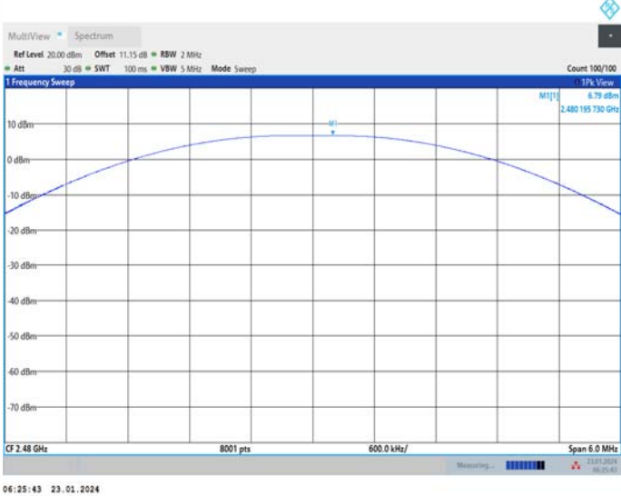
BLE_1M_Ant1_2480
