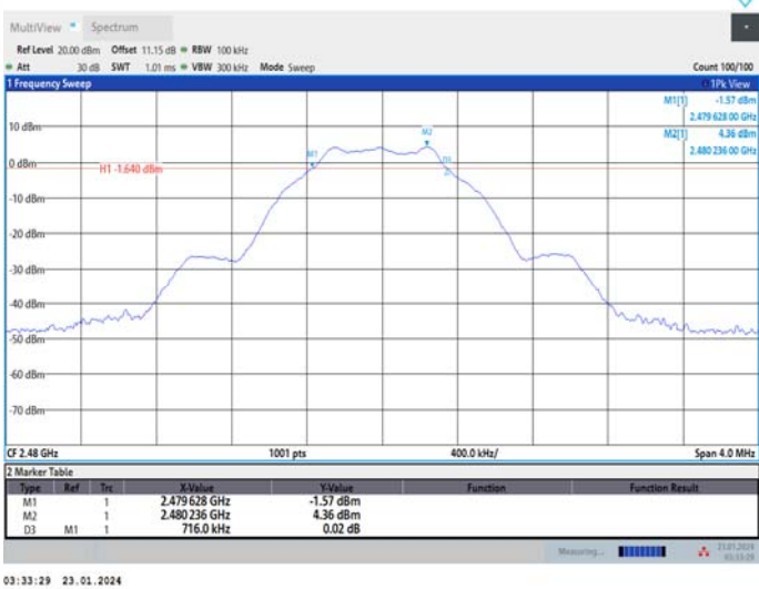
BLE_1M_Ant1_2480
