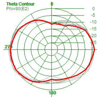
Efficiency: 71.3%
