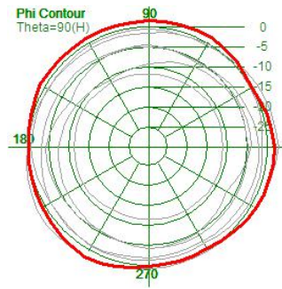
Gain: 2.26dBi
