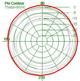
Gain: 2.31dBi
