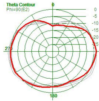
Efficiency: 70.4%
