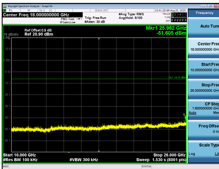
RF Conducted Spurious Emissions_DH5_2480
