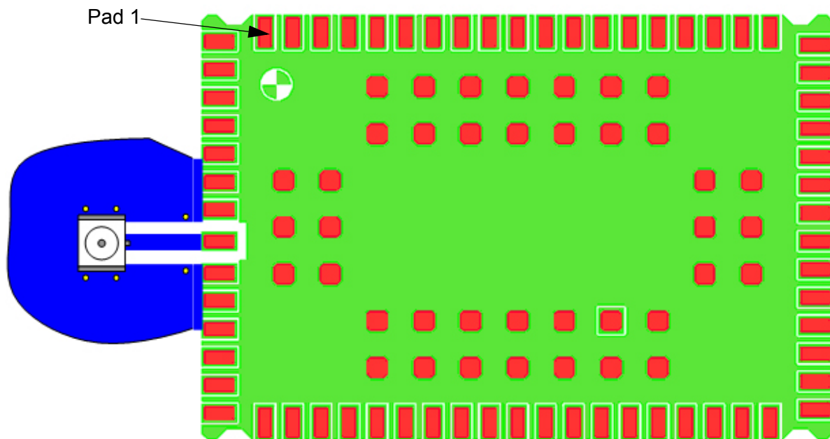
Figure 11: Routing to application's RF connector - top view
