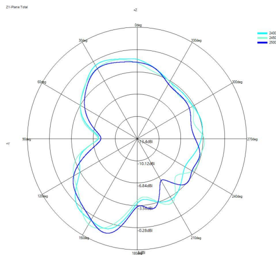
(2) Y-Z Plane(unit:dBi):
