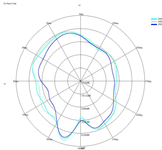
(1) X-Z Plane(unit:dBi):
