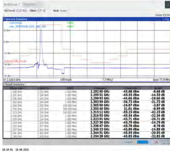
1-N30--30-10-L-1-DFT-PI2BPSK-Edge_1RB_Left-1@0-Ant1-PASS-see graph
