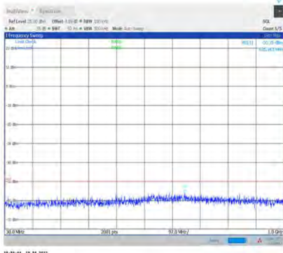
1-N30--15-10-H-1-DFT-PI2BPSK-Inner_1RB_Left- 1@1-30-1000-Ant1--55.75--50-PASS
