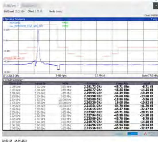
1-N30--30-10-L-4-CP-QPSK-Edge_1RB_Left-1@0-Ant1-PASS-see graph
