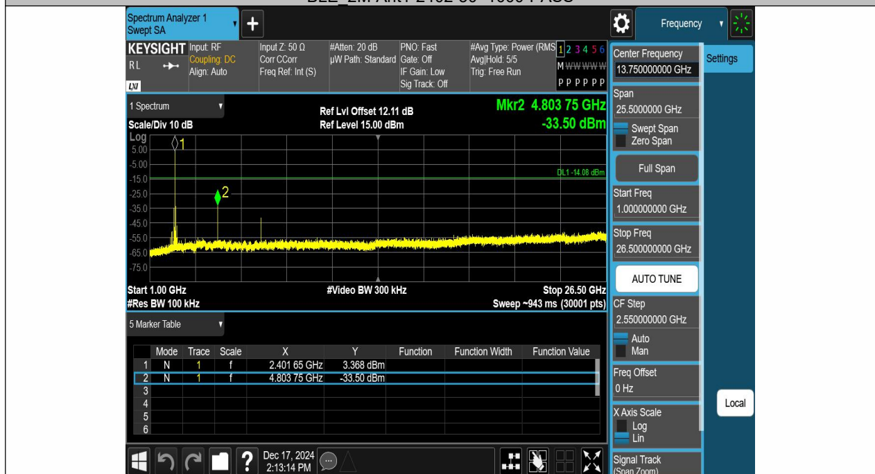
BLE_2M-Ant1-2402-1000~26500-PASS
