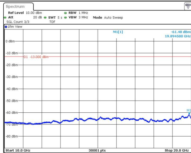
Band2-9262-3-10000~20000MHz
