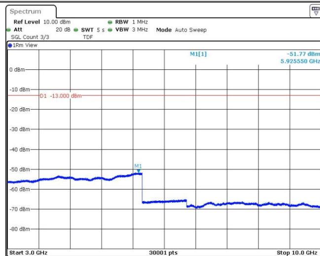
Band5-4233-4-3000~10000MHz
