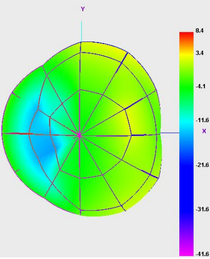
Bluetooth 78 TRP
