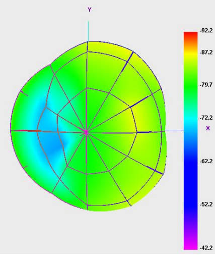
Bluetooth 78 TIS
