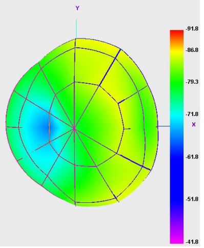
Bluetooth 39 TIS
