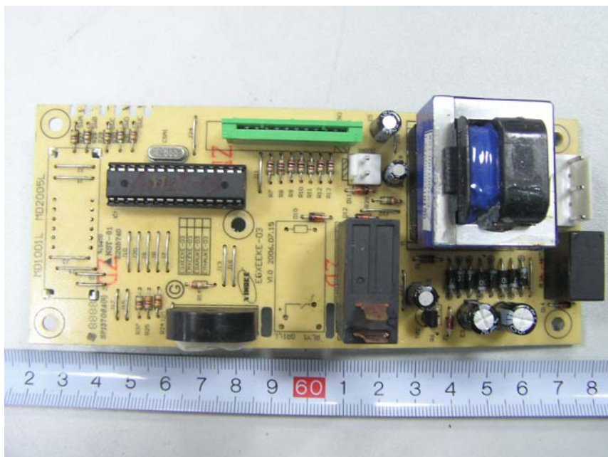
EUT – Main Board PCB Front View
