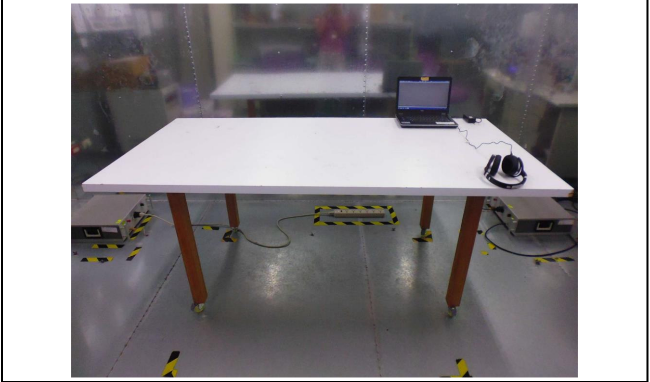
Conducted Emission Test (Model:SCBT6, Charging mode)
