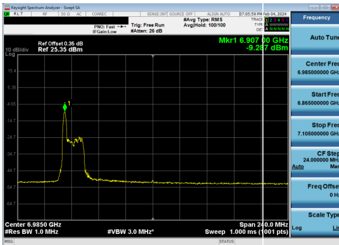
Plot 7-858. LPI Power Spectral Density Plot SDM Diversity Antenna WF7 (160MHz 802.11ax RU26 (UNII Band 8) – Ch. 207)
