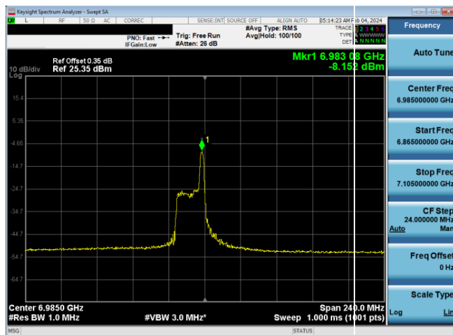
Plot 7-859. LPI Power Spectral Density Plot SDM Diversity Antenna WF8 (160MHz 802.11ax RU26 (UNII Band 8) – Ch. 207)
