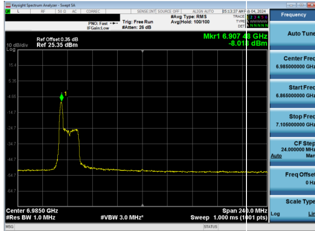
Plot 7-857. LPI Power Spectral Density Plot SDM Diversity Antenna WF8 (160MHz 802.11ax RU26 (UNII Band 8) – Ch. 207)
