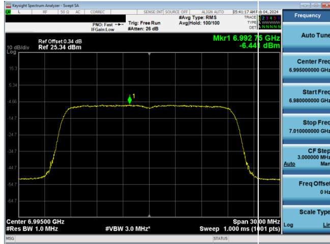
Plot 7-839. LPI Power Spectral Density Plot SDM Diversity Antenna WF8 (20MHz 802.11ax RU242 (UNII Band 8) - Ch. 209)
