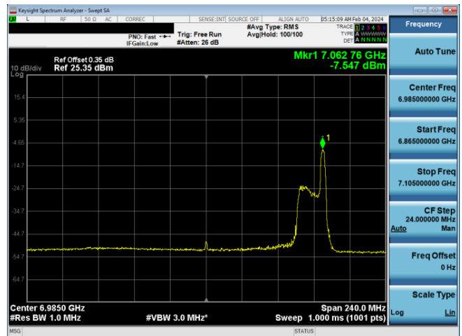
Plot 7-861. LPI Power Spectral Density Plot SDM Diversity Antenna WF8 (160MHz 802.11ax RU26 (UNII Band 8) – Ch. 207)
