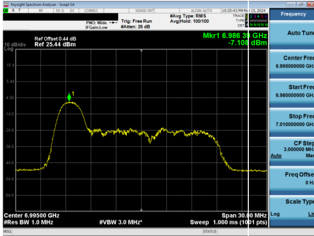
Plot 7-833. LPI Power Spectral Density Plot SDM Diversity Antenna WF8 (20MHz 802.11ax RU26 (UNII Band 8) – Ch. 209)
