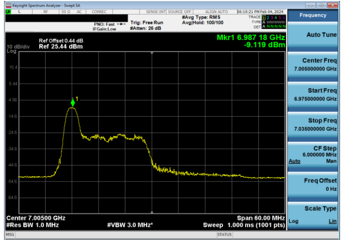
Plot 7-842. LPI Power Spectral Density Plot SDM Diversity Antenna WF7 (40MHz 802.11ax RU26 (UNII Band 8) - Ch. 211)
