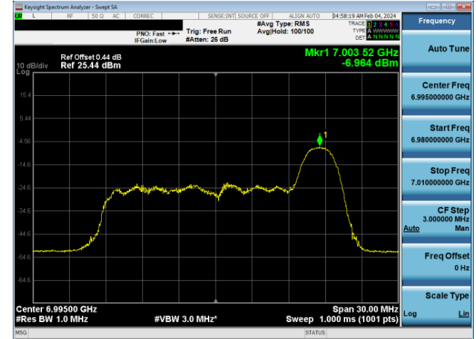
Plot 7-837. LPI Power Spectral Density Plot SDM Diversity Antenna WF8 (20MHz 802.11ax RU26 (UNII Band 8) – Ch. 209)
