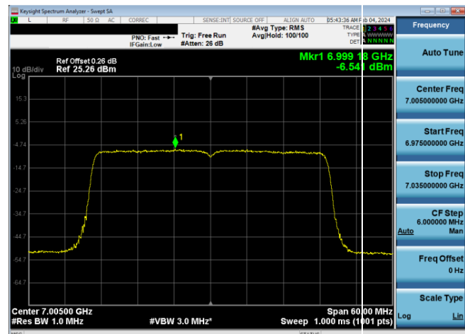
Plot 7-847. LPI Power Spectral Density Plot SDM Diversity Antenna WF8 (40MHz 802.11ax RU484 (UNII Band 8) – Ch. 211)
