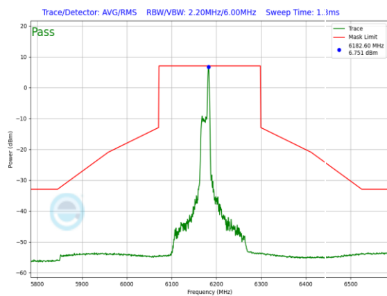
Plot 7-878. SP In-Band Emission Plot Antenna WF5B (160MHz 802.11ax RU26 (UNII Band 5) – Ch. 47)
