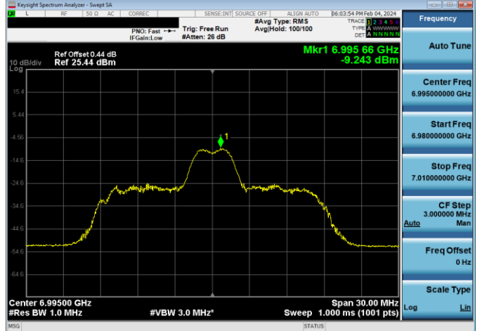
Plot 7-836. LPI Power Spectral Density Plot SDM Diversity Antenna WF7 (20MHz 802.11ax RU26 (UNII Band 8) – Ch. 209)
