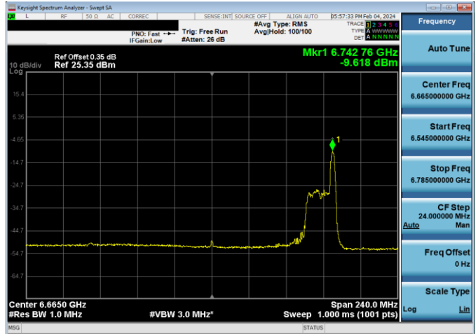
Plot 7-830. LPI Power Spectral Density Plot SDM Diversity Antenna WF7 (160MHz 802.11ax RU26 (UNII Band 7) – Ch. 143)
