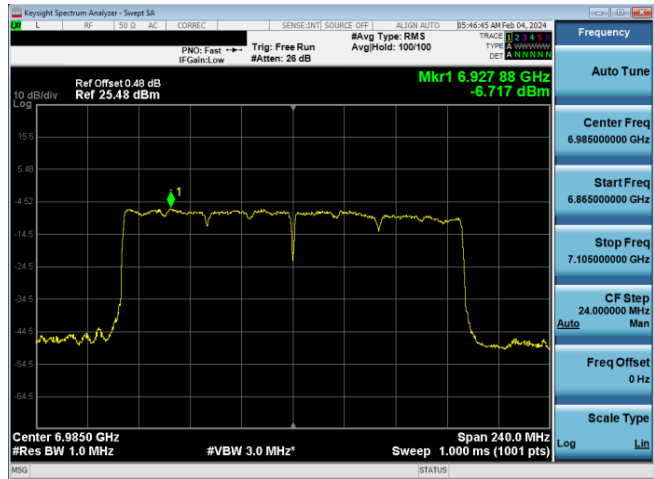
Plot 7-863. LPI Power Spectral Density Plot SDM Diversity Antenna WF8 (160MHz 802.11ax RU996x2 (UNII Band 8) – Ch. 207)
