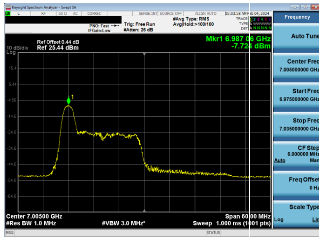
Plot 7-841. LPI Power Spectral Density Plot SDM Diversity Antenna WF8 (40MHz 802.11ax RU26 (UNII Band 8) - Ch. 211)
