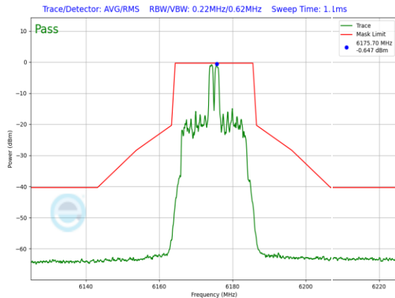
Plot 7-898. SP In-Band Emission Plot Antenna WF8 (20MHz 802.11ax RU26 (UNII Band 5) – Ch. 45)
