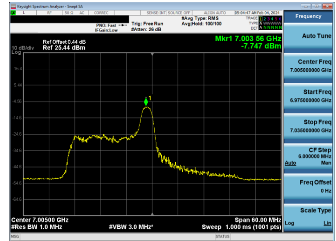
Plot 7-843. LPI Power Spectral Density Plot SDM Diversity Antenna WF8 (40MHz 802.11ax RU26 (UNII Band 8) - Ch. 211)
