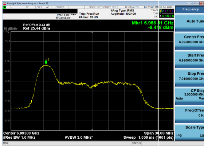
Plot 7-834. LPI Power Spectral Density Plot SDM Diversity Antenna WF7 (20MHz 802.11ax RU26 (UNII Band 8) – Ch. 209)
