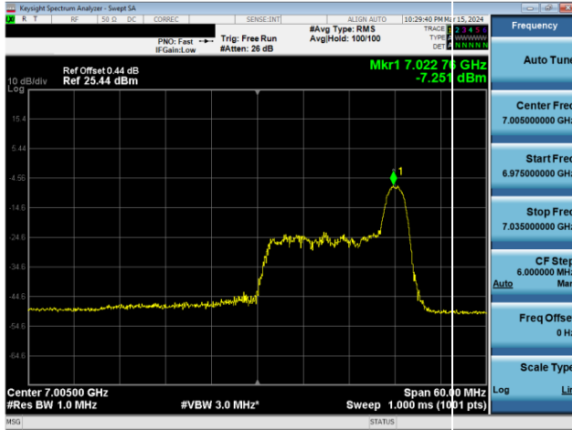
Plot 7-845. LPI Power Spectral Density Plot SDM Diversity Antenna WF8 (40MHz 802.11ax RU26 (UNII Band 8) – Ch. 211)
