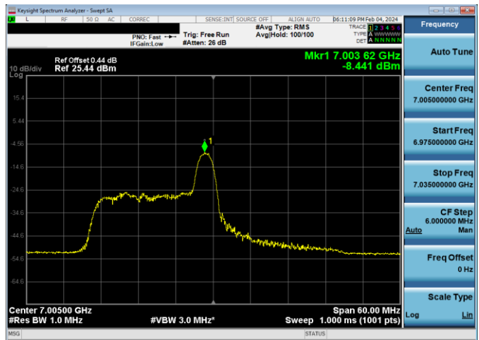
Plot 7-844. LPI Power Spectral Density Plot SDM Diversity Antenna WF7 (40MHz 802.11ax RU26 (UNII Band 8) - Ch. 211)
