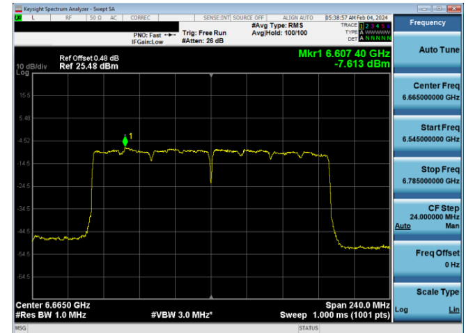
Plot 7-831. LPI Power Spectral Density Plot SDM Diversity Antenna WF8 (160MHz 802.11ax RU996x2 (UNII Band 7) – Ch. 143)
