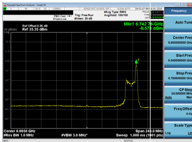
Plot 7-829. LPI Power Spectral Density Plot SDM Diversity Antenna WF8 (160MHz 802.11ax RU26 (UNII Band 7) – Ch. 143)
