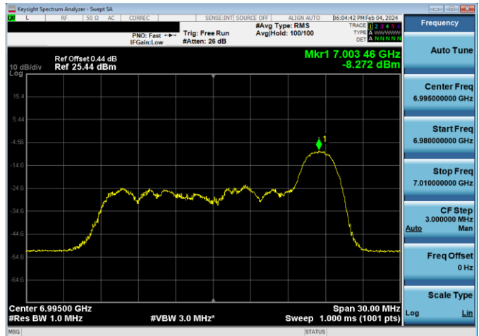
Plot 7-838. LPI Power Spectral Density Plot SDM Diversity Antenna WF7 (20MHz 802.11ax RU26 (UNII Band 8) – Ch. 209)
