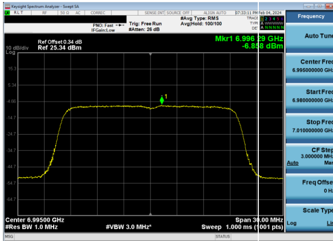
Plot 7-840. LPI Power Spectral Density Plot SDM Diversity Antenna WF7 (20MHz 802.11ax RU242 (UNII Band 8) - Ch. 209)
