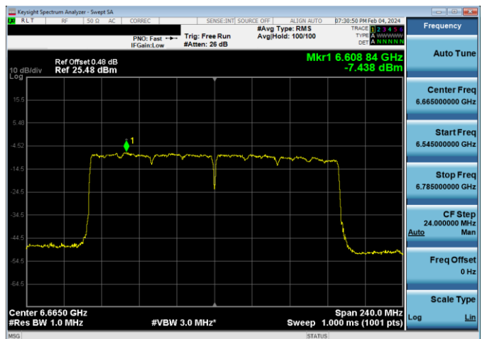
Plot 7-832. LPI Power Spectral Density Plot SDM Diversity Antenna WF7 (160MHz 802.11ax RU996x2 (UNII Band 7) – Ch. 143)
