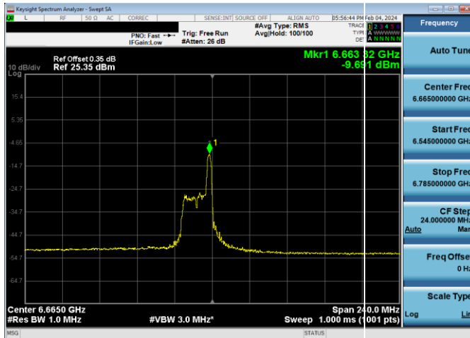
Plot 7-828. LPI Power Spectral Density Plot SDM Diversity Antenna WF7 (160MHz 802.11ax RU26 (UNII Band 7) – Ch. 143)
