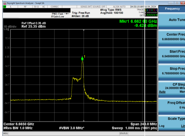
Plot 7-827. LPI Power Spectral Density Plot SDM Diversity Antenna WF8 (160MHz 802.11ax RU26 (UNII Band 7) – Ch. 143)
